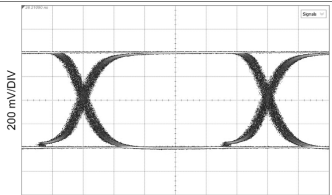
CD Mode, measured at SDI_IO+ HOST_EQ0 = F, SDI_OUT_SEL = H, OUT_CTRL = F Figure 33. 270 Mbps, TL = 20" FR4, Reclocked
