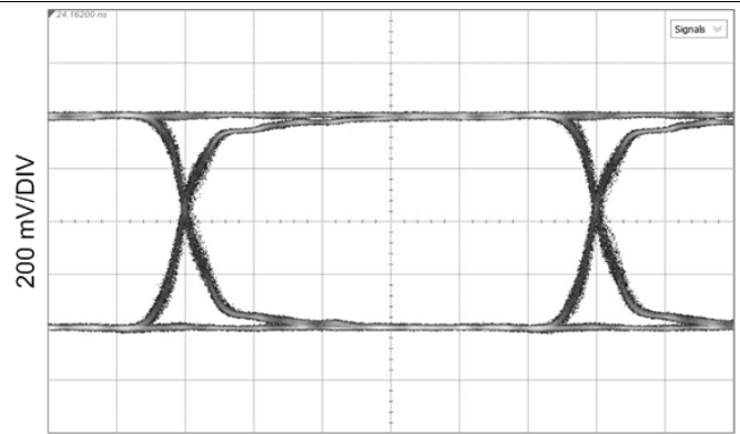
CD Mode, measured at SDI_IO+ HOST_EQ0 = F, SDI_OUT_SEL = H, OUT_CTRL = F Figure 31. 1.485 Gbps, TL = 20" FR4, Reclocked
