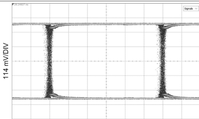
EQ Mode, measured at OUT0± HOST_EQ0 = F, SDI_OUT_SEL = H, OUT_CTRL = F Figure 32. 270 Mbps, CC = 600-m Belden 1694A, Reclocked
