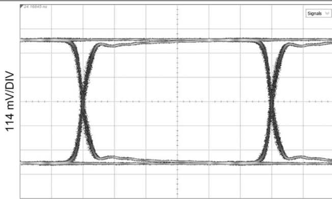
EQ Mode, measured at OUT0± HOST_EQ0 = F, SDI_OUT_SEL = H, OUT_CTRL = F Figure 30. 1.485 Gbps, CC = 300-m Belden 1694A, Reclocked
