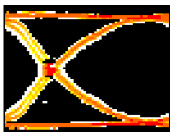
Figure 11. Internal Eye Monitor Hit Density Plot
