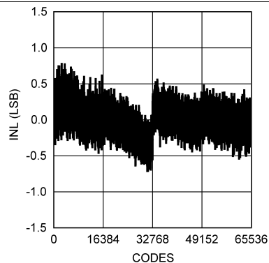
Figure 8. INL - 250 kSPS
