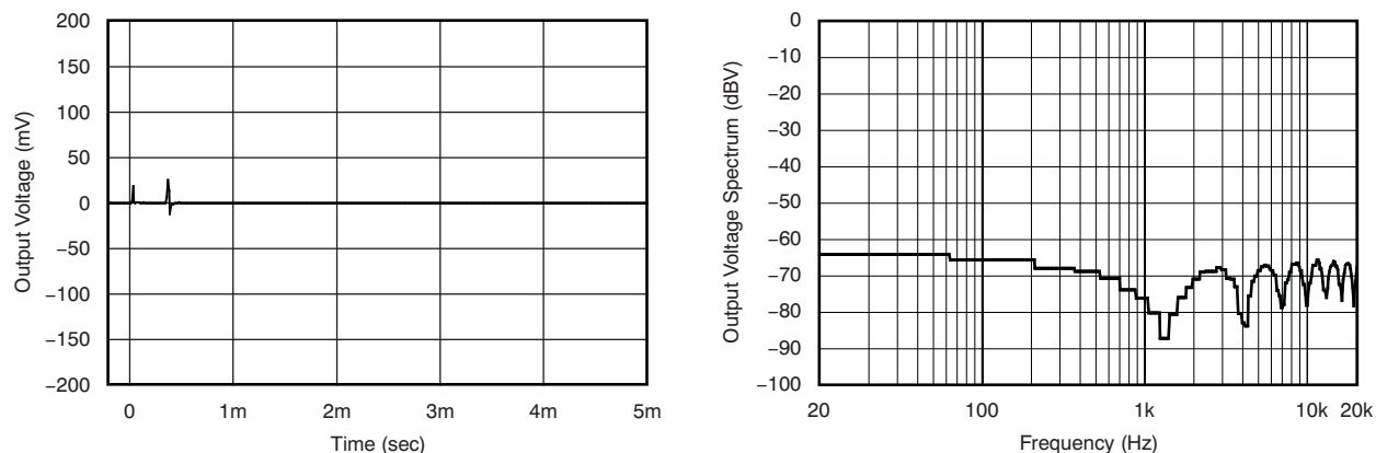
Figure 14. Pop/Click (Enable)
