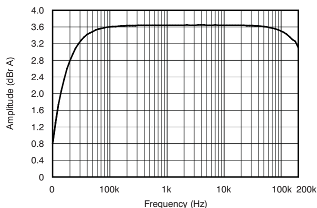
Figure 12. Frequency Response
