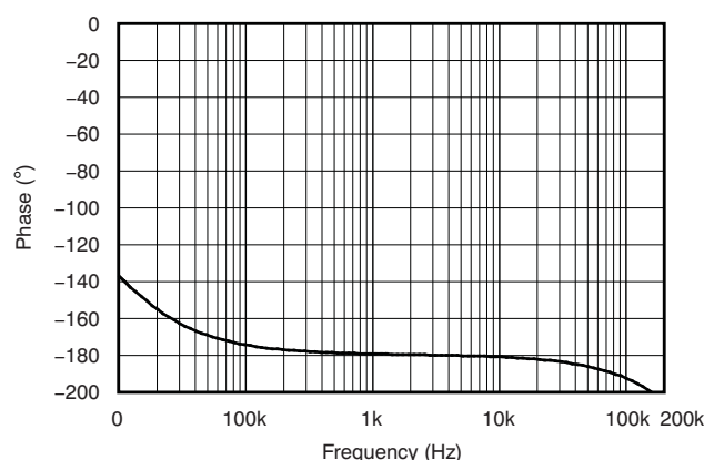
Figure 13. Phase Response
