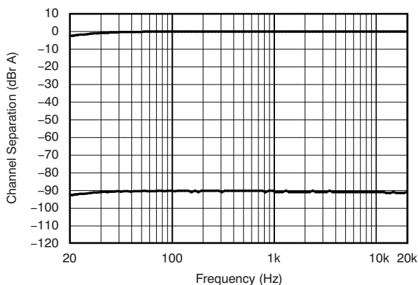
Figure 11. Channel Separation
