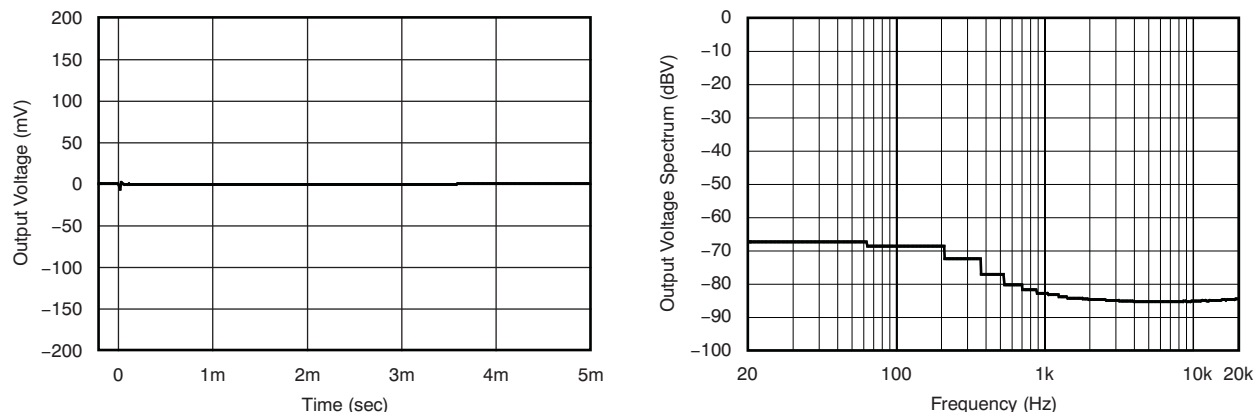
Figure 15. Pop/Click (Disable)
