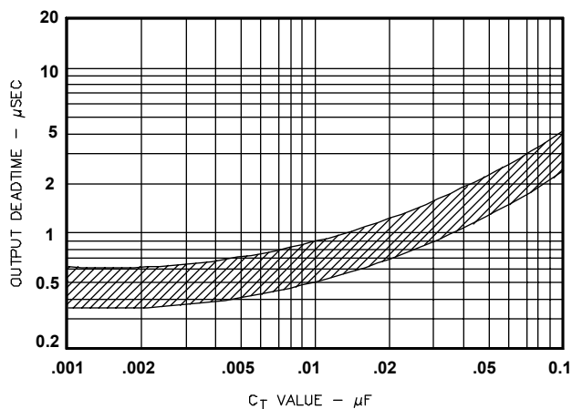
Figure 2 · Output Stage Deadtime vs. C_T
