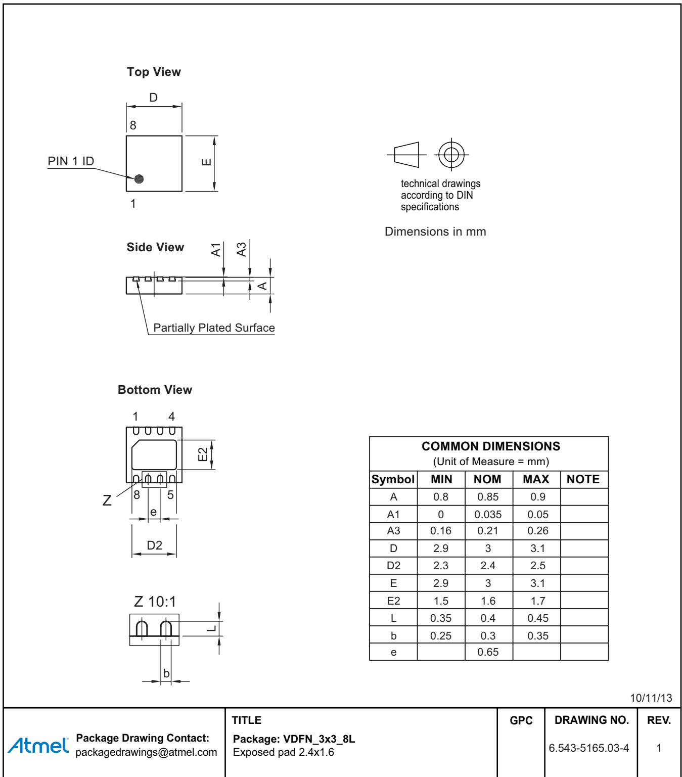
Figure 11-1. DFN8
