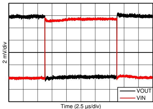
Figure 25. Negative Overload Recovery
