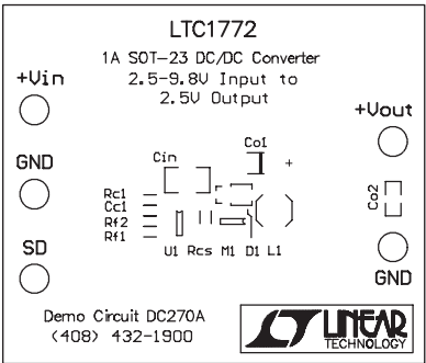
Component Side Silkscreen
