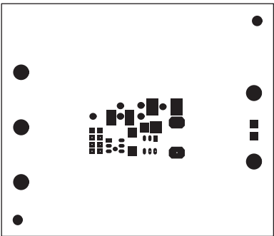
Component Side Solder Mask
