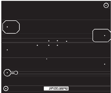
Solder Side
