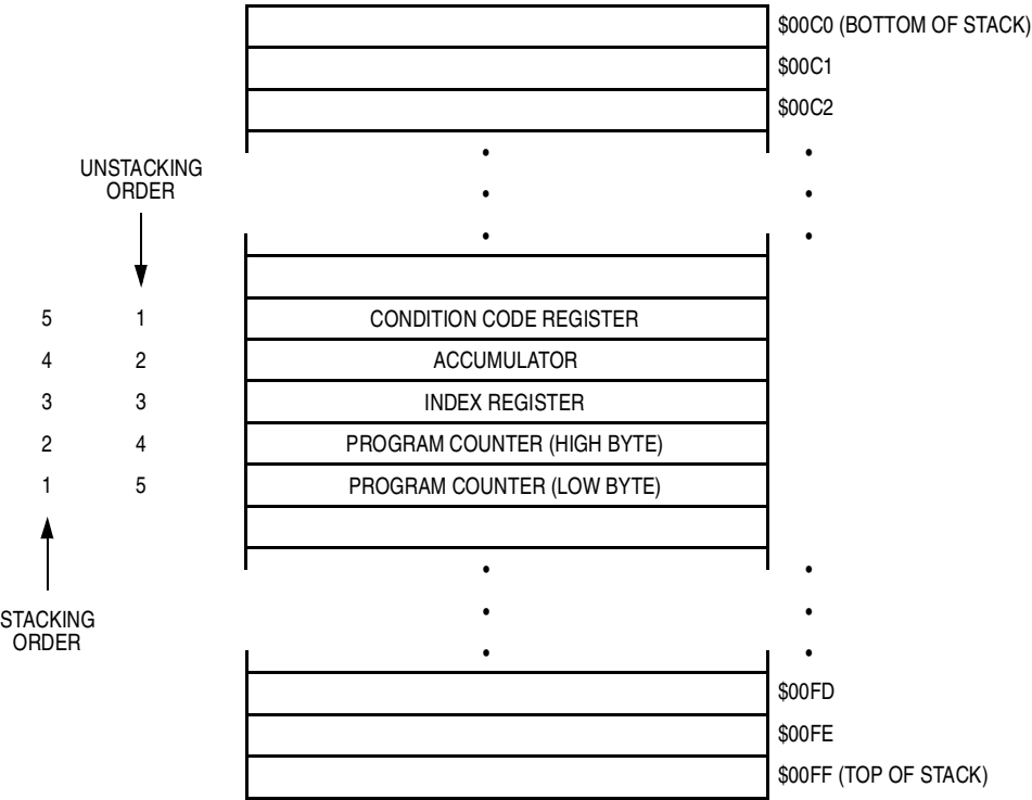
Figure 4-6. Interrupt Stacking Order
