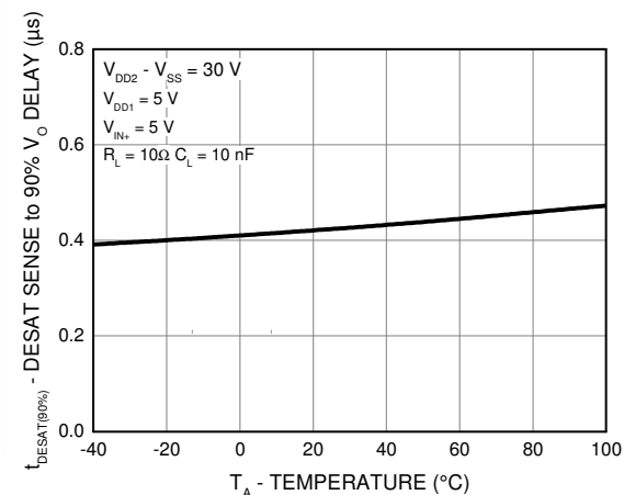
Figure 23. DESAT Sense to 90% V_O Delay ( t_{DESAT(90\%)} ) vs. Temperature
