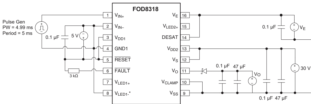
Figure 37. Low Level Output Current ( I_{OL} ) Test Circuit
