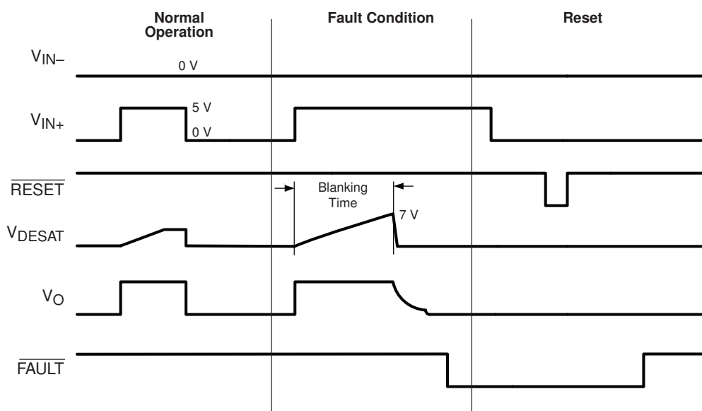
Figure 58. Timing Relationship Among DESAT, \overline{\text{FAULT}} , and \overline{\text{RESET}}
