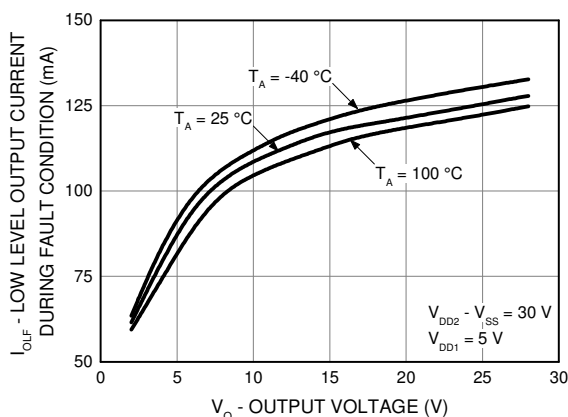
Figure 4. Low Level Output Current During Fault Condition ( I_{\text{OLF}} ) vs. Output Voltage ( V_O )
