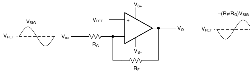
Figure 63. Inverting Amplifier
