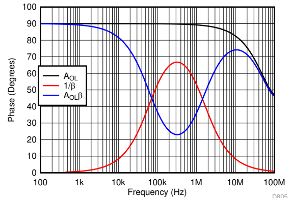
Figure 75. Loop-Gain Phase vs Frequency for the Transimpedance Amplifier Circuit of Figure 73
