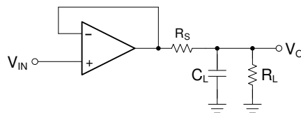
Figure 60. OPA810 Driving Capacitive Load
