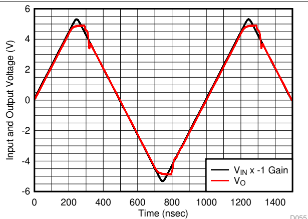
Figure 14. Output Overdrive Recovery
