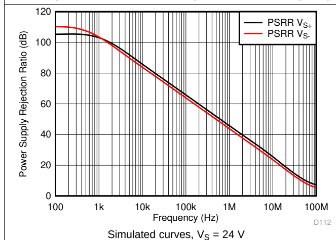
Figure 52. Power Supply Rejection Ratio vs Frequency
