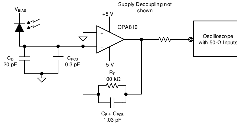
Figure 73. Wideband, High-Sensitivity, Transimpedance Amplifier
