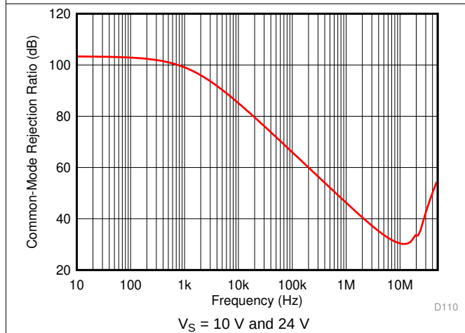
Figure 50. Common-Mode Rejection Ratio vs Frequency
