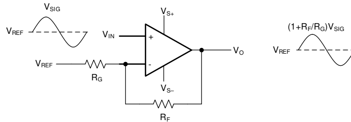
Figure 62. Noninverting Amplifier
