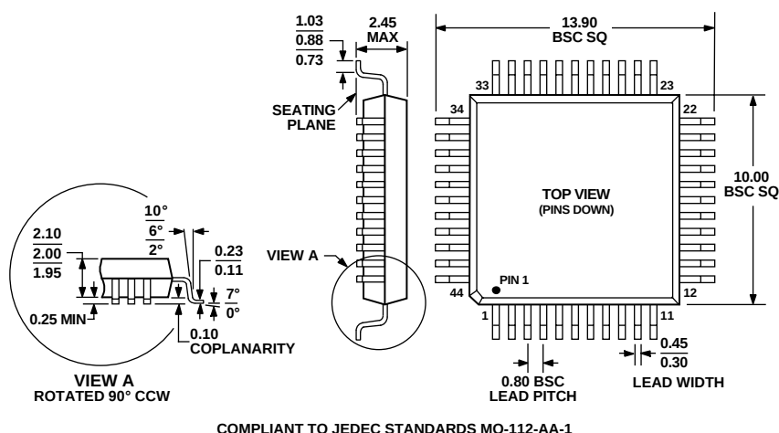
Figure 67. Metric Quad Flat Package [MQFP] (S-44-2) Dimensions shown in millimeters
