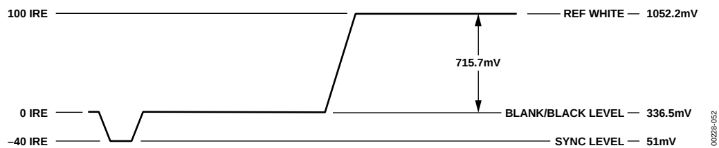
Figure 52. NTSC RGB Video Levels
