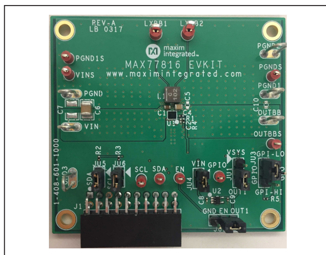
Figure 1. MAX77816 EV Kit Photo
