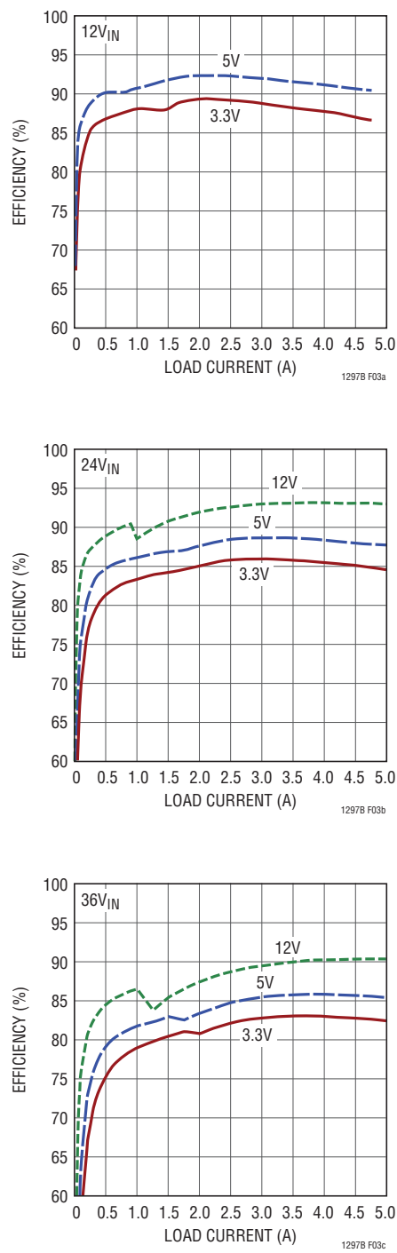
Figure 3. Measured DC1297B Efficiency at 12V_{IN} , 24V_{IN} , 36V_{IN} (DCM mode enabled)
