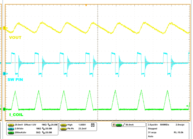
Figure 13. Output ripple, V_{IN}=3.6\text{ V} , V_{OUT} = 1.8\text{ V} , I_{OUT} = 50\text{ mA}
