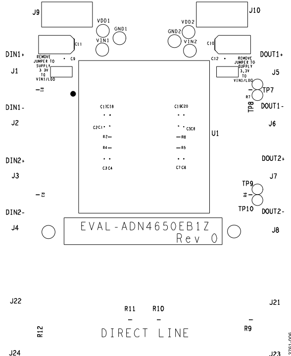
Figure 7. EVAL-ADN4650EB1Z Silkscreen
