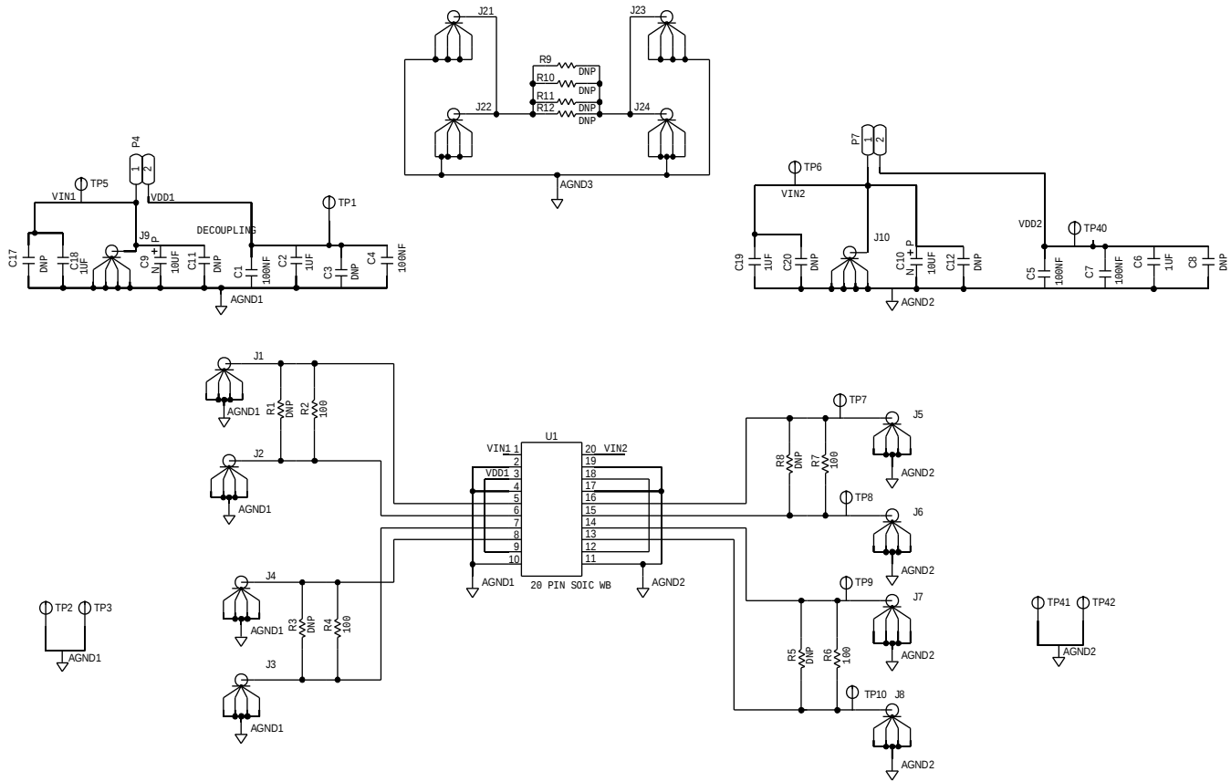
Figure 6. EVAL-ADN4650EB1Z Schematic
