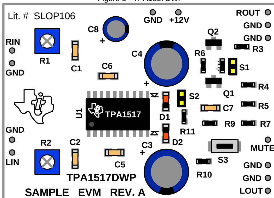
Figure 1 - TPA1517DWP
