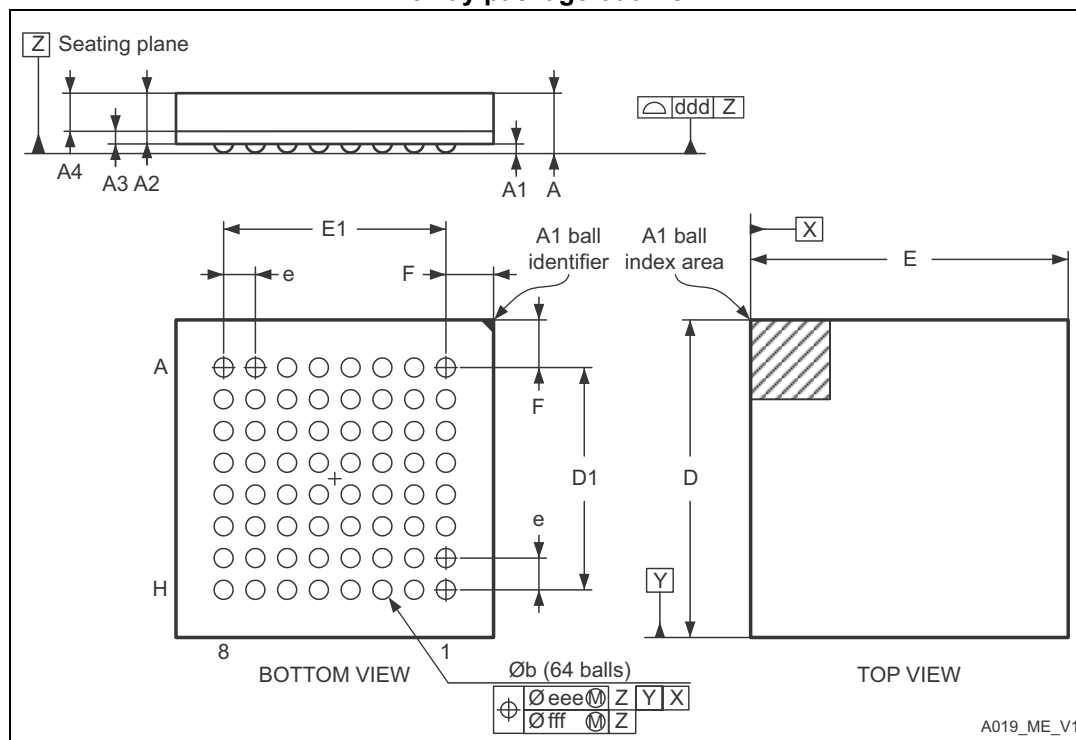
Figure 38. UFBGA – 64 balls, 5 x 5 mm, 0.5 mm pitch ultra profile fine pitch ball grid array package outline
