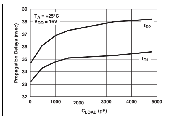
FIGURE 2-12: Propagation Delays vs. Capacitive Load.
