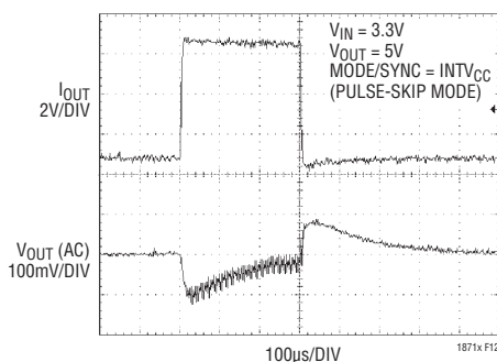
Figure 12. Load Transient Response for a 3.3V Input, 5V Output Boost Converter Application, 0.7A to 7A Step
