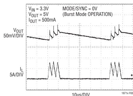
Figure 3. LTC1871X Burst Mode Operation (MODE/SYNC = 0V) at Low Output Current
