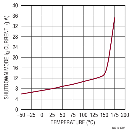
Shutdown Mode I_Q vs Temperature
