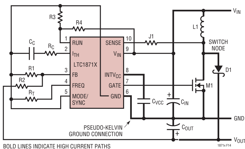
Figure 14. LTC1871X Boost Converter Layout Diagram
