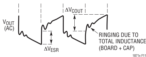
11e. Output Voltage Ripple Waveform
