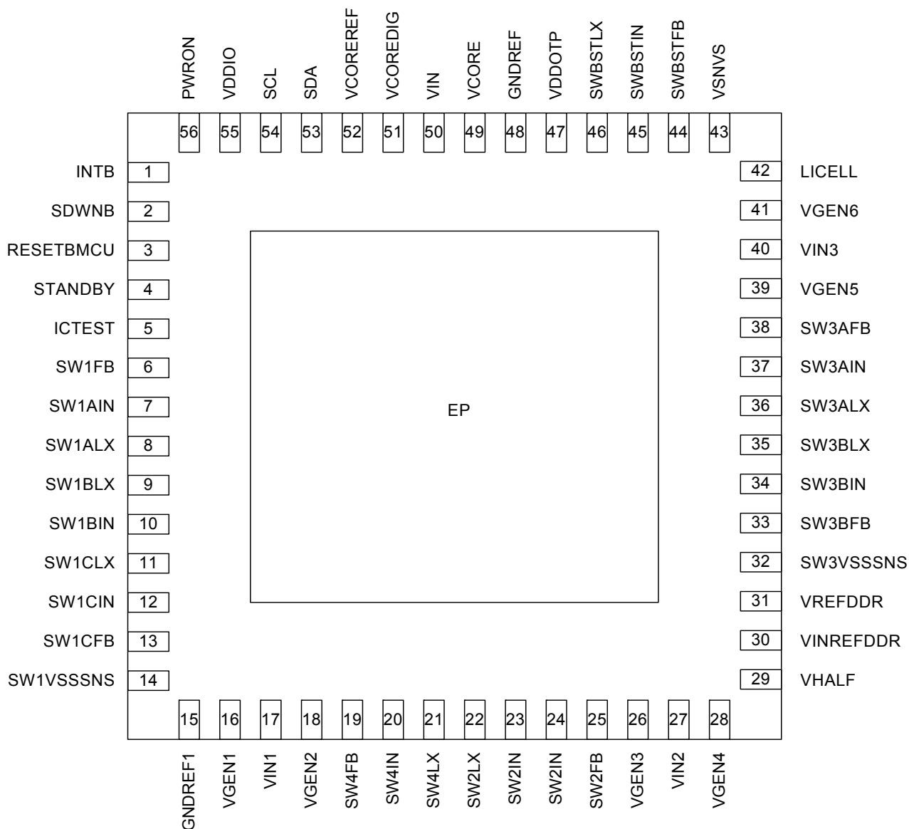
Figure 3. Pinout diagram
