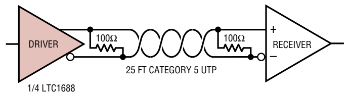
Figure 12. 100Mbps Differential Data Connection
