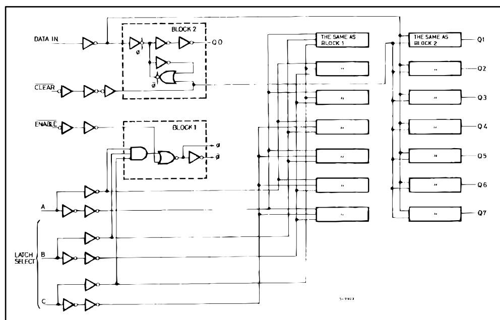
Figure 3: Logic diagram
