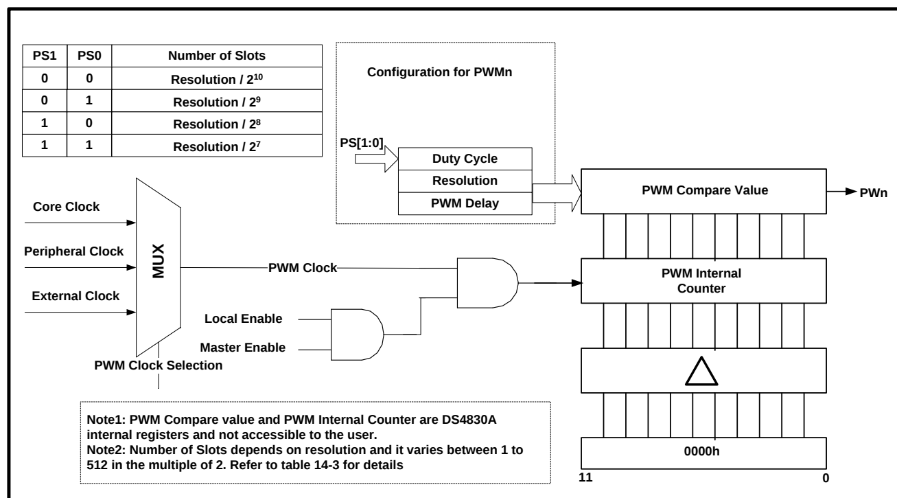
Figure 14-3: Block Diagram of One PWM Channel
