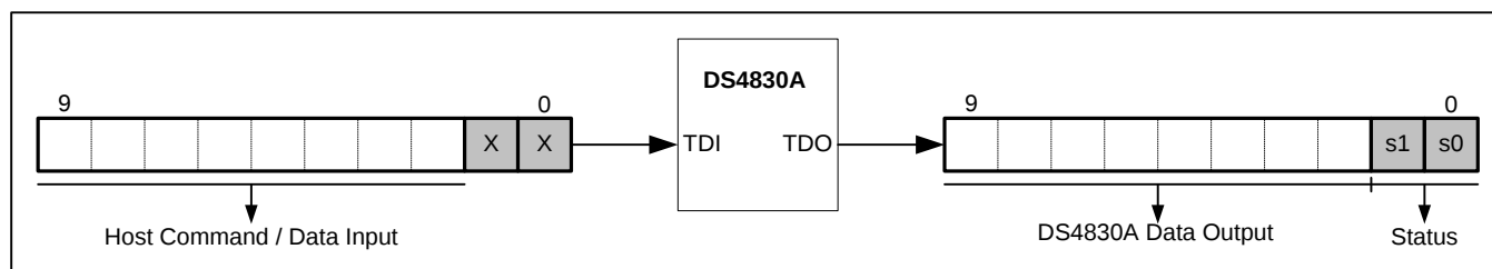
Figure 21-2: 10-Bit Word Format
