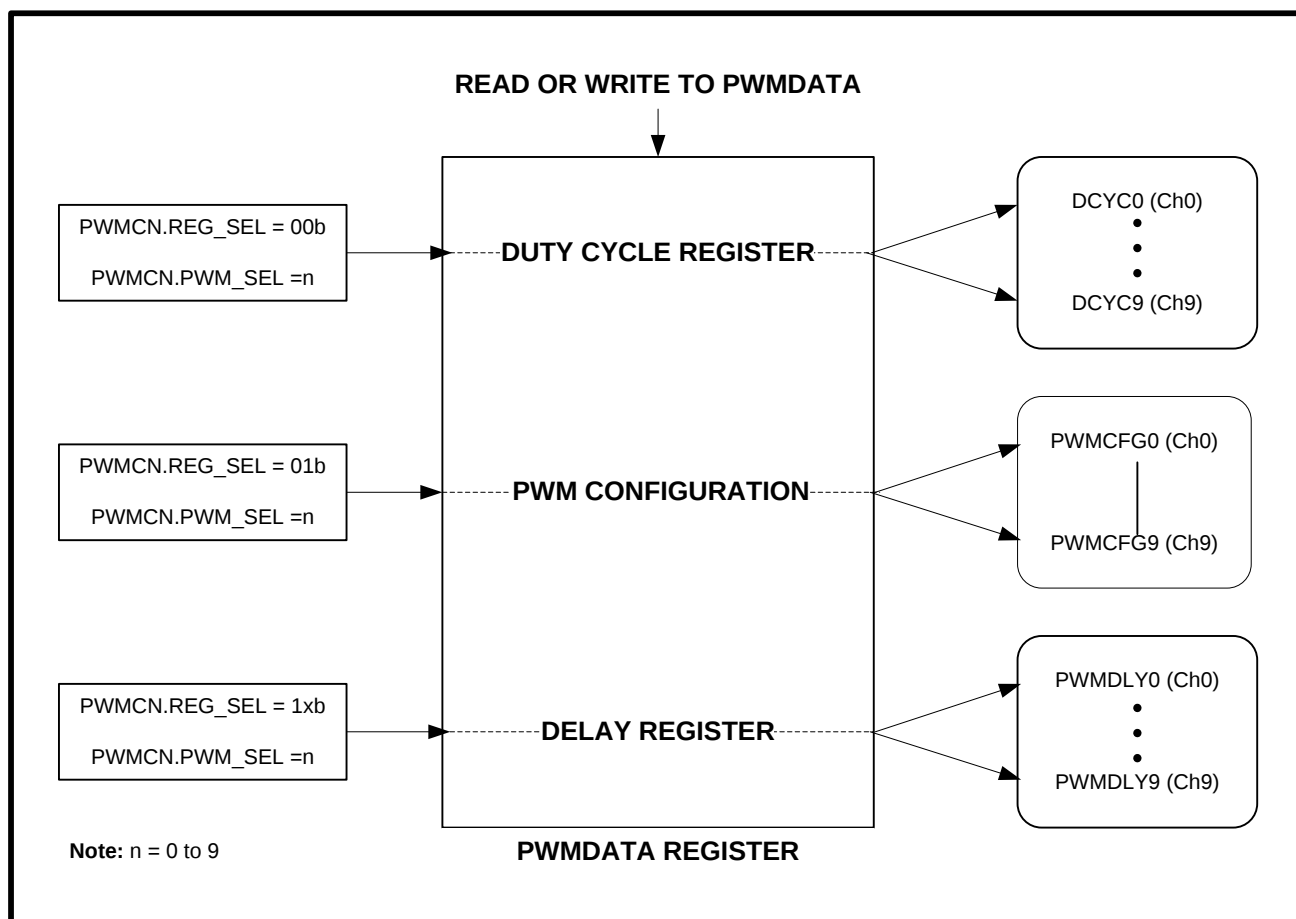
Figure 14-1: Illustration of PWMDATA and PWMCFG SFRs
