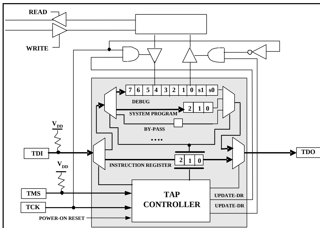
Figure 20-1: TAP and TAP Controller
