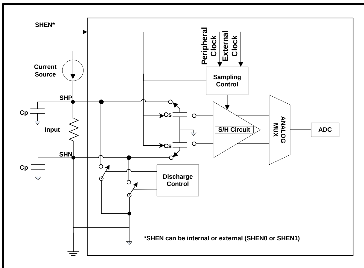
Figure 8-1: Sample and Hold Functional Block Diagram
