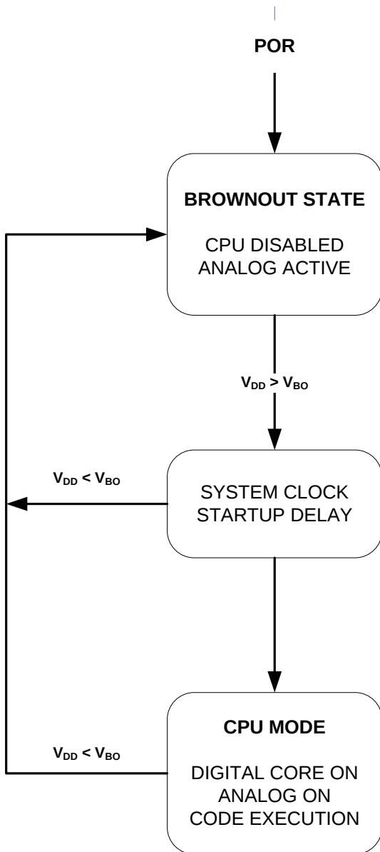
Figure 2-6: DS4830A State Diagram
