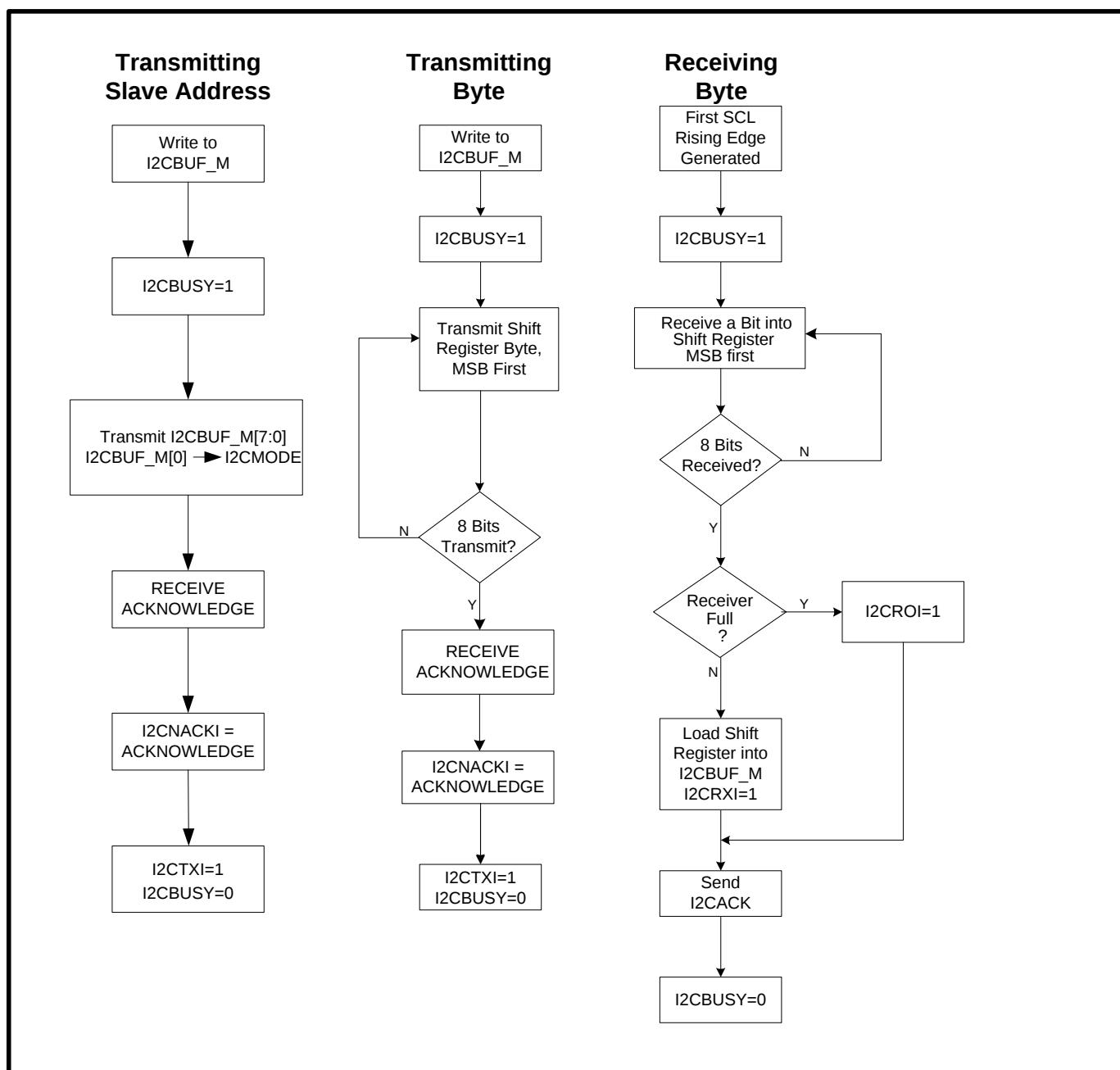
Figure 10-5: Master I 2 C Data Flow
