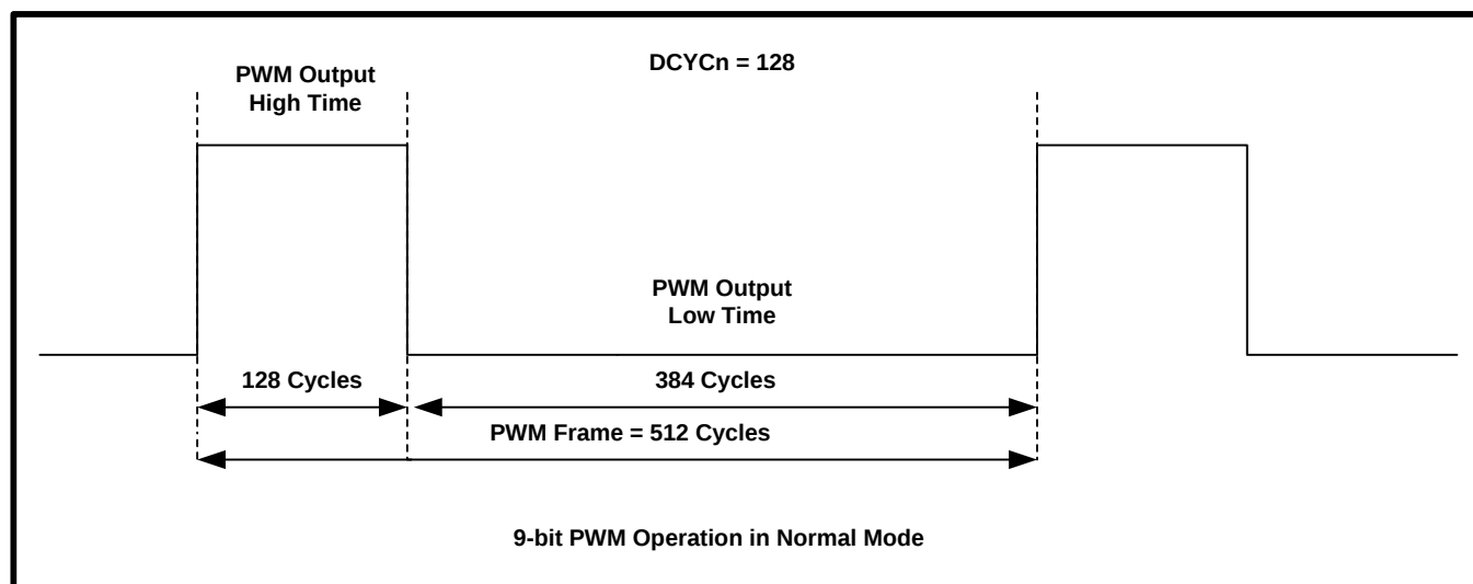
Figure 14-4: PWM Duty Cycle Set to 128 with 9-Bit Resolution
