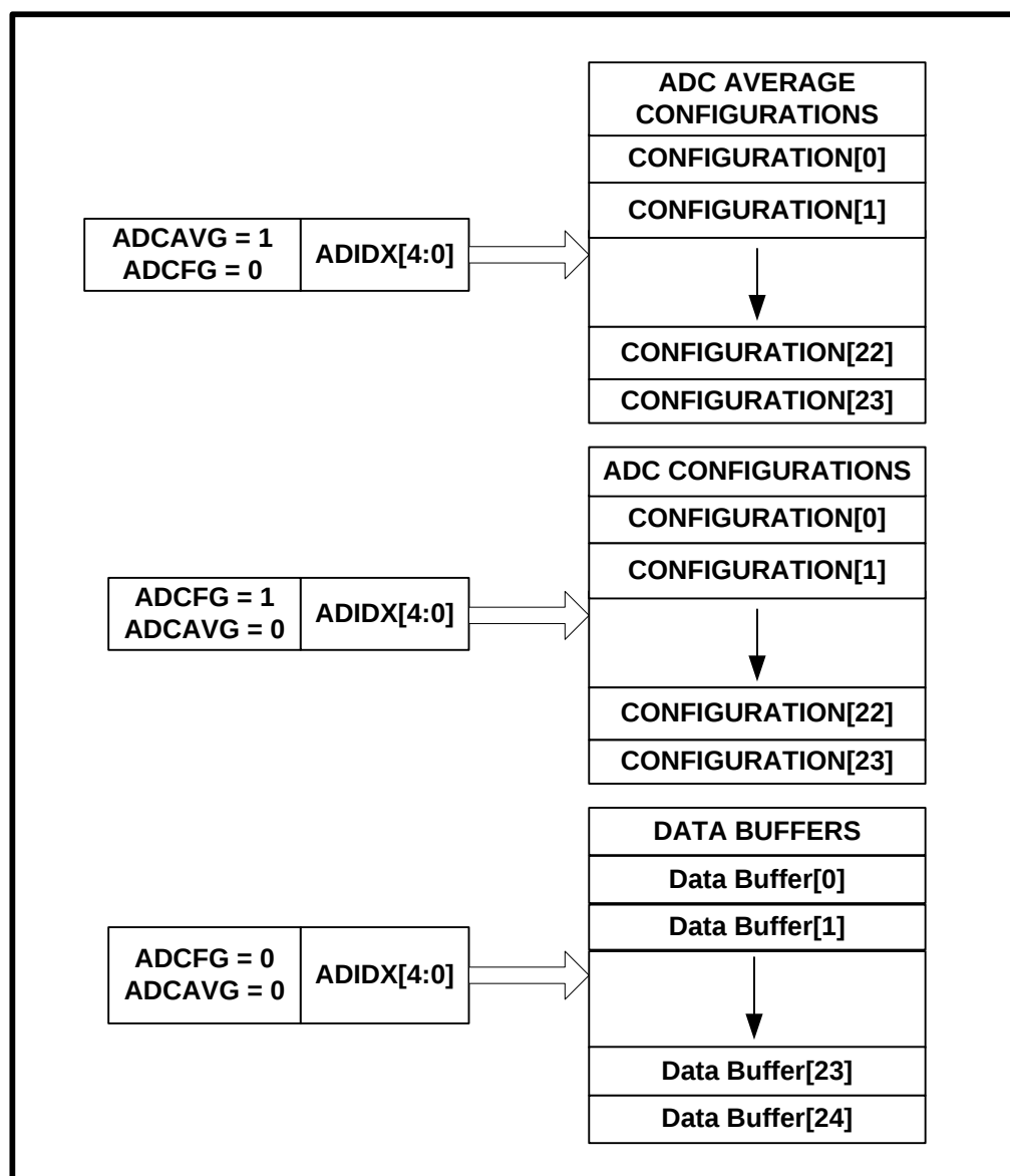
Figure 7-2: ADC Configurations and Data Buffers
