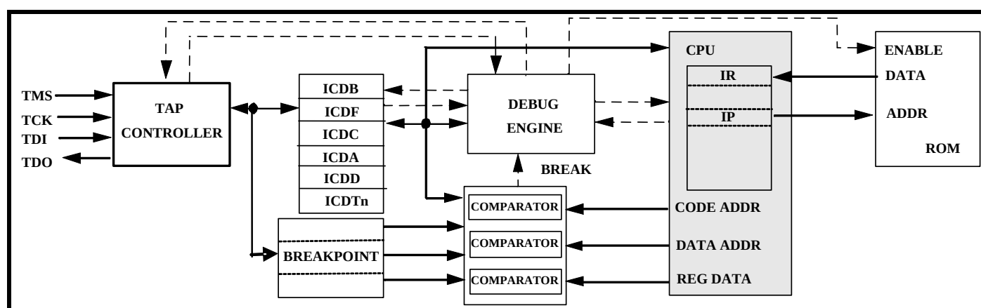
Figure 21-1: In-Circuit Debugger
