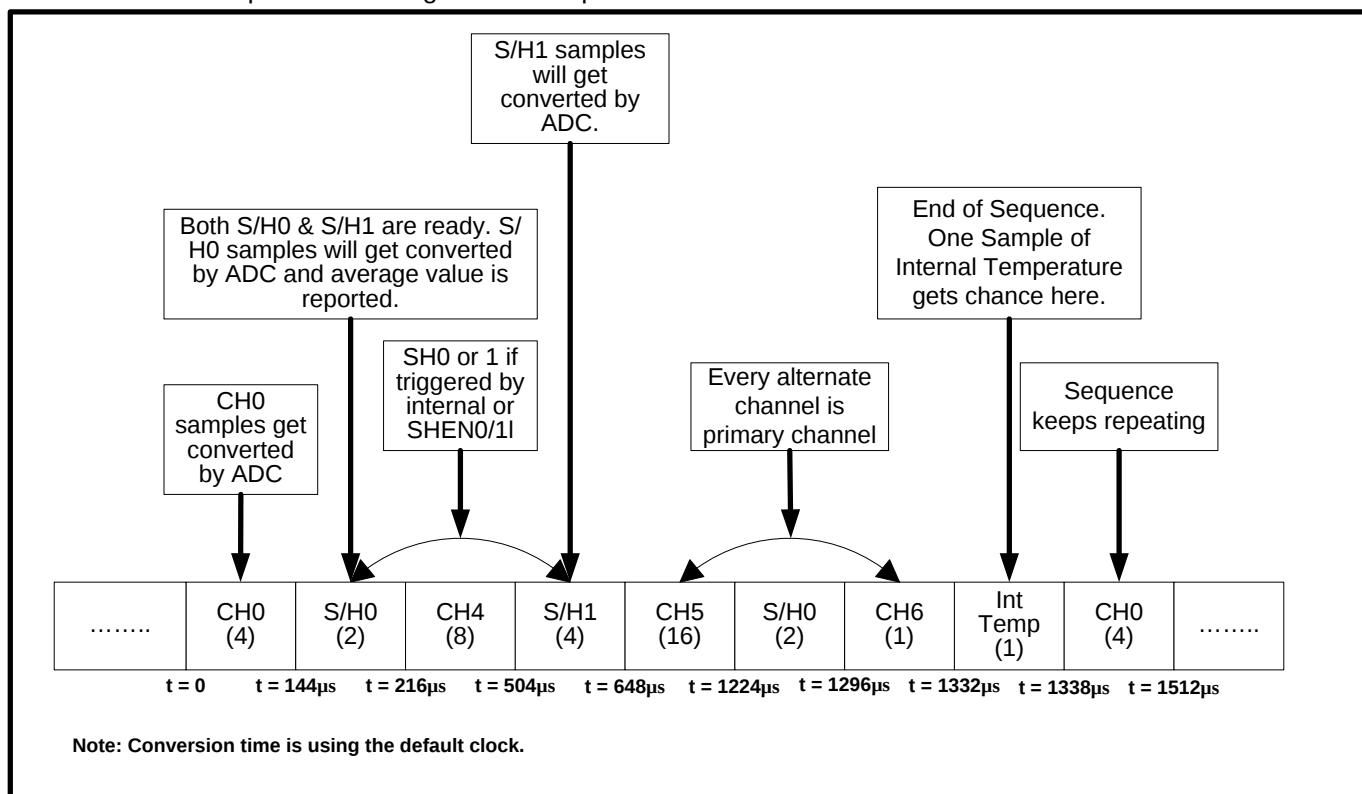
Figure 7-5: ADC Frame Sequence with Averaging
