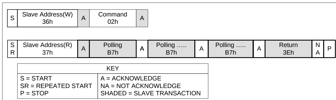
Figure 22-2: I 2 C Bootloader Polling
