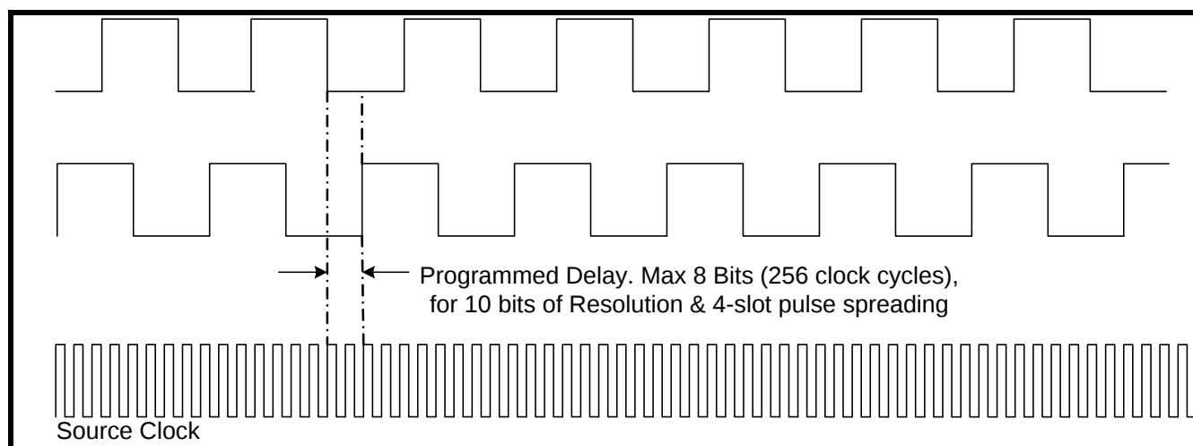
Figure 14-6: PWM Delay Operation without Pulse Spreading
