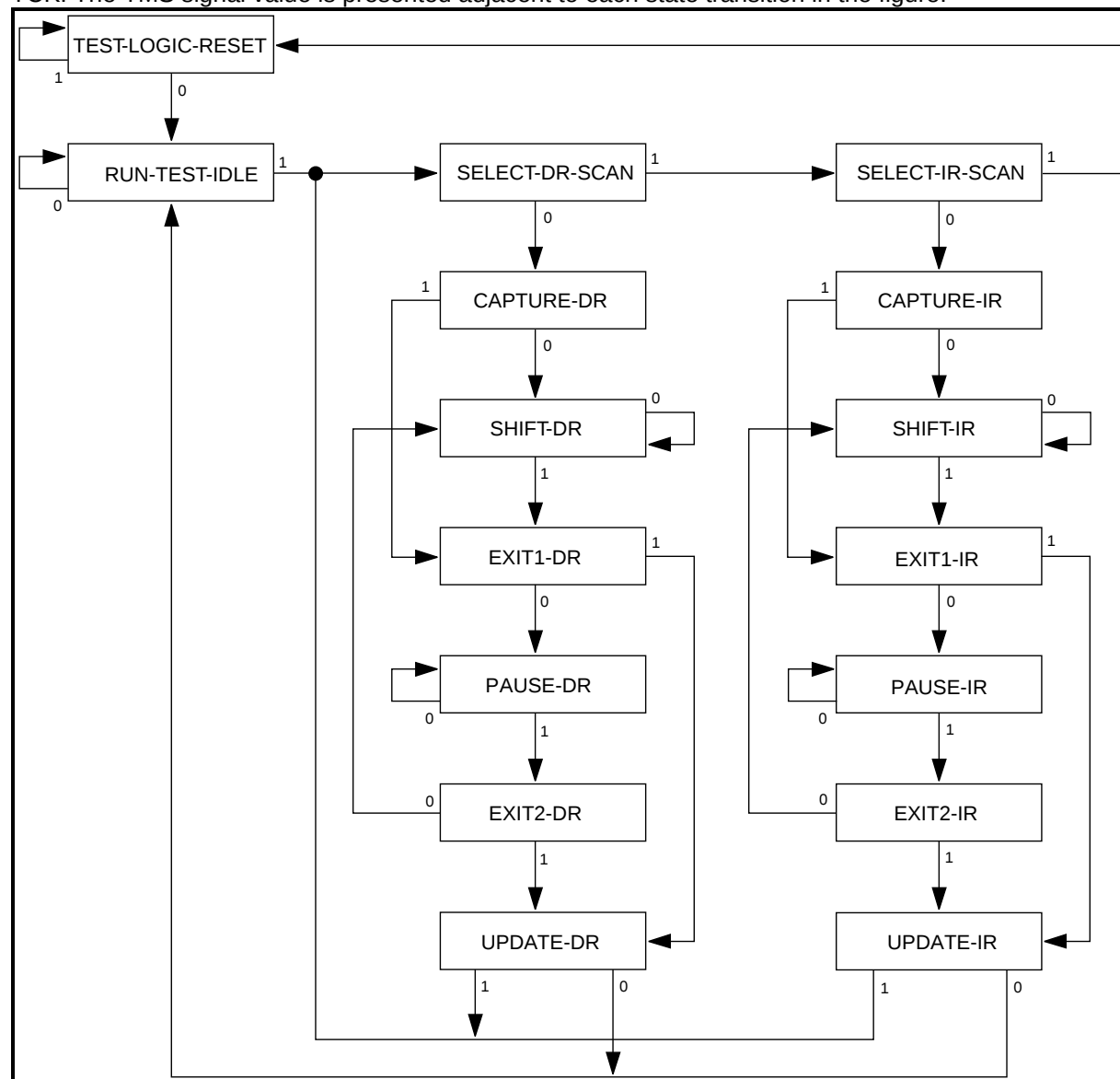
Figure 20-2: TAP Controller State Diagram
