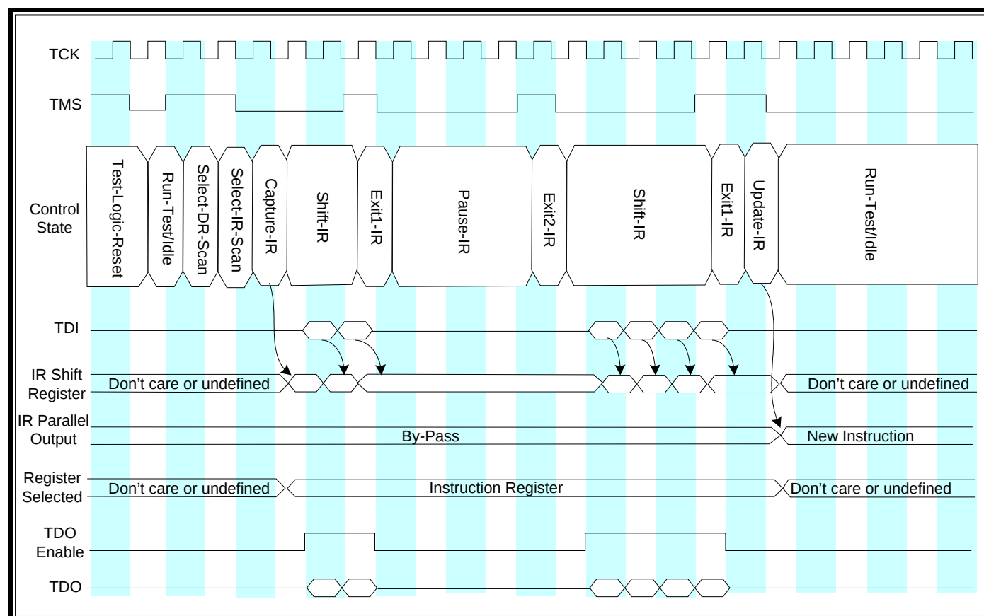
Figure 20-3: TAP Controller Debug Mode IR-Scan Example
