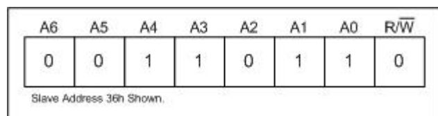
Figure 10-4: Slave Address Format
