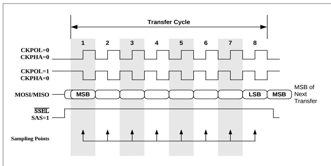
Figure 12-3: SPI Transfer Formats (CKPHA=0)
