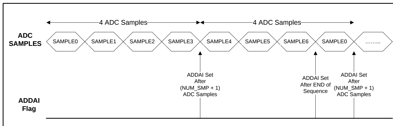
Figure 7-6: ADC Interrupt Intervals with NUM\_SMP
