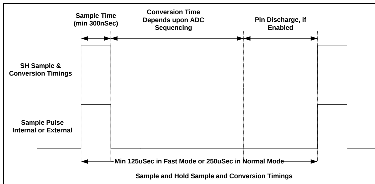
Figure 8-2: Sample and Hold Conversion Timings without Averaging
