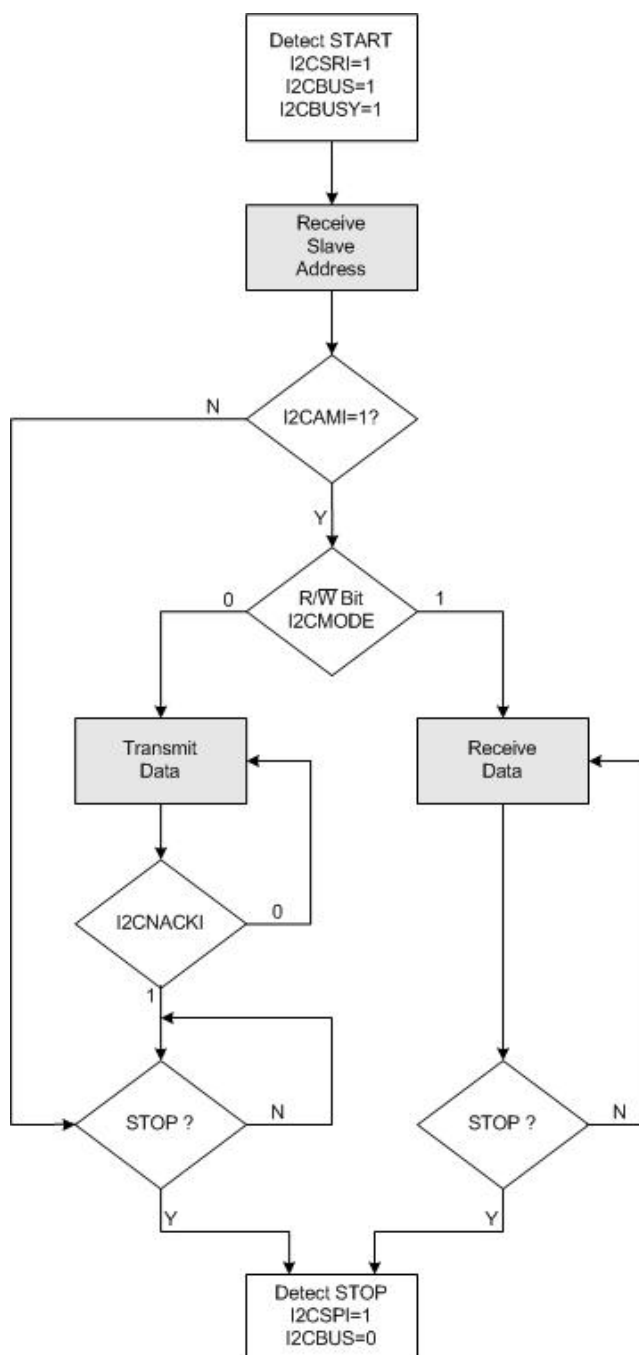
Figure 11-1: Slave I 2 C Flow
