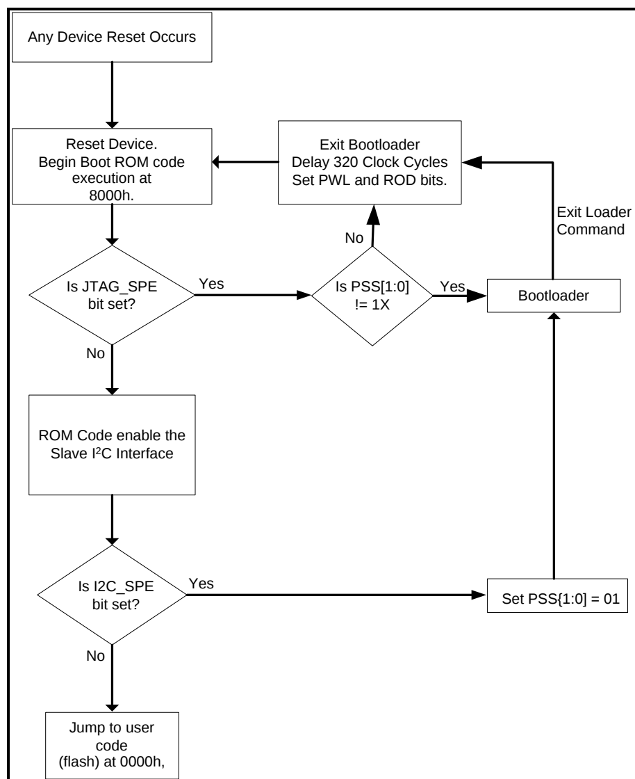
Figure 22-1: Entering Bootloader Operation
