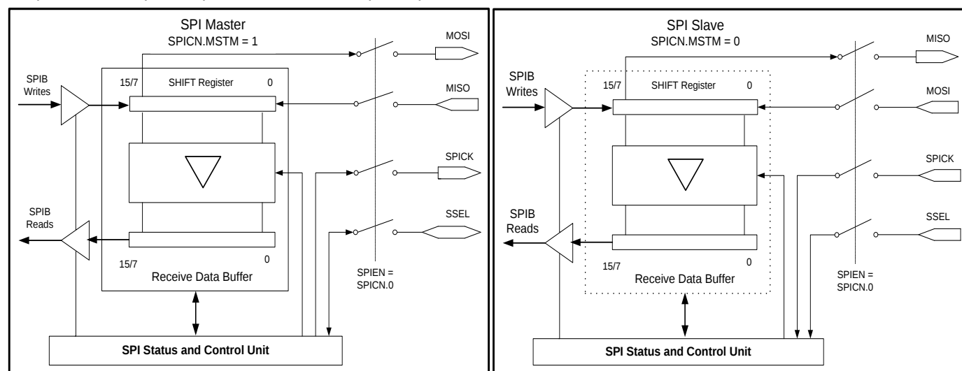
Figure 12-1: SPI Master and Slave Block Diagram
