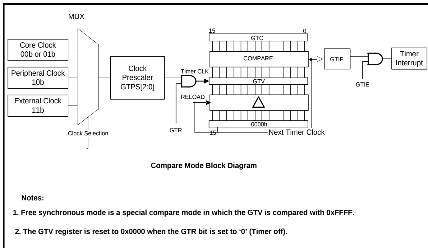
Figure 16-1: Timer Functional Diagram
