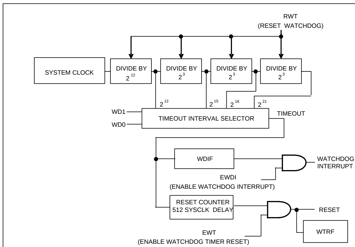
Figure 19-1: Watchdog Timer Block Diagram
