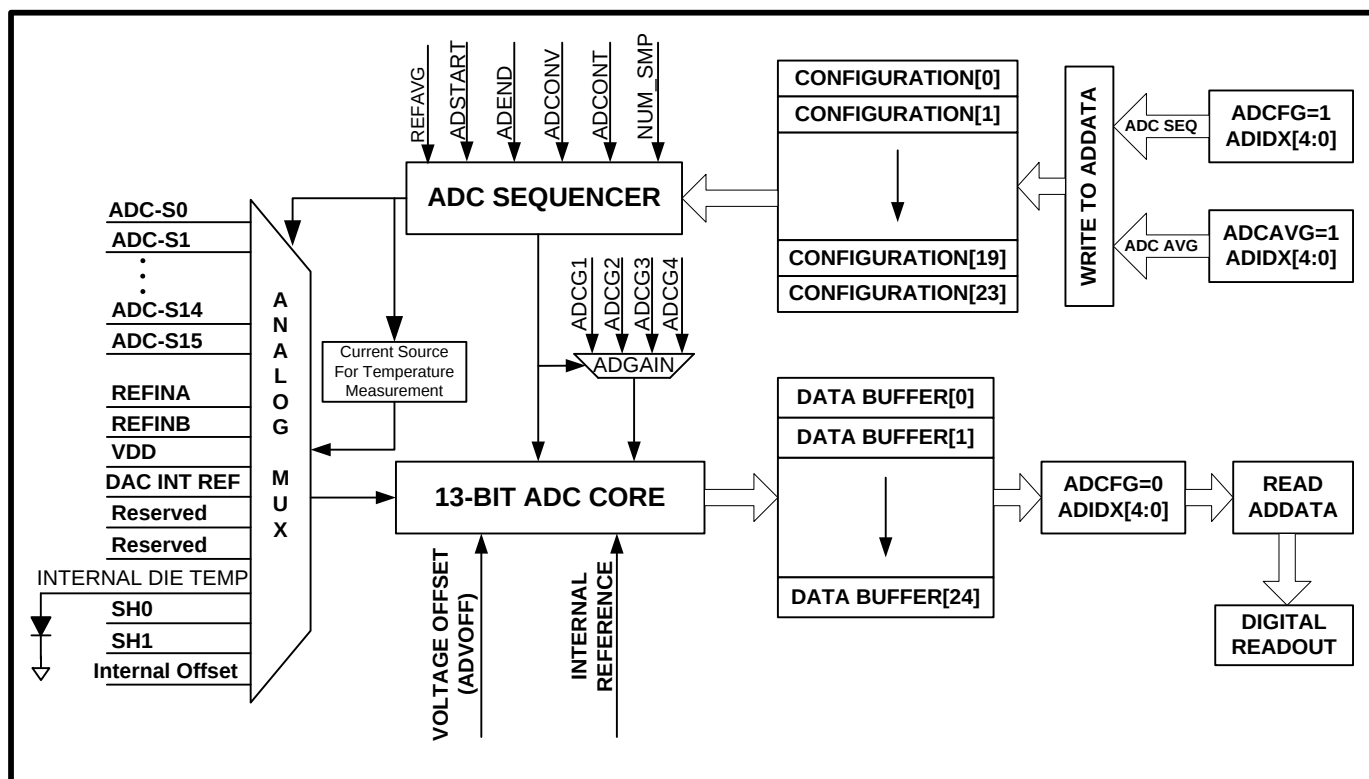
Figure 7-1: ADC Functional Diagram
