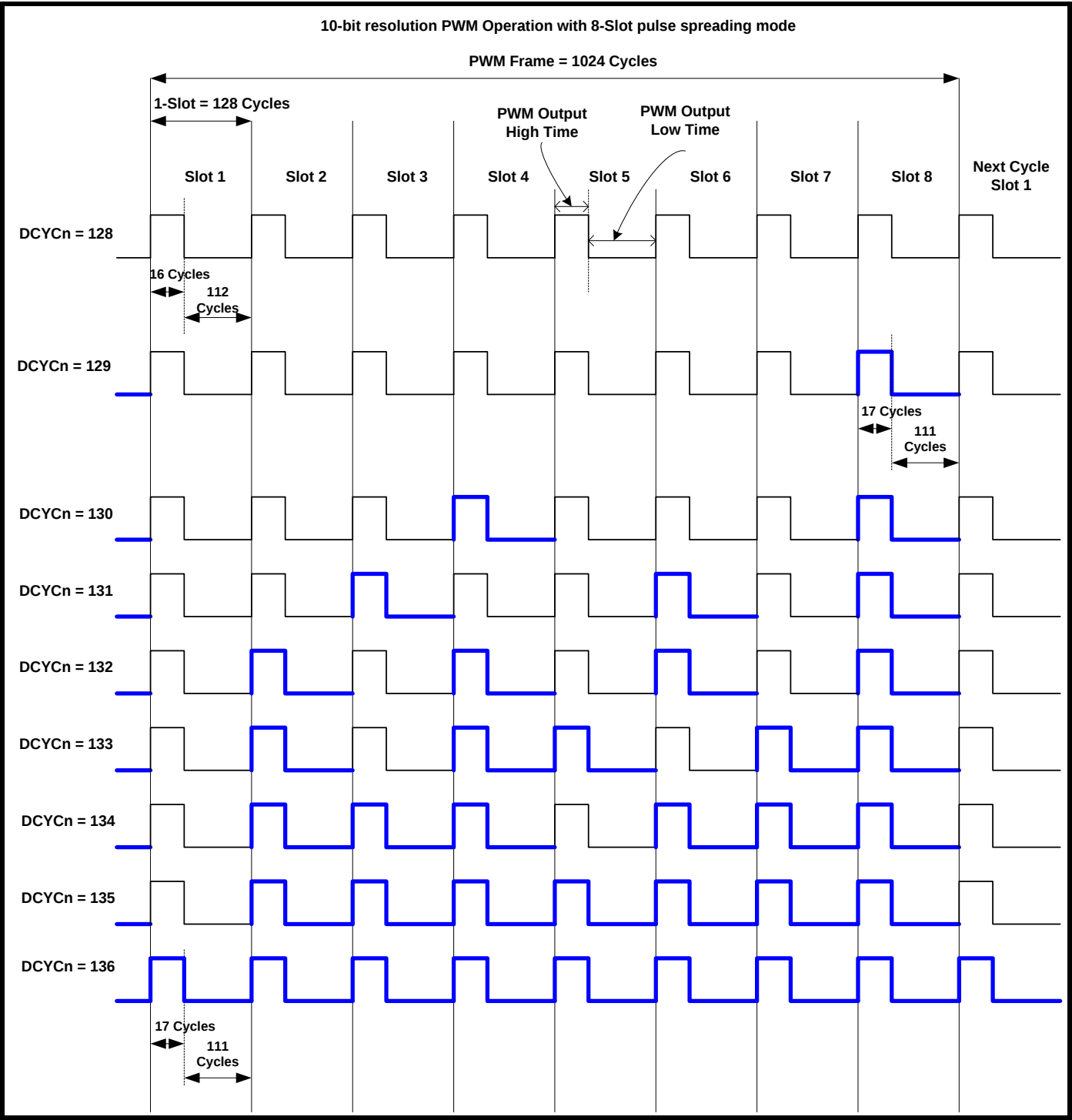
Figure 14-5: Duty Cycle Distribution with 8-Slot Pulse Spreading (PS[1:0] = 11b) for 10-Bit PWM Operation
