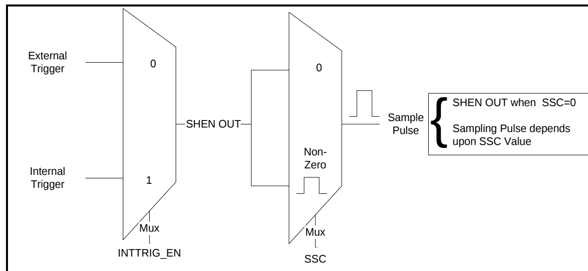
Figure 8-3: Sample Pulse
