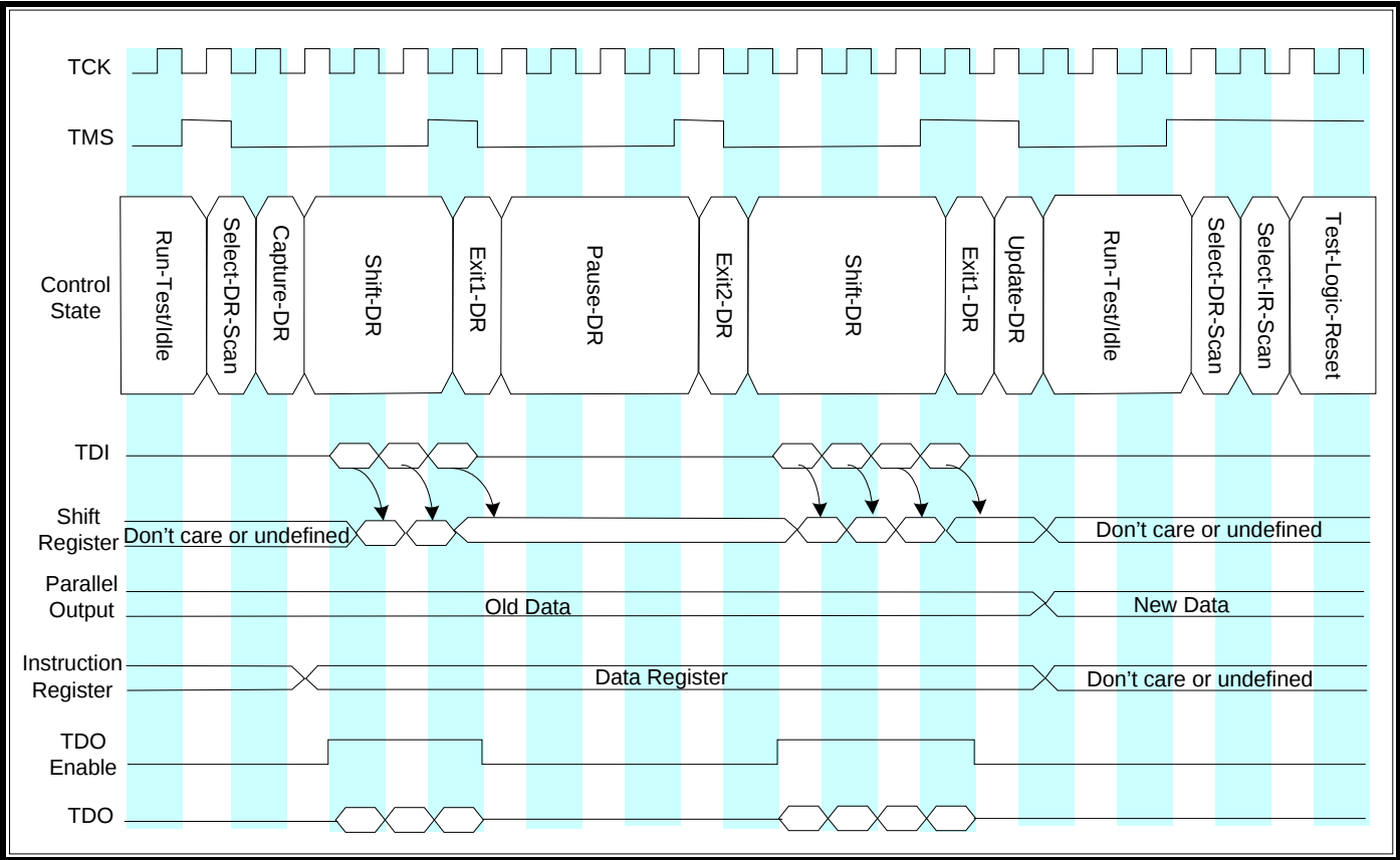
Figure 20-4: TAP Controller Debug Mode DR-Scan Example
