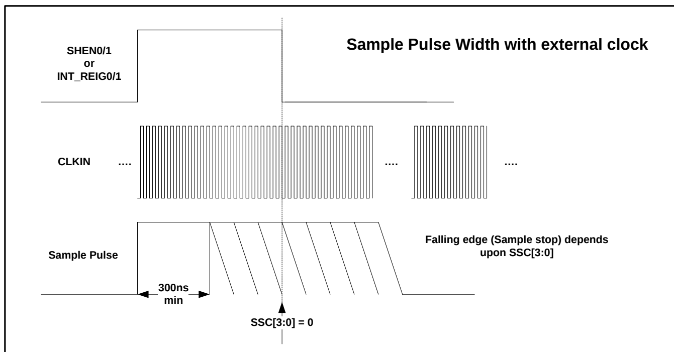
Figure 8-5: Sample Pulse Width with the External Clock
