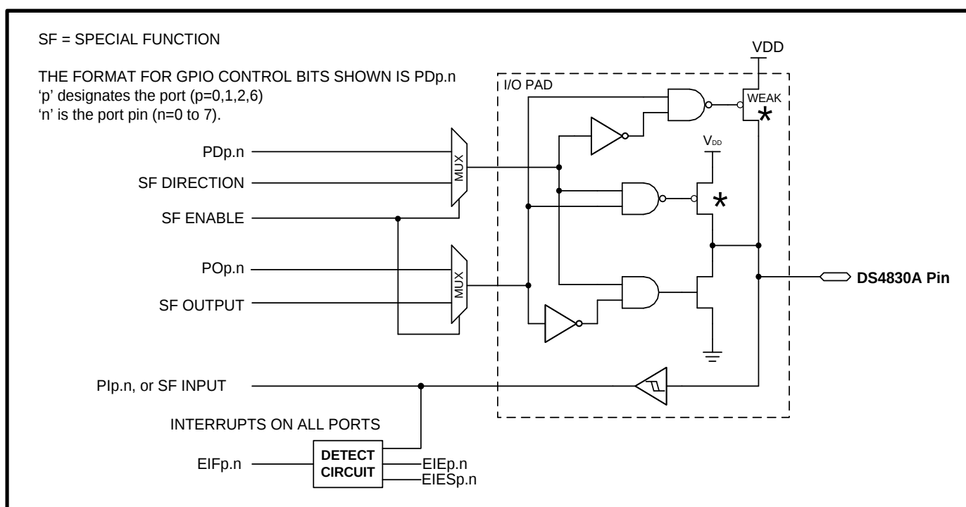
Figure 15-1: GPIO Pin Block Diagram
