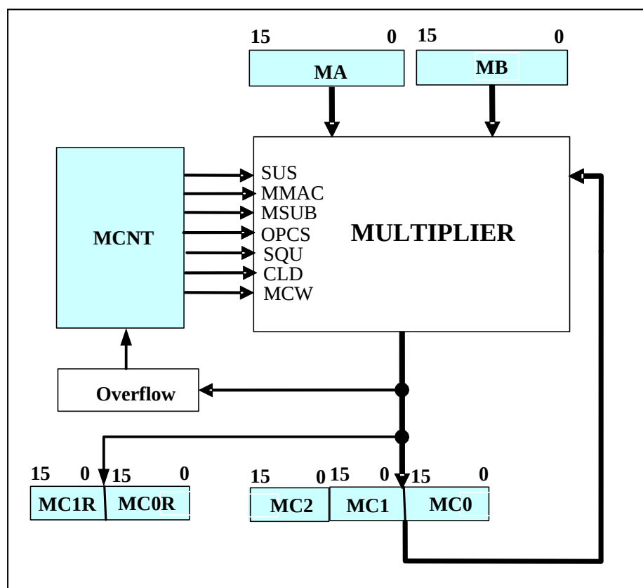
Figure 18-1: Multiplier Organization
