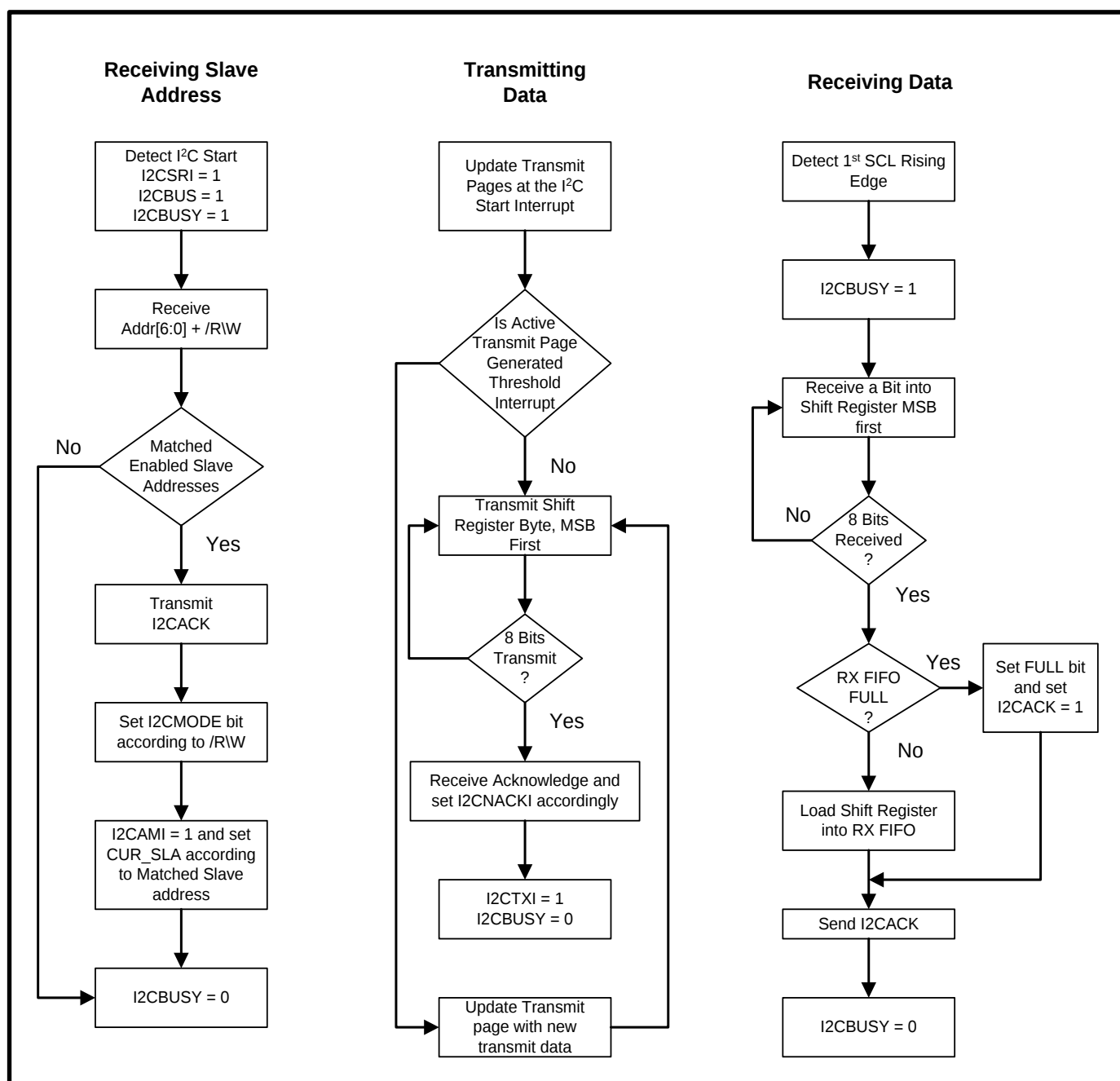
Figure 11-4: Slave I²C Data Flow Using 8-Byte Transmit Page and 8-Byte Receive FIFO
