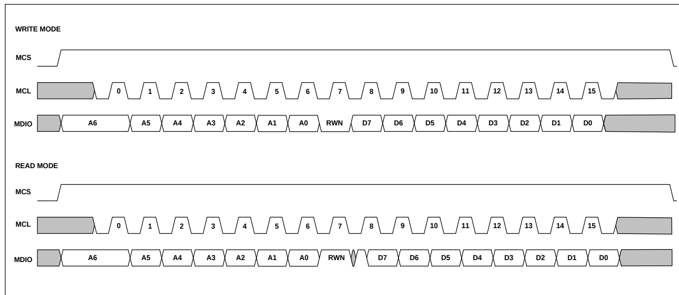
Figure 13-1: 3-Wire Write and Read Operation
