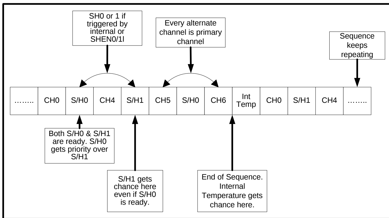
Figure 7-3: ADC Frame Sequence
