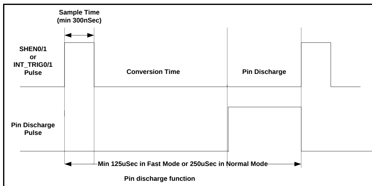
Figure 8-6: Pin Discharge Operation
