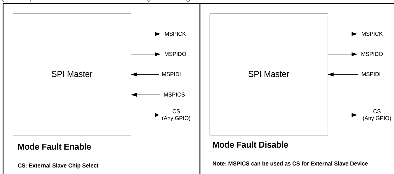
Figure 12-4: SPI Master Pin Configurations with Mode Fault Enable and Disable
