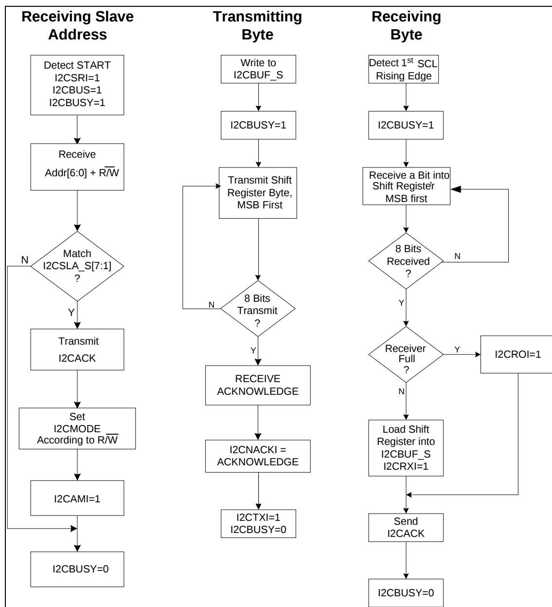
Figure 11-2: Slave I 2 C Data Flow
