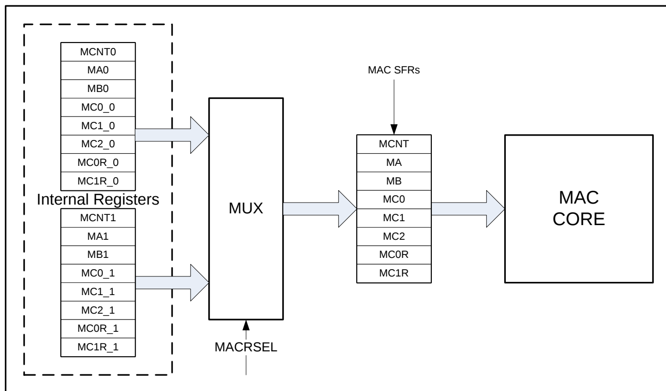
Figure 18-2: Dual MAC Registers Organization
