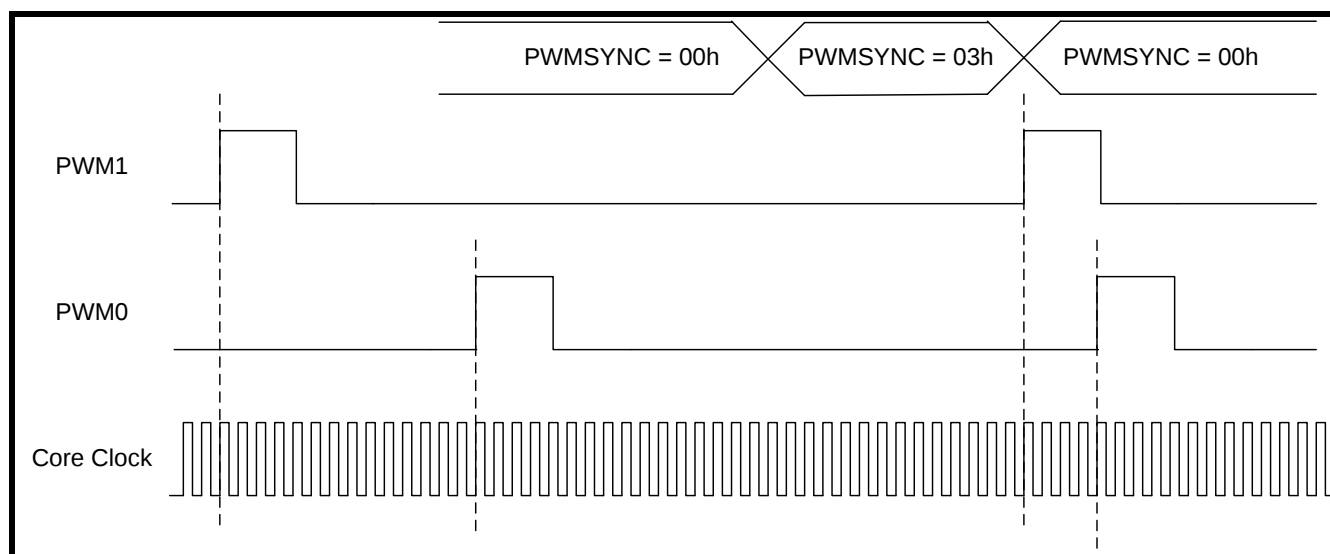
Figure 14-7: PWM Output Synchronization with 4 Clocks Delay
