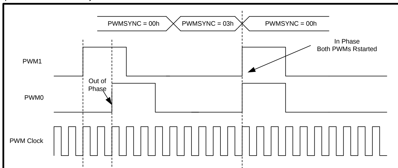
Figure 14-2: PWM Output Synchronization When the Same Delay is Programmed
