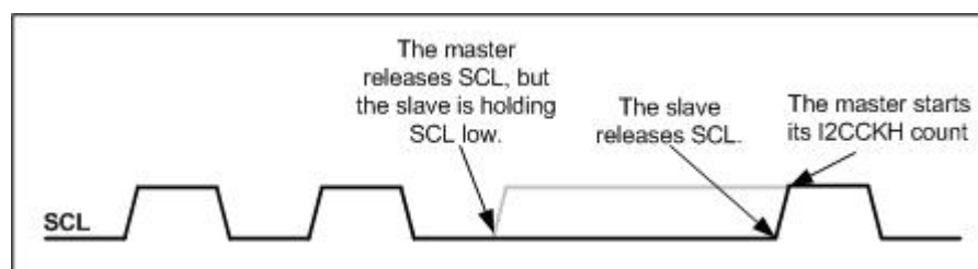
Figure 10-2: Master I 2 C Clock Generation During Slave Clock Stretching
