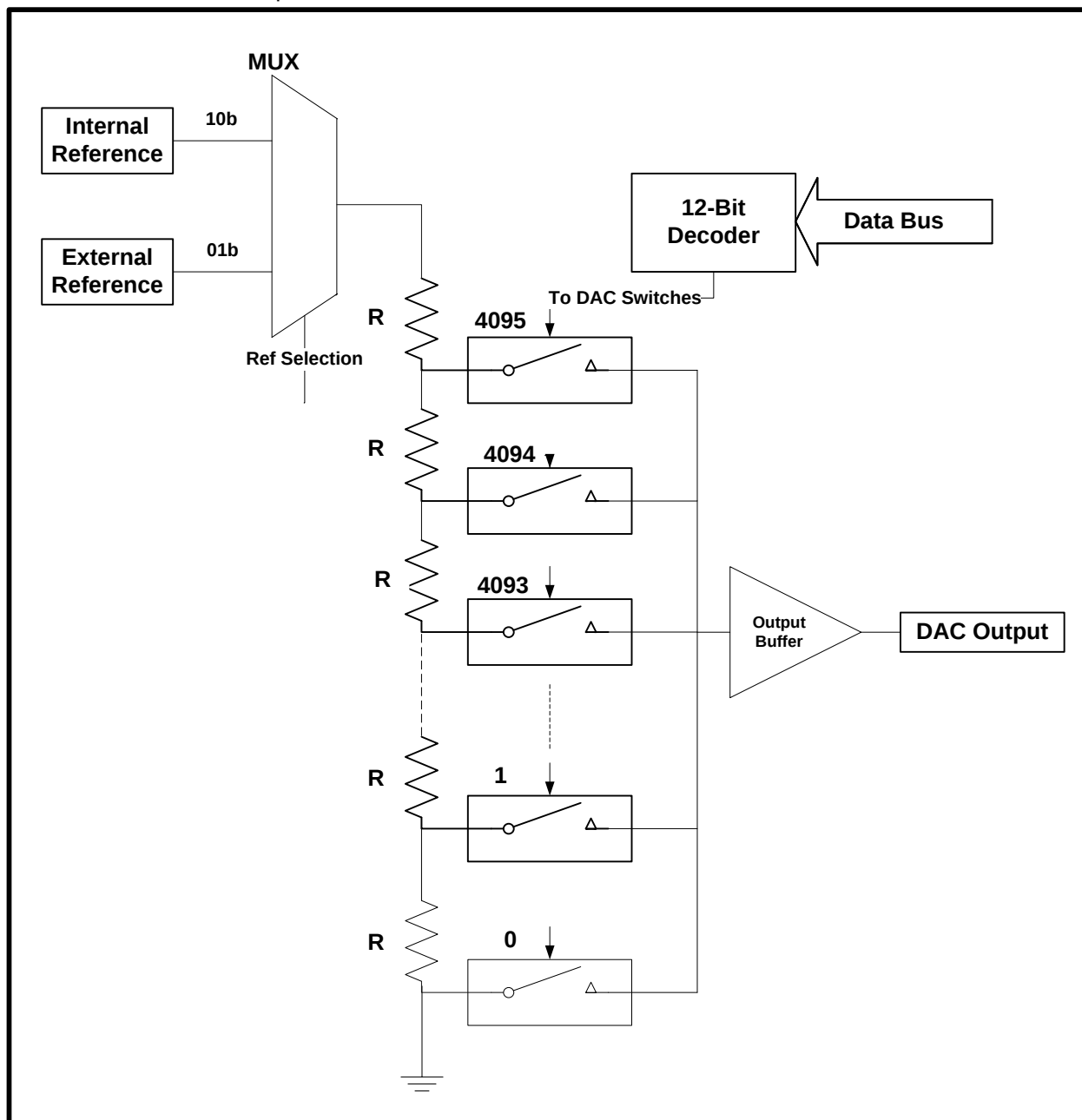
Figure 6-1: DAC Functional Diagram
