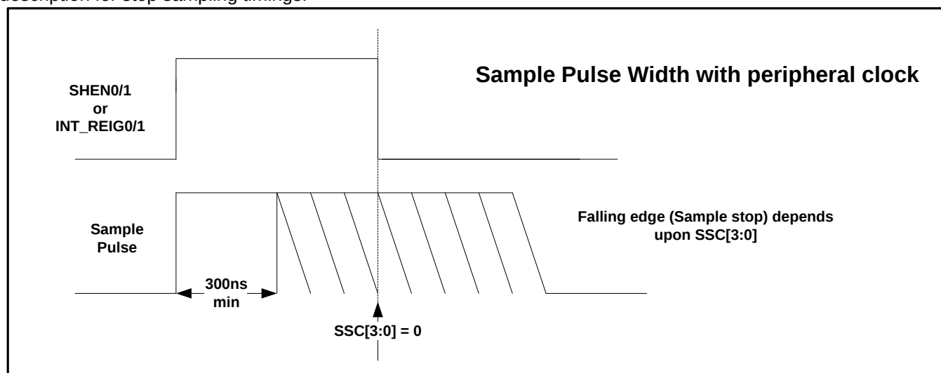
Figure 8-4: Sample Pulse Width with the Peripheral Clock
