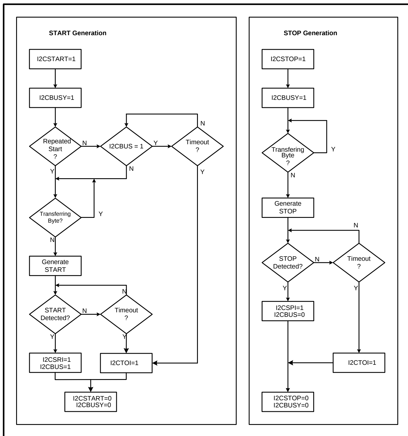
Figure 10-3: Master I 2 C-Generated START and STOP
