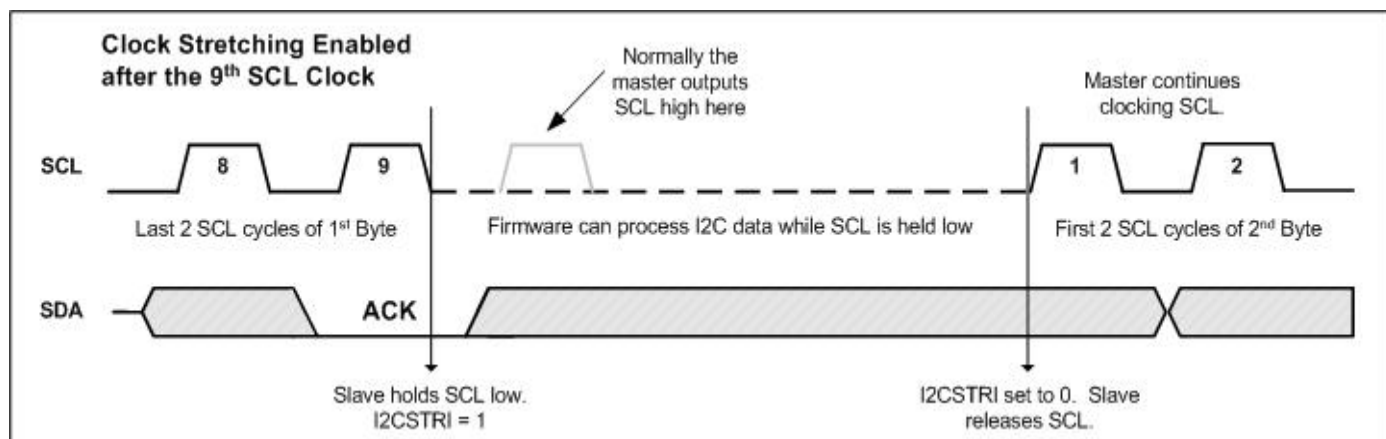
Figure 11-5: Slave I 2 C Clock Stretching
