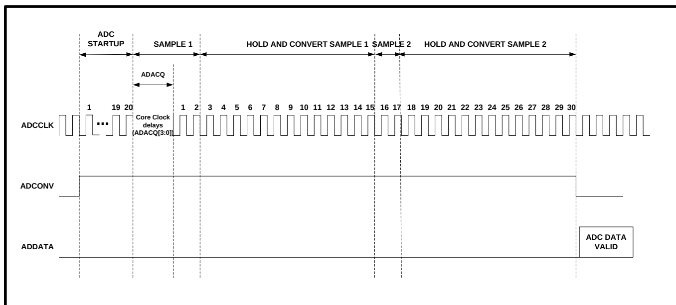
Figure 7-4: Extended Acquisition Time
