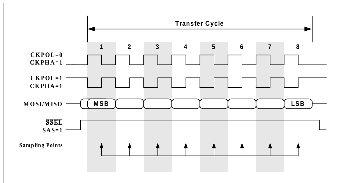
Figure 12-2: SPI Transfer Formats (CKPHA=1)
