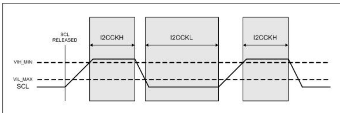
Figure 10-1: I 2 C Clock Generation
