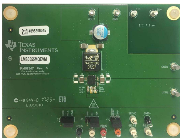
Figure 1. LMS3635xQEVM and LMS3655xQEVM Evaluation Board – Top View
