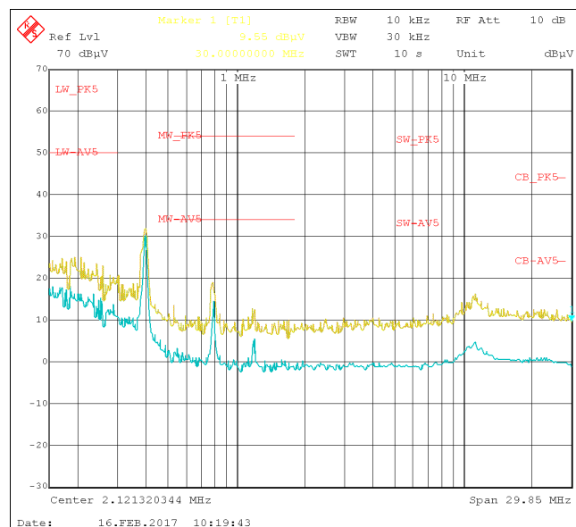
Figure 19. LMS3655MQEVM Low Frequency Conducted EMI Results for 5 Vout With Spread Spectrum. Blue-Average and Yellow-Peak
