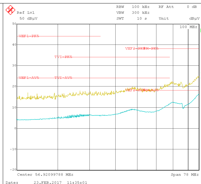
Figure 20. LMS3655MQEVM High Frequency Conducted EMI Results for 5 Vout With Spread Spectrum. Blue-Average and Yellow-Peak
