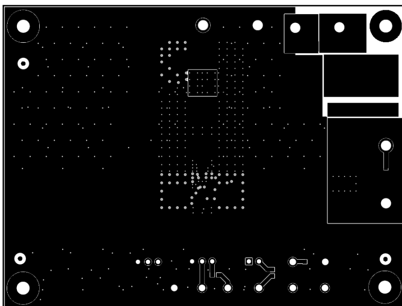
Figure 8. PCB Layer Bottom Layer 4 – Flipped View (as Seen From Bottom of Board)
