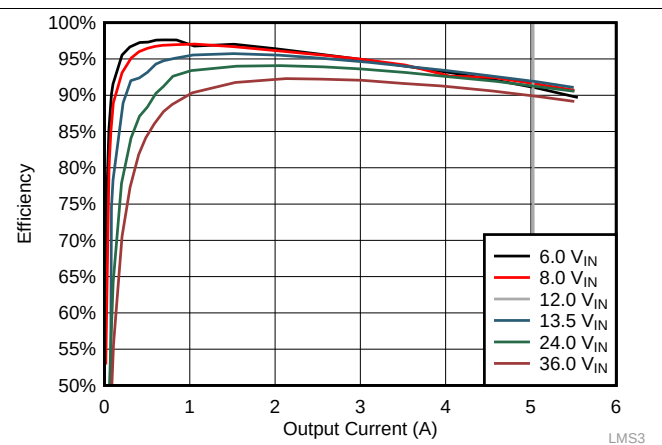
Figure 13. LMS3655MQEVM Efficiency
