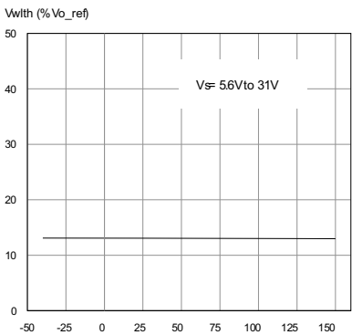
Figure 17. V_{wlth} vs. T_j
