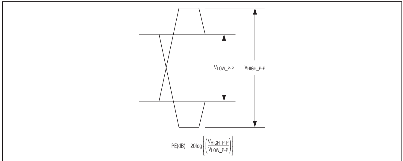
Figure 1. Output Preemphasis
