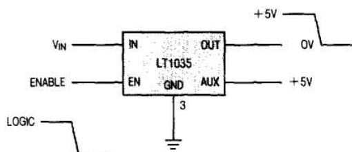
Functional Diagram
