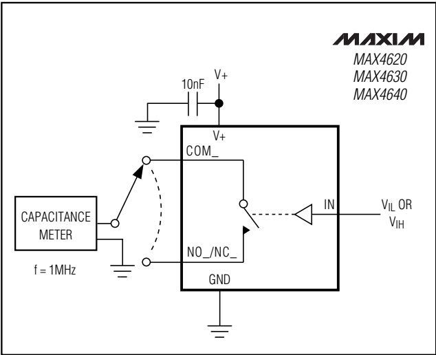
Figure 3. Channel Off/On-Capacitance
