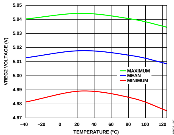
Figure 9. VREG2 Voltage vs. Temperature
