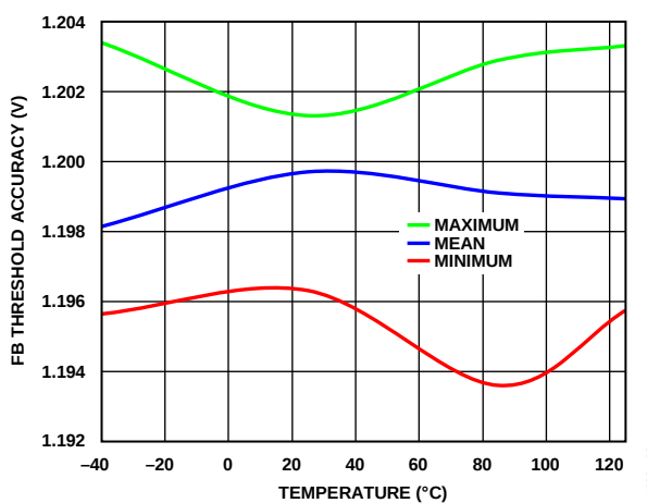
Figure 10. FB Threshold vs. Temperature
