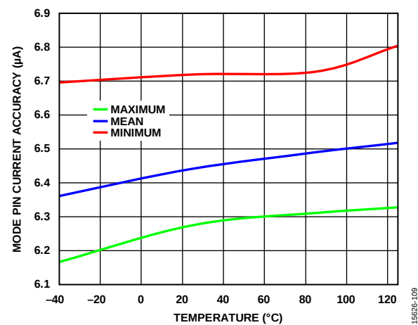
Figure 11. MODE Pin Current Source Accuracy vs. Temperature
