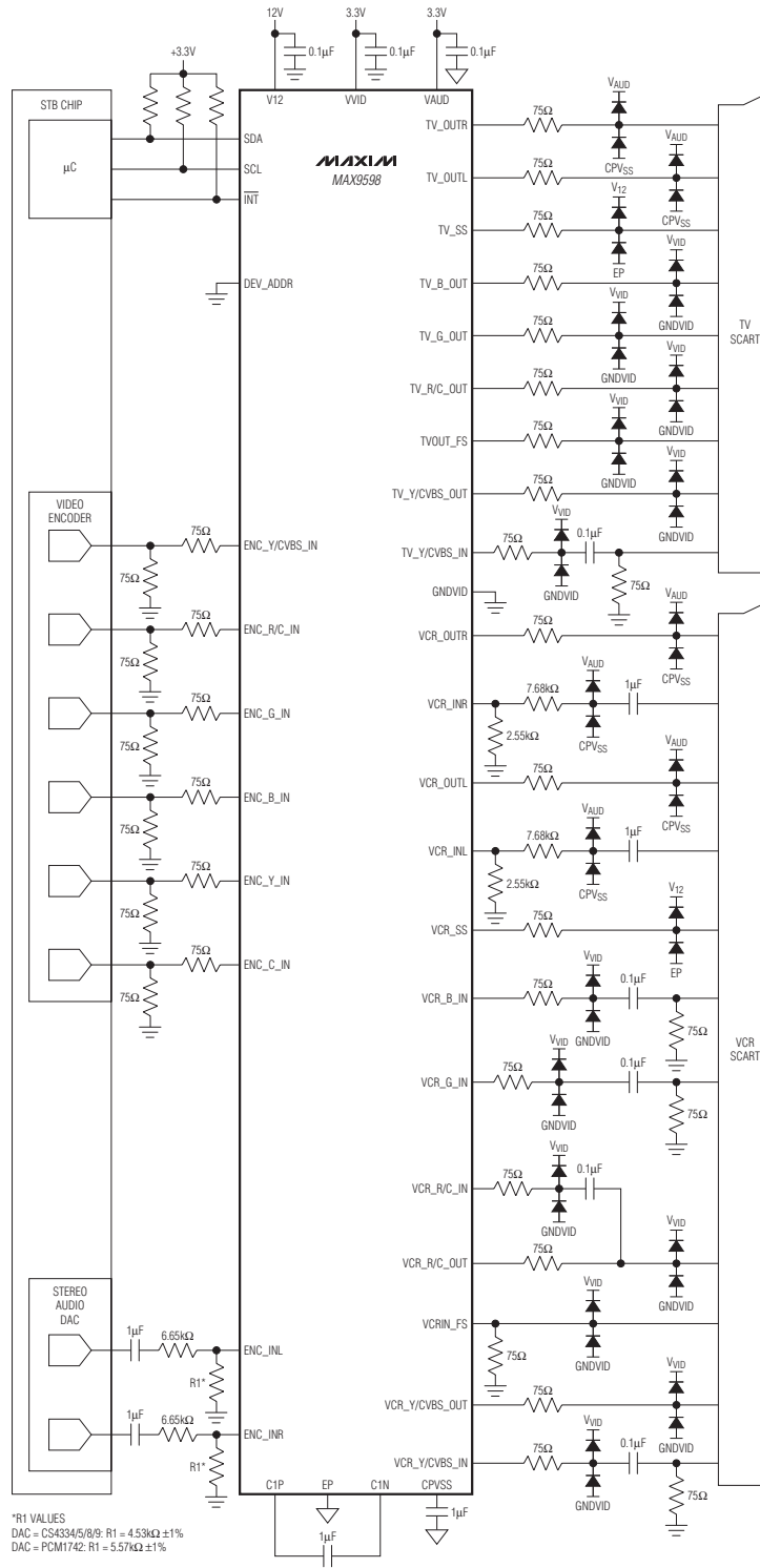
Figure 17. Application Circuit to Connect Series Resistors and External ESD Protection Diodes at MAX9598 Outputs
