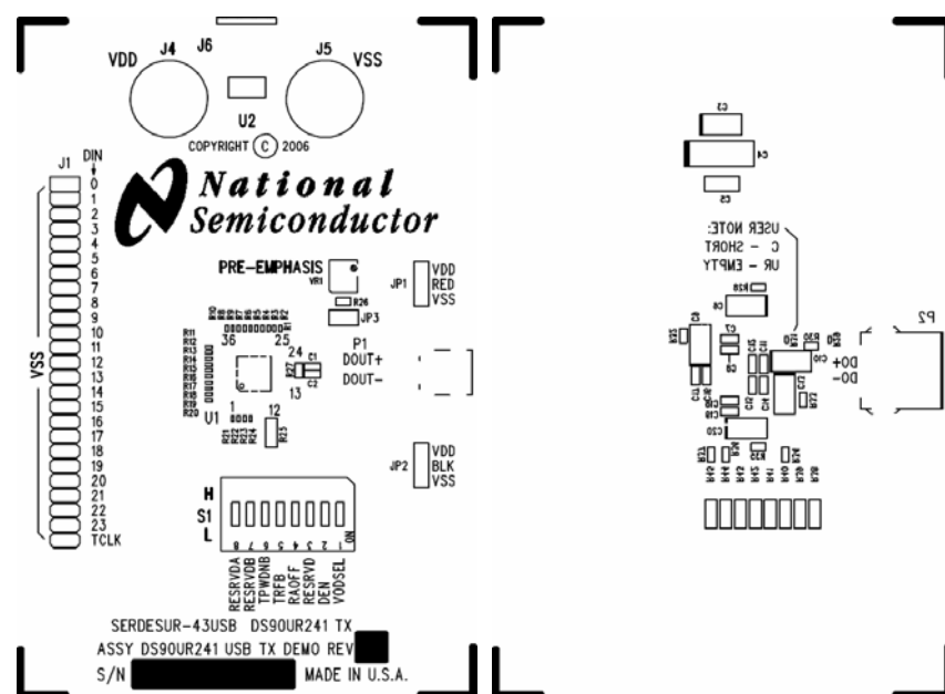
SILKSCREEN COMP SIDE – SILKSCREEN (LAYER 4)
