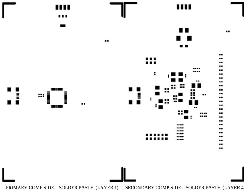
PRIMARY COMP SIDE – SOLDER PASTE (LAYER 1) SECONDARY COMP SIDE – SOLDER PASTE (LAYER 4)
