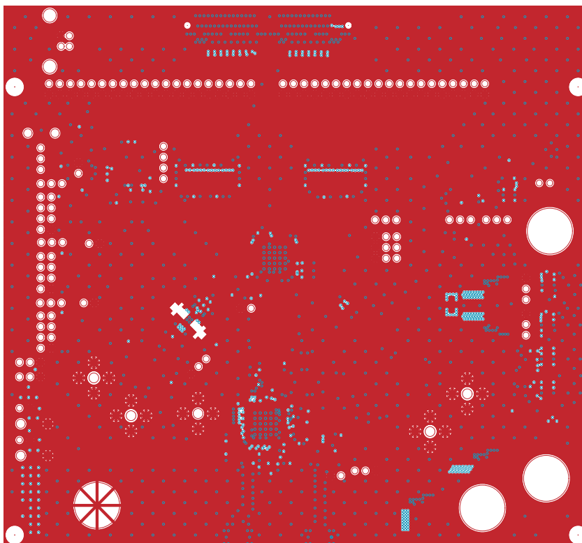
Figure 17. Layer 3
