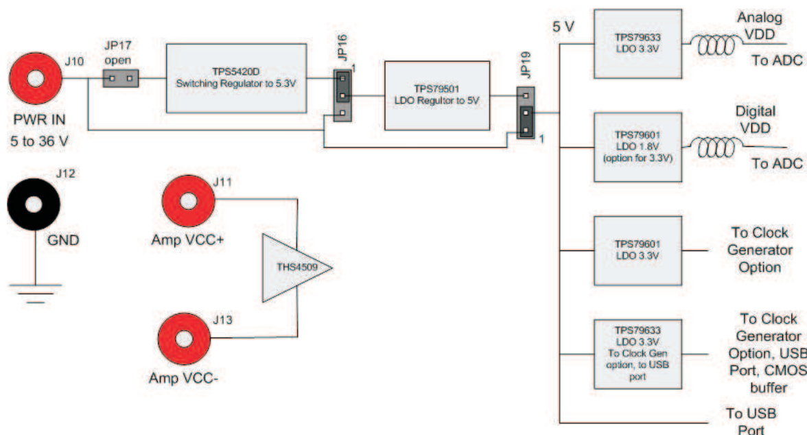
Figure 3. ADS62PXXEVM Power Distribution
