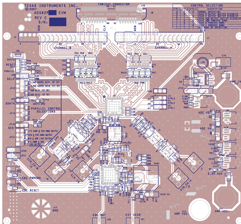
Figure 13. Top Silkscreen
