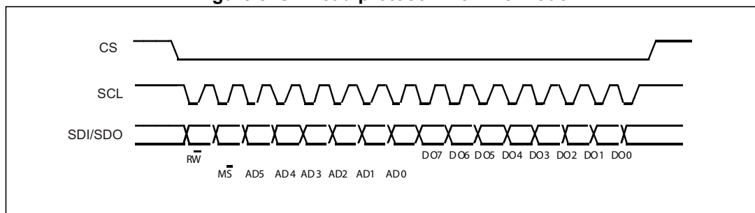
Figure 8. SPI read protocol in 3-wire mode
