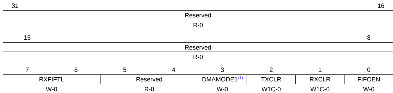
Figure 26-13. FIFO Control Register (FCR)
