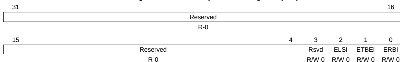
Figure 26-11. Interrupt Enable Register (IER)
