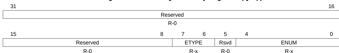
Figure 16-57. Event Queue Entry Registers (QxEy)
