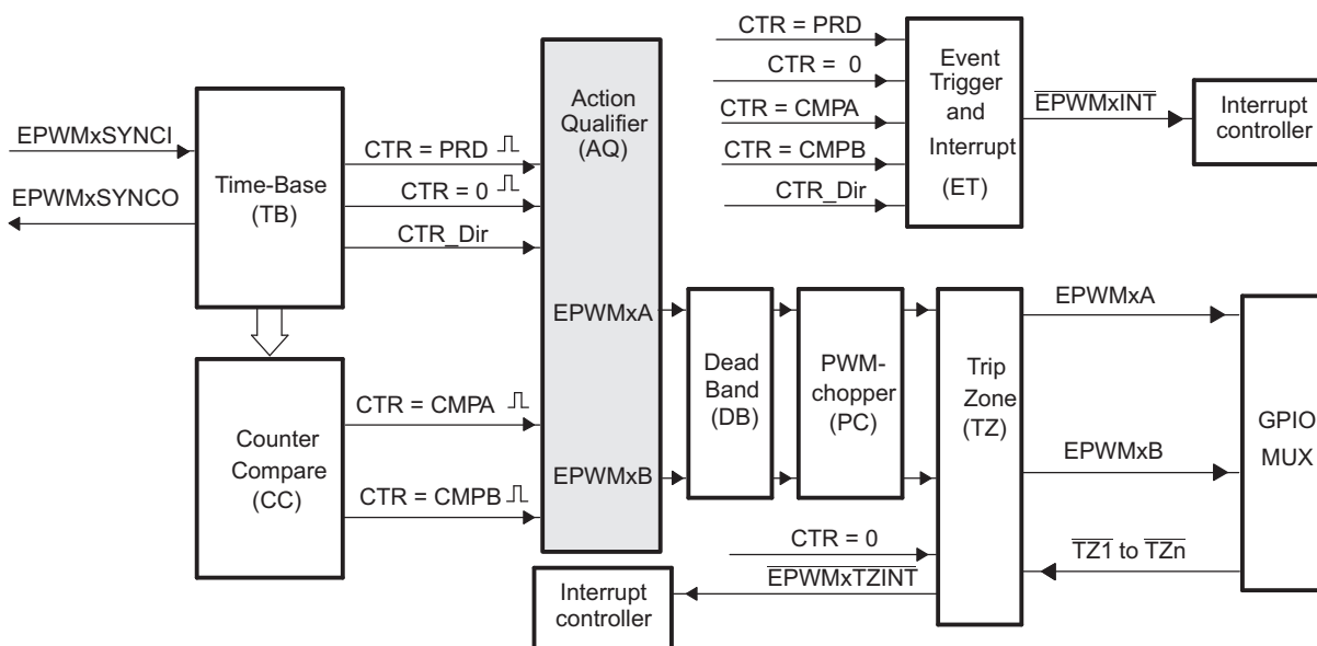
Figure 14-18. Action-Qualifier Submodule
