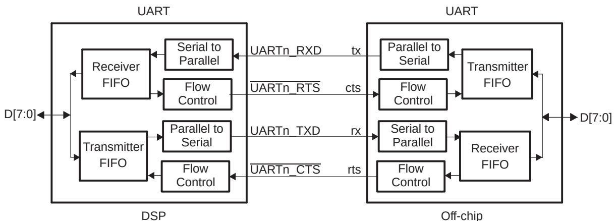
Figure 26-5. UART Interface Using Autoflow Diagram
