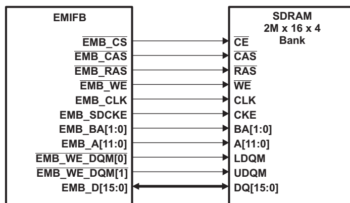
Figure 19-3. EMIFB to 2\text{M} \times 16 \times 4 bank SDRAM Interface
