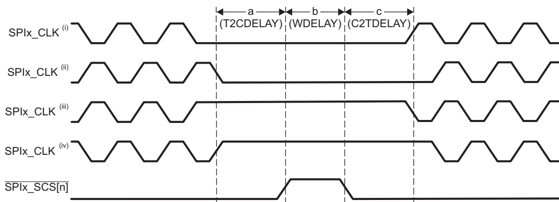
Figure 24-14. SPI 4-Pin with \overline{\text{SPIx\_SCS}}[n] Mode with T2CDELAY, WDELAY, and C2TDELAY
