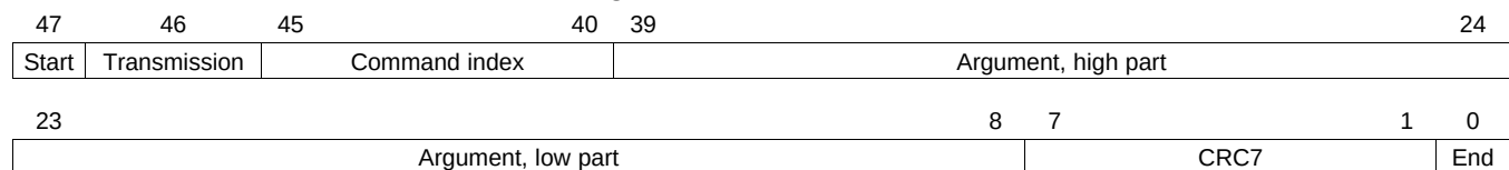
Figure 23-30. Command Format
