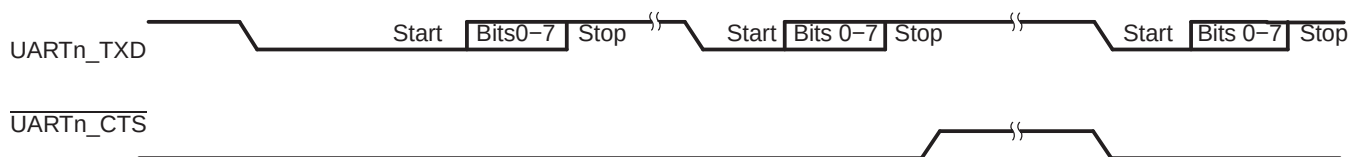
Figure 26-7. Autoflow Functional Timing Waveforms for UARTn_CTS
