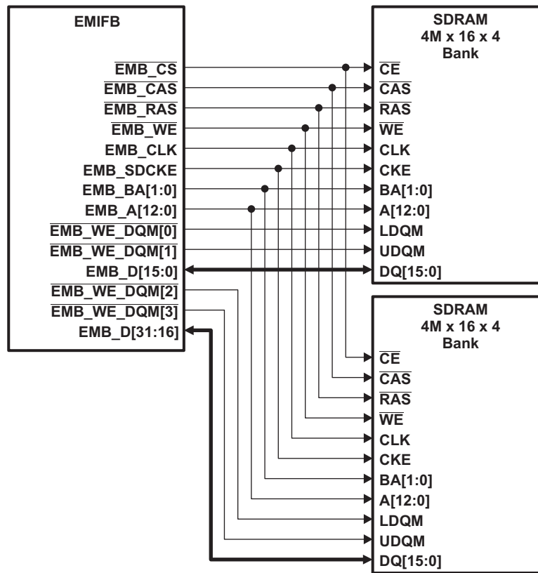
Figure 19-5. EMIFB to Dual 4M × 16 × 4 bank SDRAM Interface
