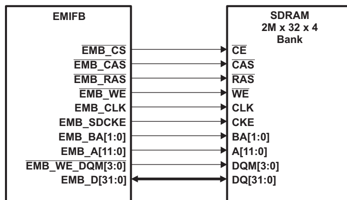
Figure 19-4. EMIFB to 2\text{M} \times 32 \times 4 bank SDRAM Interface
