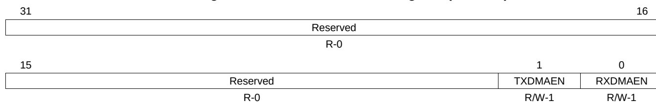
Figure 21-29. I2C DMA Control Register (ICDMAC)
