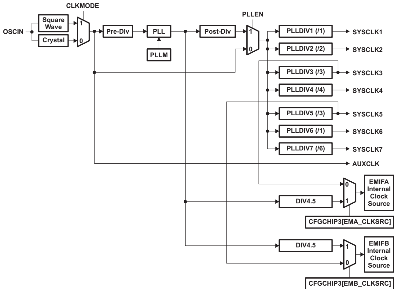
Figure 7-1. PLL0 Structure
