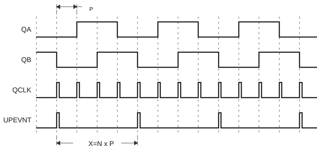
Figure 15-16. Unit Position Event for Low Speed Measurement ( QCAPCTL[UPPS] = 0010 )
