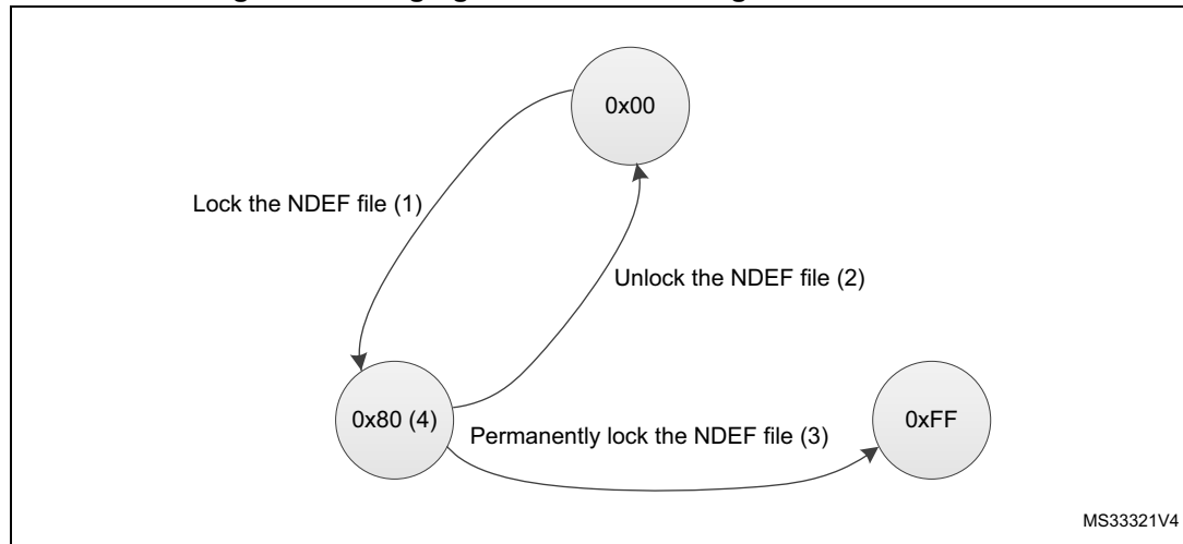
Figure 3. Changing the write access right to an NDEF file
