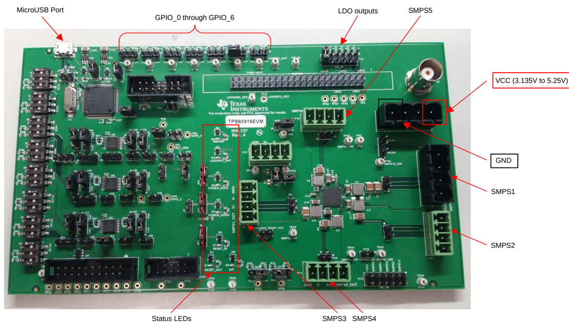
Figure 1. EVM
