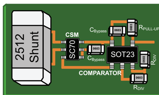
INA199 + Comp. footprint is approx. 29mm 2
