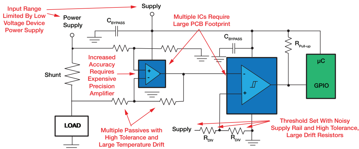
Discrete Current Detection – Op Amp plus Comparator Block Diagram
