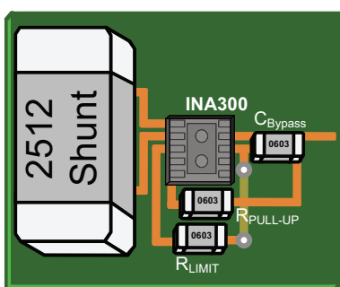
INA300 footprint is approx. 14mm 2
