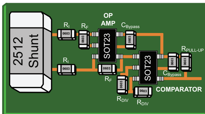
Op-Amp + Comp. footprint is approx. 47mm 2
