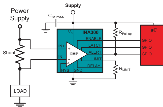
Single-Chip Over-Current Detection Solution Block Diagram
