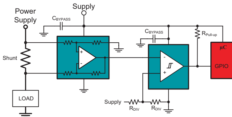
Current Sense Amplifier plus Comparator Block Diagram
