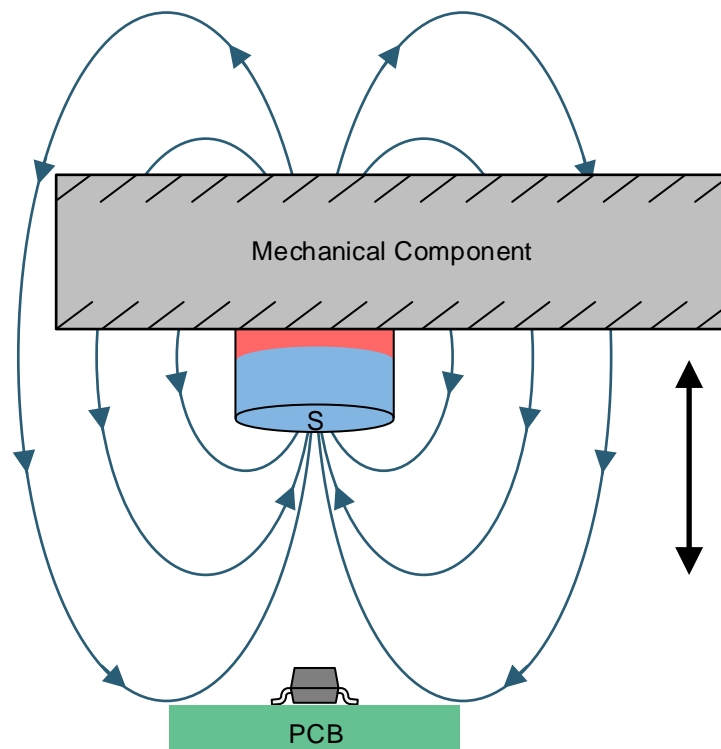
Figure 20. Physical Setup
