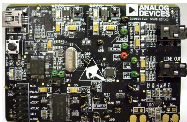
Figure 1. Top View of the SSM2604 Evaluation Board
