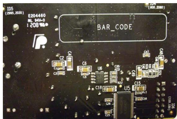
Figure 2. Bottom View of the SSM2604 Evaluation Board
