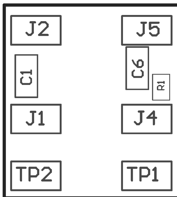
Figure 19. Bottom Assembly
