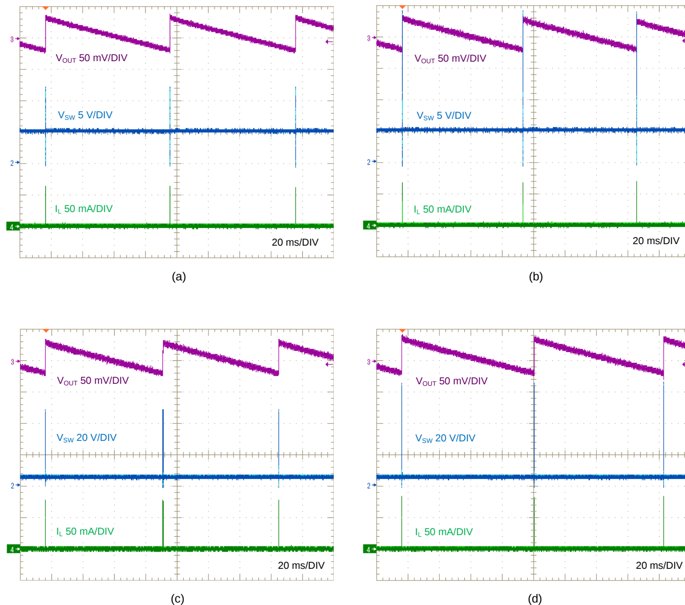
Figure 5. SW Node, V_{OUT} and I_L Waveforms at I_{OUT} = 0 mA: (a) V_{IN} = 12 V, (b) V_{IN} = 24 V, (c) V_{IN} = 36 V, (d) V_{IN} = 65 V
