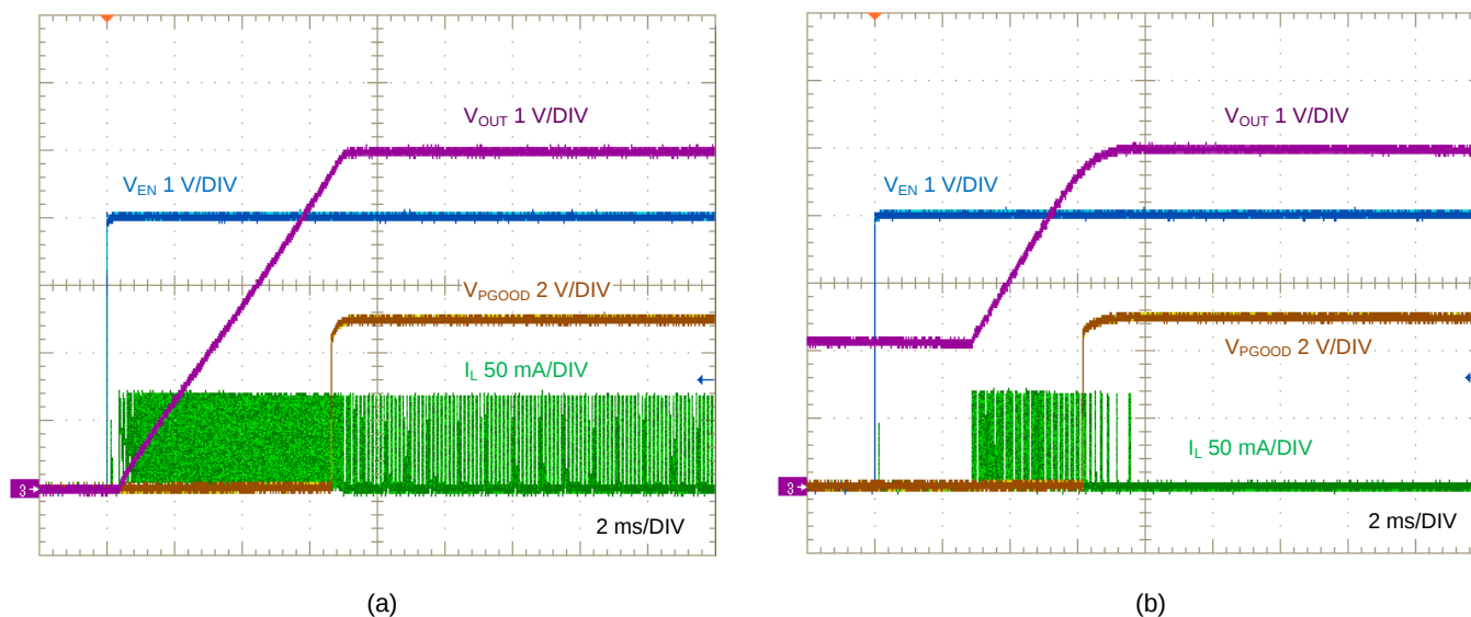
Figure 9. Enable ON at V_{IN} = 24 V: (a) I_{OUT} = 12.5 mA, (b) No Load, 2-V Output Pre-bias
