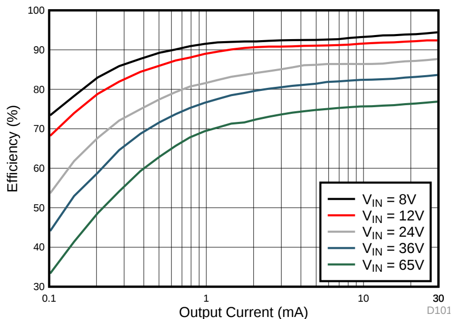
Figure 4. PFM Converter Efficiency, V_{OUT} = 5 V
