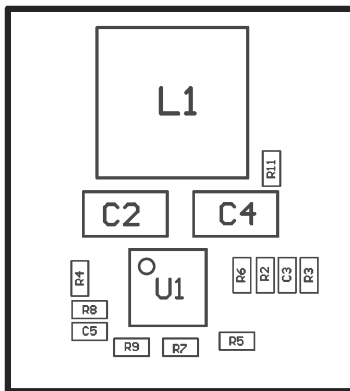
Figure 18. Top Assembly
