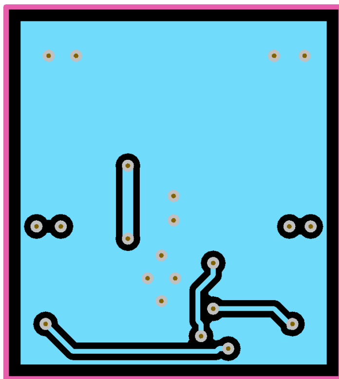
Figure 16. Layer 3 (Top View)
