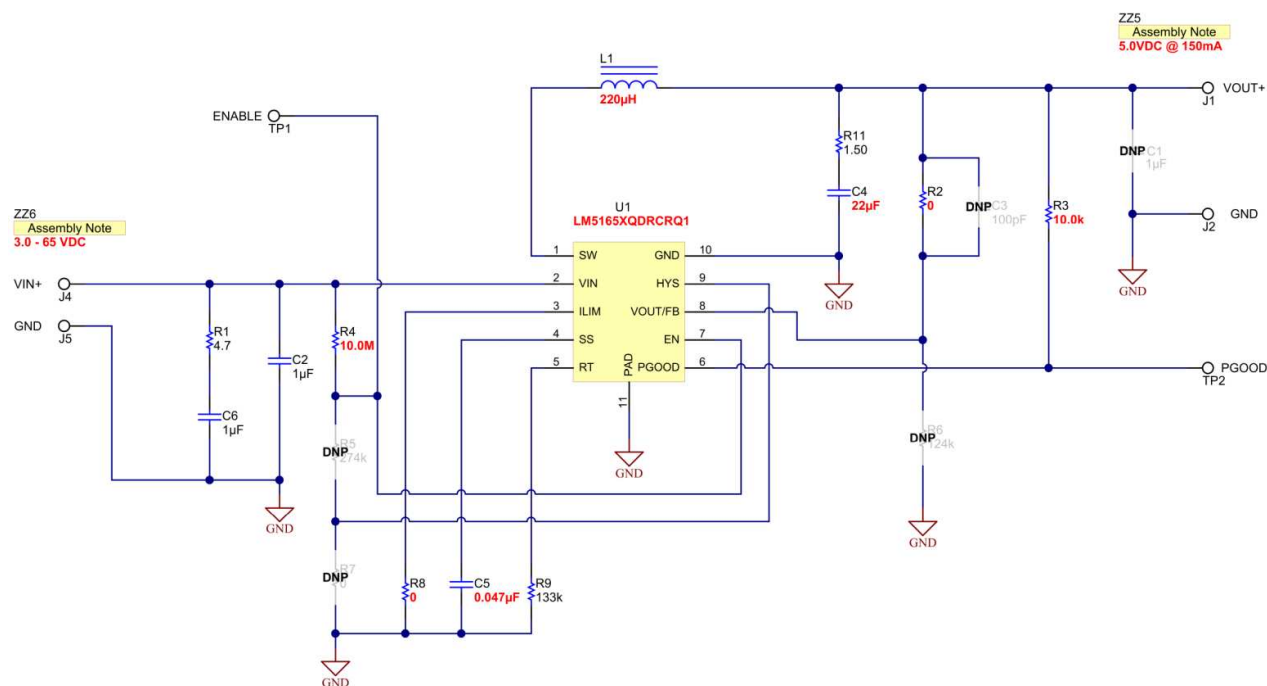
Figure 20. COT, 5V, 150mA Schematic (Fixed 5V Output Version)
