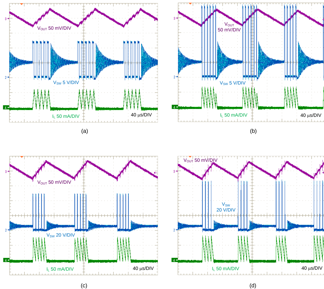
Figure 6. SW Node, V_{OUT} and I_L Waveforms at I_{OUT} = 12.5 \text{ mA} : (a) V_{IN} = 12 \text{ V} , (b) V_{IN} = 24 \text{ V} , (c) V_{IN} = 36 \text{ V} , (d) V_{IN} = 65 \text{ V}
