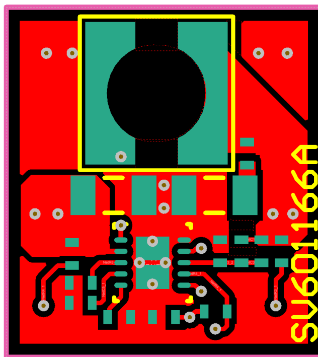
Figure 14. Top Copper (Top View)
