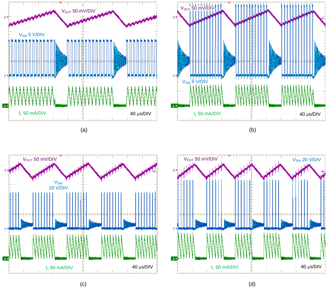
Figure 7. SW Node, V_{OUT} and I_L Waveforms at I_{OUT} = 25 mA: (a) V_{IN} = 24 V, (b) V_{IN} = 24 V, (c) V_{IN} = 36 V, (d) V_{IN} = 65 V
