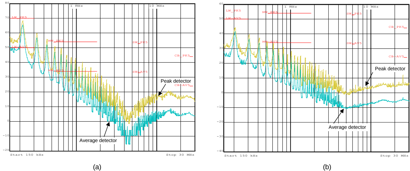
Figure 11. CISPR 25 Class 5 Conducted Emissions Plot, 150 kHz to 30 MHz, V_{IN} = 13.5 V, I_{OUT} = 25 mA: (a) Unfiltered, (b) Filtered
