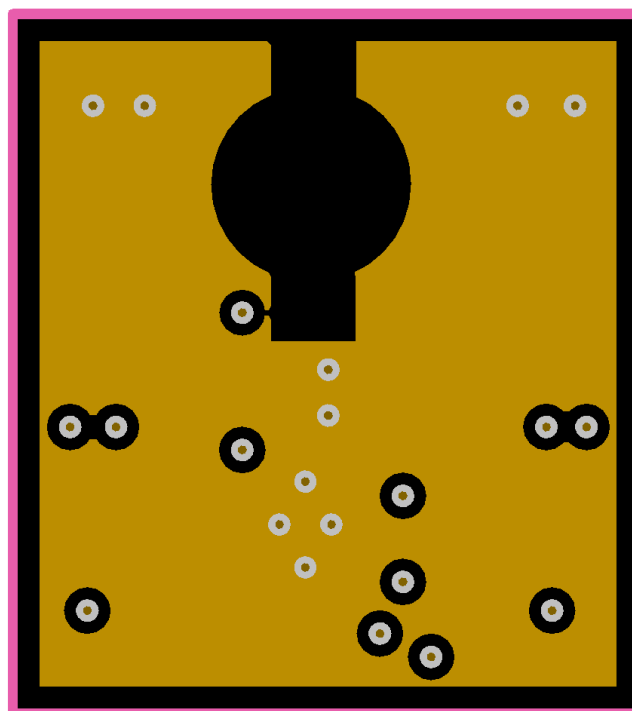
Figure 15. Layer 2 (Top View)
