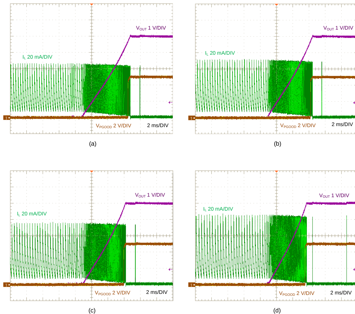
Figure 10. Short Circuit Recovery into No Load: (a) V_{IN} = 12\text{ V} , (b) V_{IN} = 24\text{ V} , (c) V_{IN} = 36\text{ V} , (d) V_{IN} = 65\text{ V}
