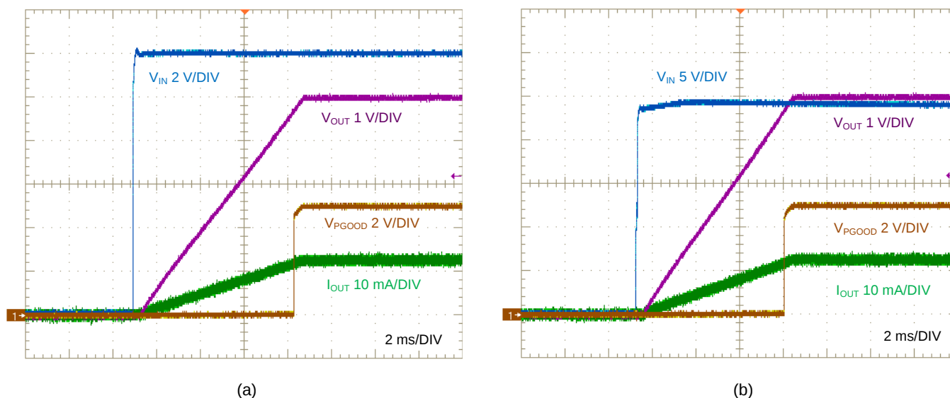
Figure 8. Startup at I_{OUT} = 12.5 mA: (a) V_{IN} = 12 V, (b) V_{IN} = 24 V
