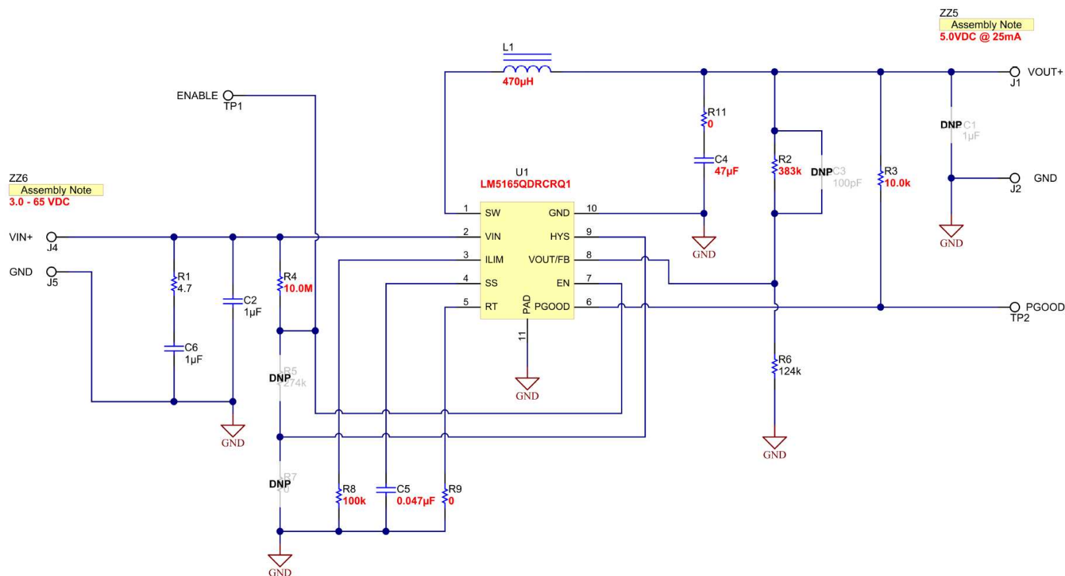
Figure 13. 5V, 25mA PFM Schematic (Adjustable Output Version)
