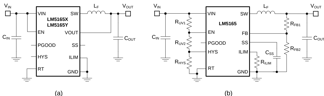
Figure 1. LM5165 PFM-controlled Buck Converter Schematics, (a) Fixed Output of 3.3 V or 5 V, (b) Adjustable Output with Soft-start, Current Limit and Input UVLO Components
