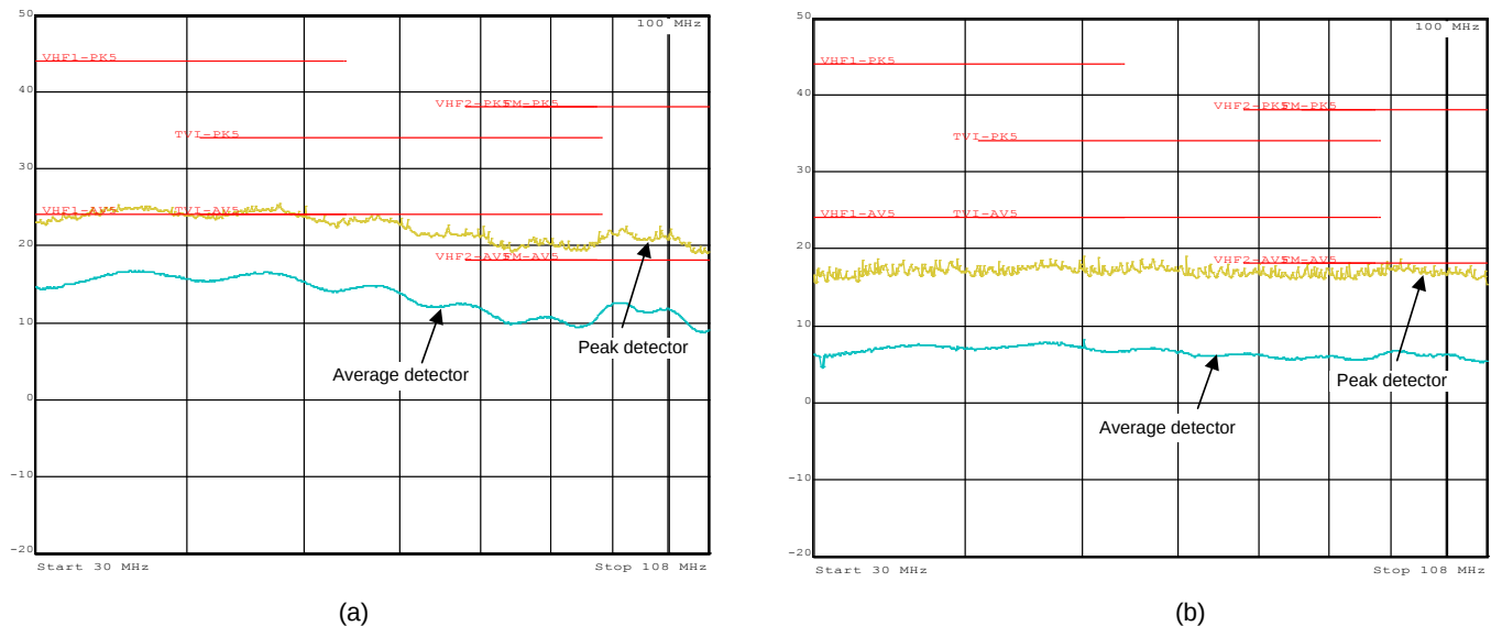
Figure 12. CISPR 25 Class 5 Conducted Emissions Plot, 30 MHz to 108 MHz, V_{IN} = 13.5 V, I_{OUT} = 25 mA: (a) Unfiltered, (b) Filtered
