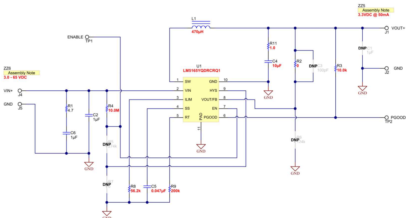
Figure 21. COT, 3.3V, 50mA Schematic (Fixed 3.3V Output Version)
