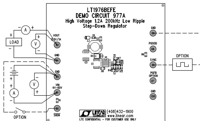
Figure 1. Proper Measurement Equipment Setup
