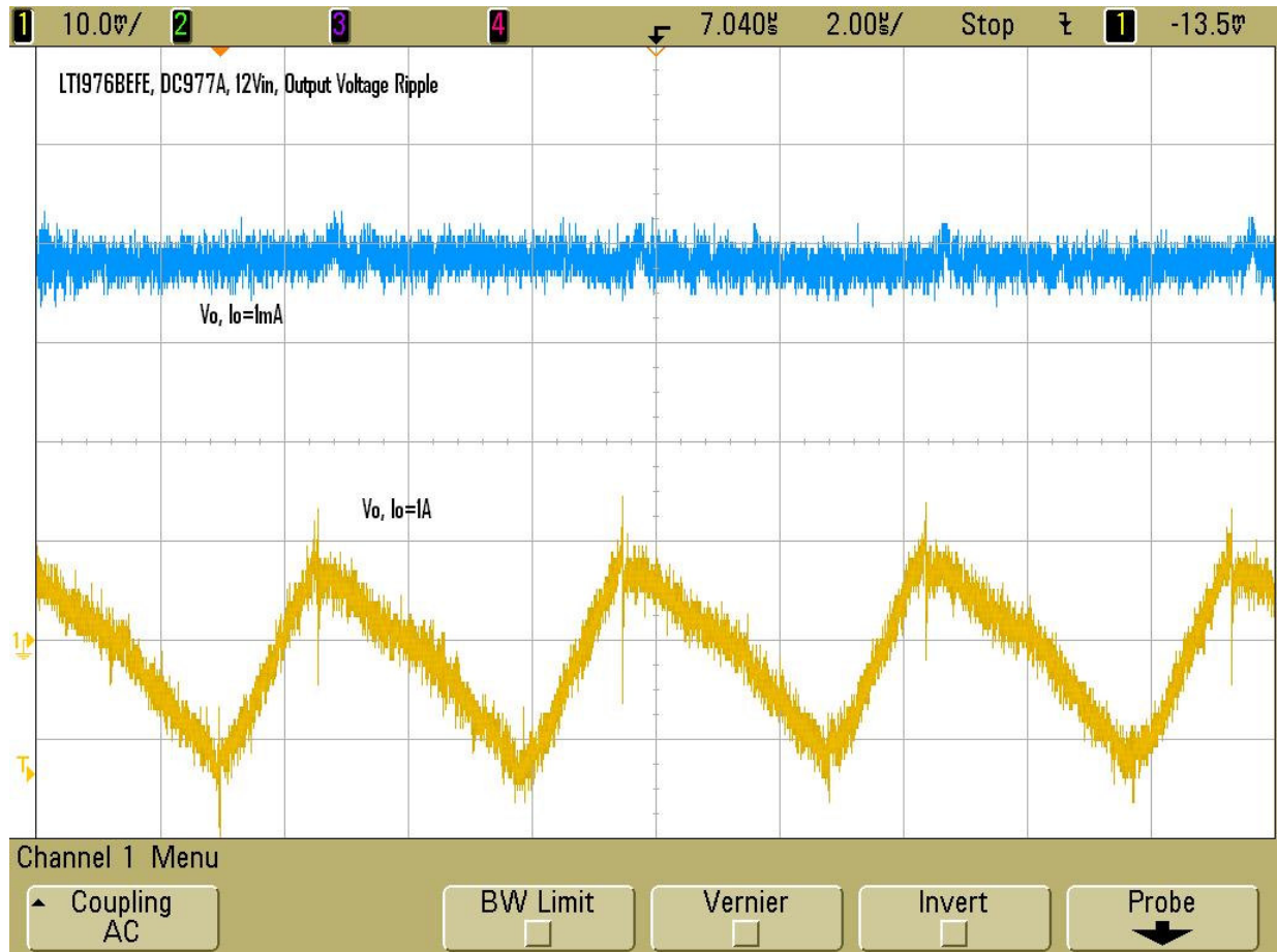
Figure 3. DC977 Typical Low Output Voltage Ripple ( I_{OUT} = 1\text{mA} and 1\text{A} , V_{IN} = 12\text{V} , V_{OUT} = 3.3\text{V} , T_A = 25^\circ\text{C} )
