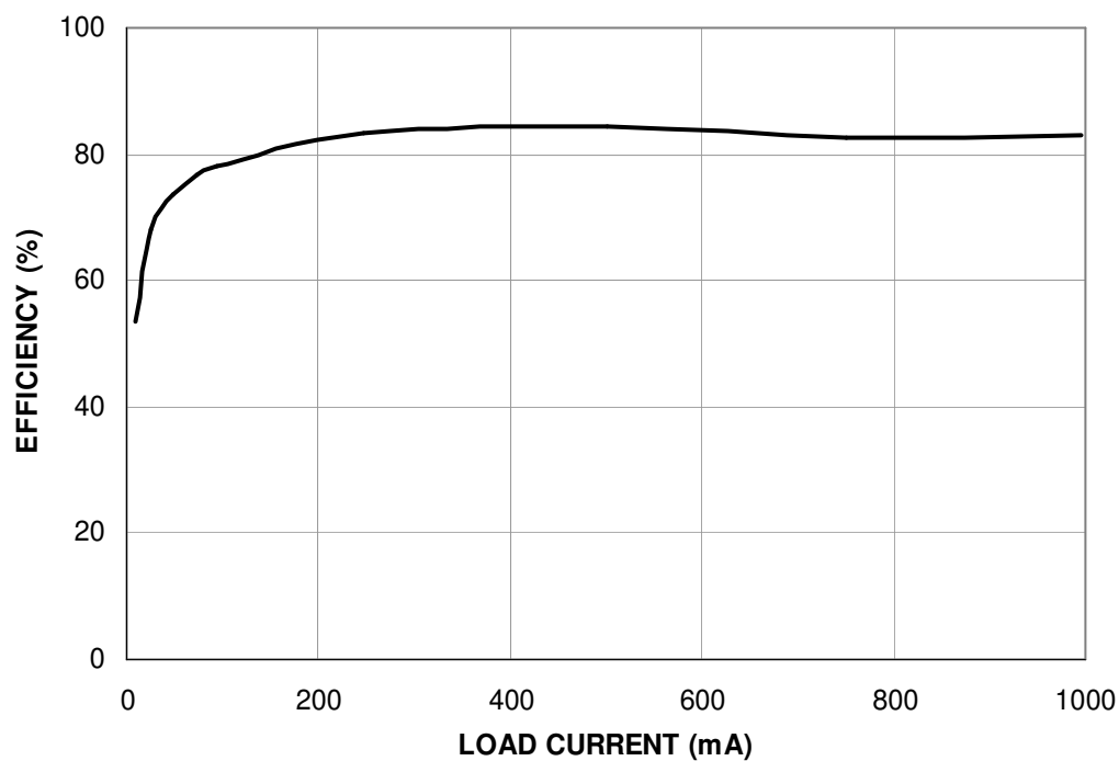
Figure 2. DC977 Typical Efficiency ( T_A = 25^{\circ}\text{C} , V_{OUT} = 3.3\text{V} )
