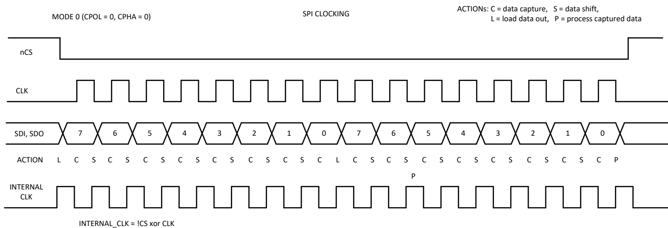
Figure 29. SPI Clocking
