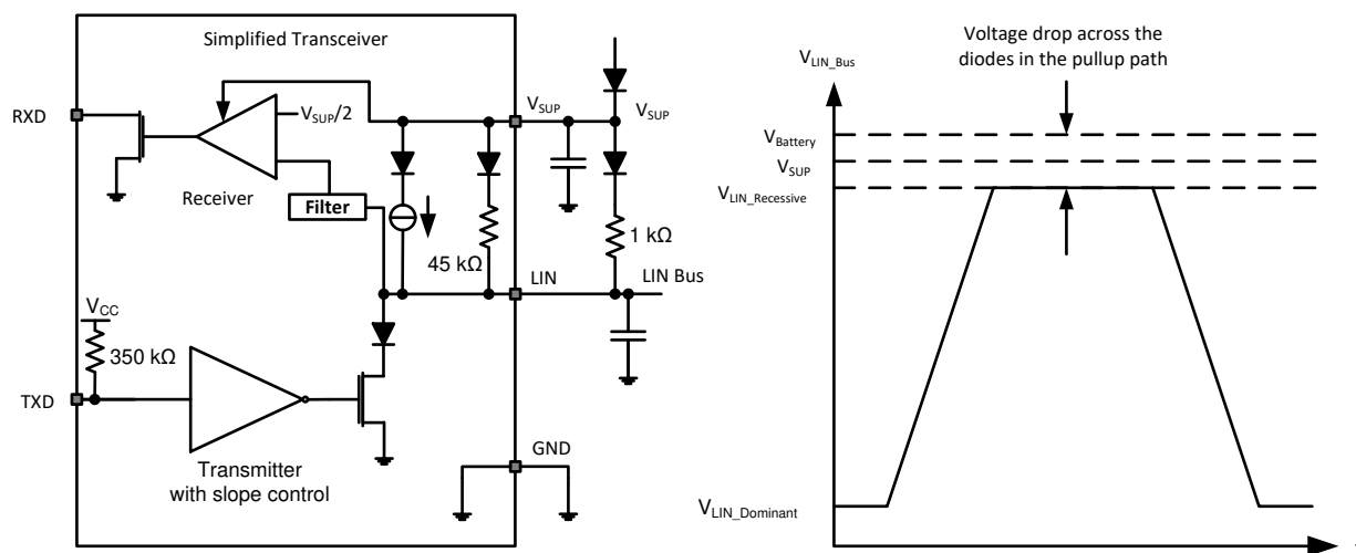
Figure 22. Master Node Configuration with Voltage Levels
