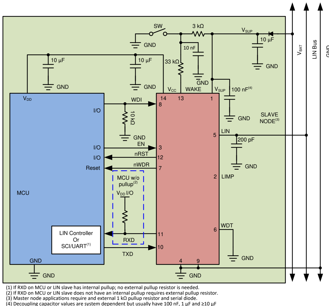
Figure 32. Typical LIN Slave in Pin Control Mode
