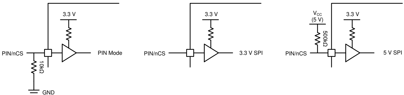
Figure 23. PIN/nCS Configuration
