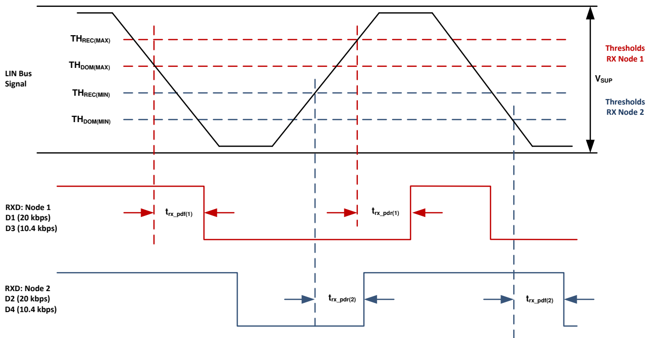
Figure 14. Propagation Delay
