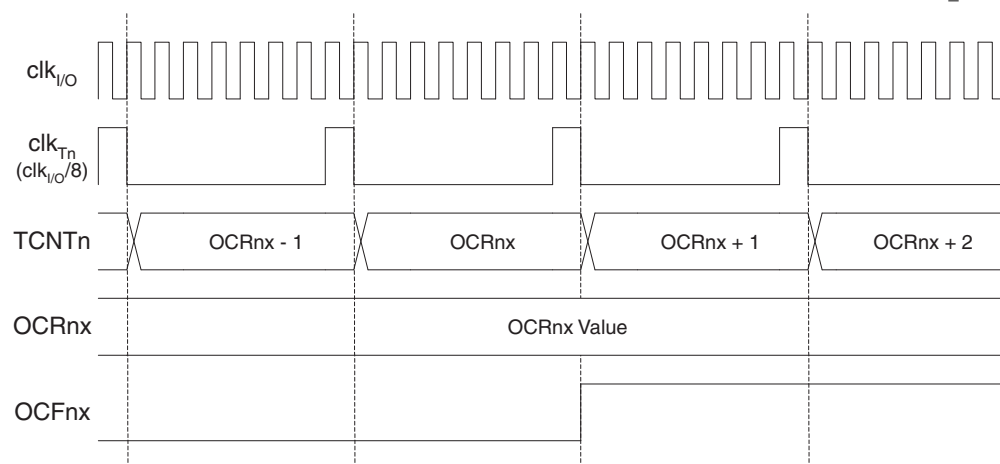
Figure 57. Timer/Counter Timing Diagram, Setting of OCF1x, with Prescaler ( f_{clk_{I/O}/8} )
