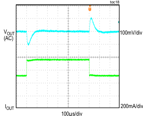
LOAD CURRENT STEPPED FROM 0.5A TO 0.75A (5V OUTPUT, PWM MODE, FIGURE 4 CIRCUIT)
