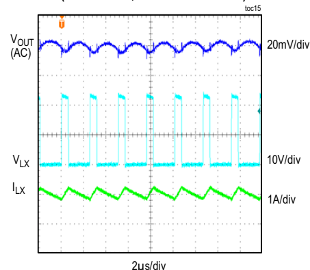
STEADY-STATE SWITCHING WAVEFORMS (5V OUTPUT, FIGURE 4 CIRCUIT)
