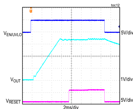
SOFT-START/SHUTDOWN FROM EN/UVLO, (3.3V OUTPUT, PFM MODE, 5mA LOAD CURRENT, FIGURE 5 CIRCUIT)
