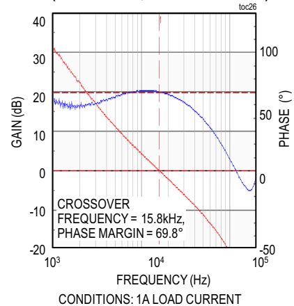
BODE PLOT (3.3V OUTPUT, FIGURE 5 CIRCUIT)
