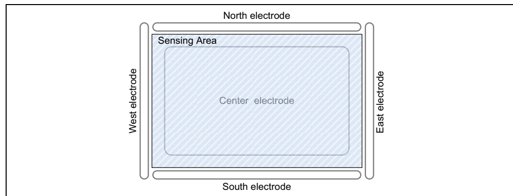
FIGURE 3-5: SENSING AREA
