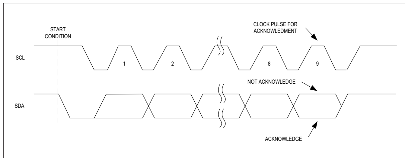
Figure 5. I 2 C Acknowledge Bit
