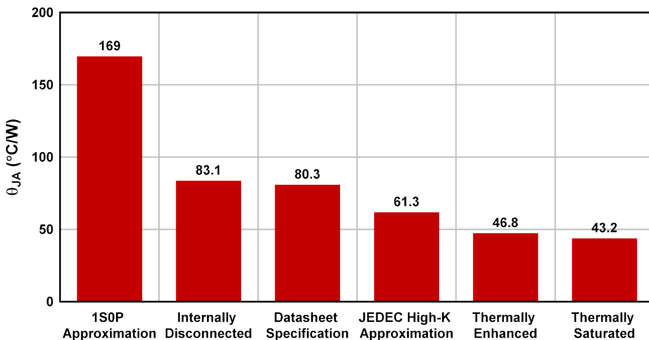
Figure 57. TPS746-Q1 (WSN) R_{\theta JA} vs Board Layout
