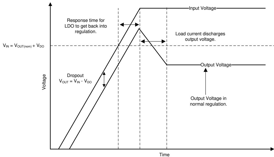
Figure 51. Startup Into Dropout
