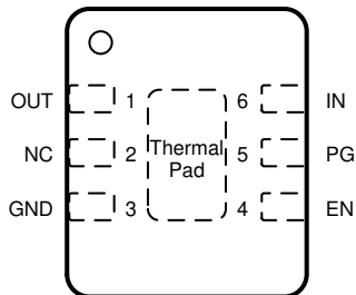
DRV Package 6-Pin Fixed WSON Top View
