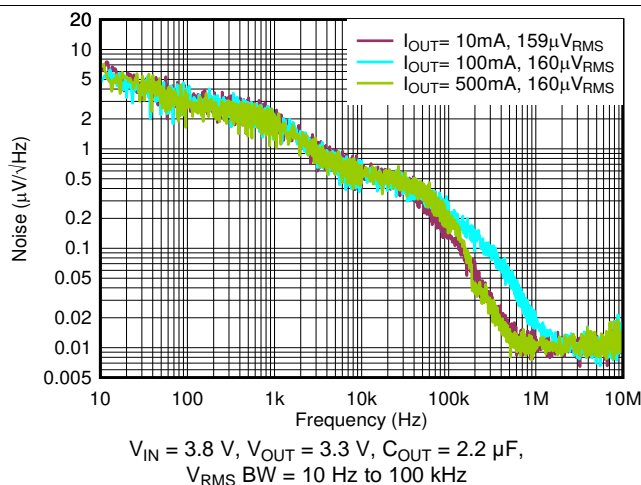
Figure 41. Output Spectral Noise Density vs Frequency and I_{OUT}
