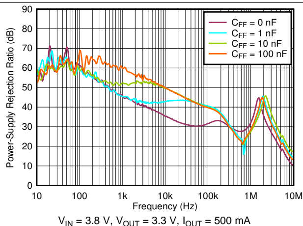
Figure 38. PSRR vs Frequency and C_{FF}
