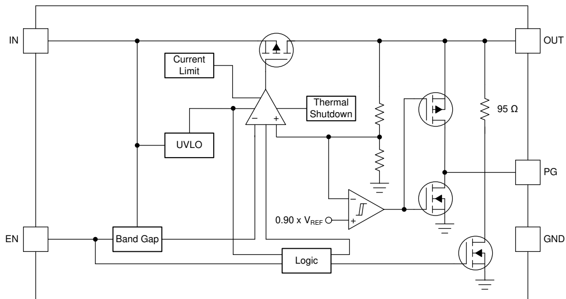
Figure 48. Fixed Voltage Version With Push-Pull Power-Good
