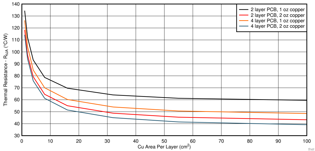
Figure 54. R_{\theta JA} versus Cu Area for the WSON (DRV) Package
