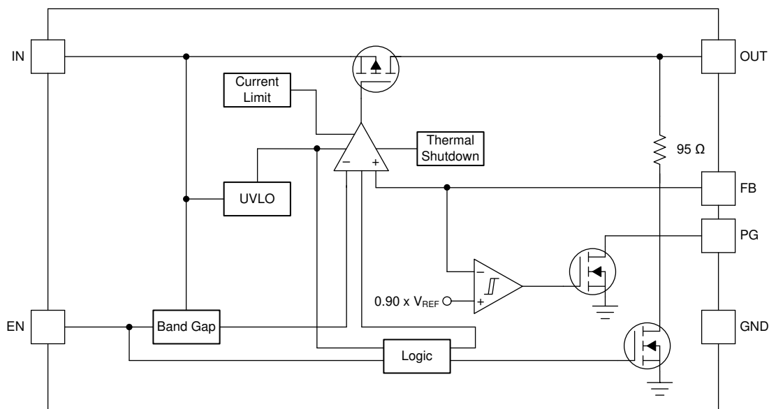
Figure 45. Adjustable Version With Open-Drain Power-Good
