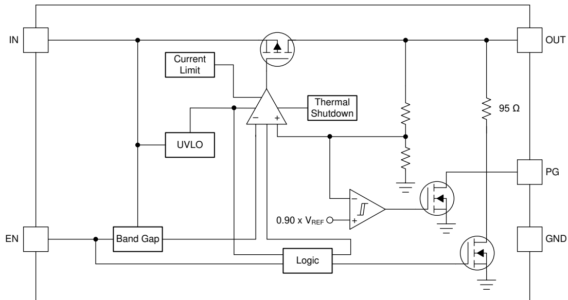
Figure 47. Fixed Voltage Version With Open-Drain Power-Good
