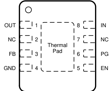
DRB Package (Preview) 8-Pin Adjustable WSON Top View
