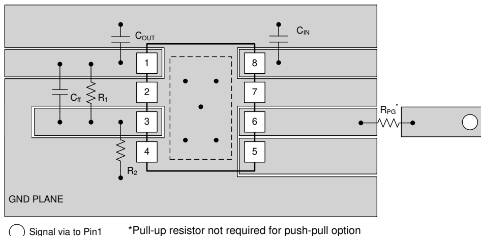
Figure 61. Layout Example for the DRB package
