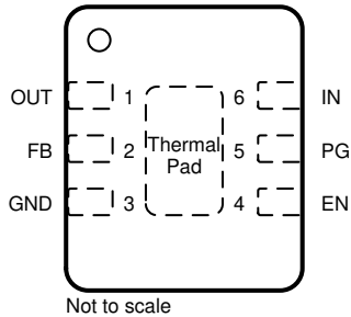
DRV Package 6-Pin Fixed WSON Top View
