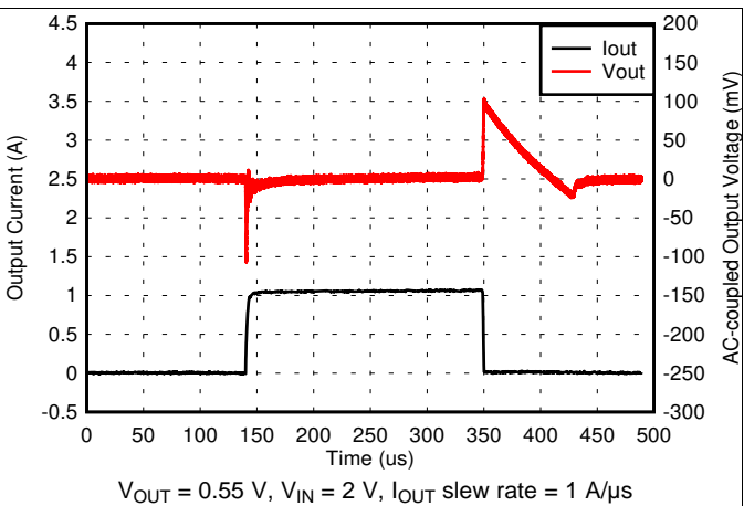
Figure 26. 1-mA to 1-A Load Transient (0.55 V)
