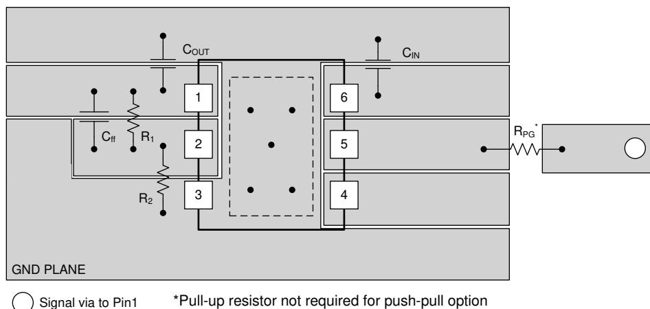
Figure 60. Layout Example for the DRV Package
