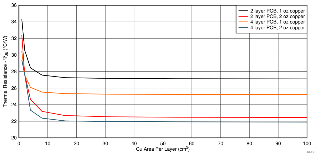
Figure 55. \psi_{JB} versus Cu Area for the WSON (DRV) Package
