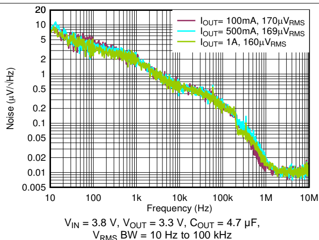
Figure 40. Output Spectral Noise Density vs Frequency and I_{OUT}
