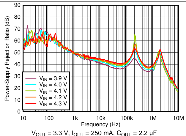
Figure 34. PSRR vs Frequency and V_{IN}
