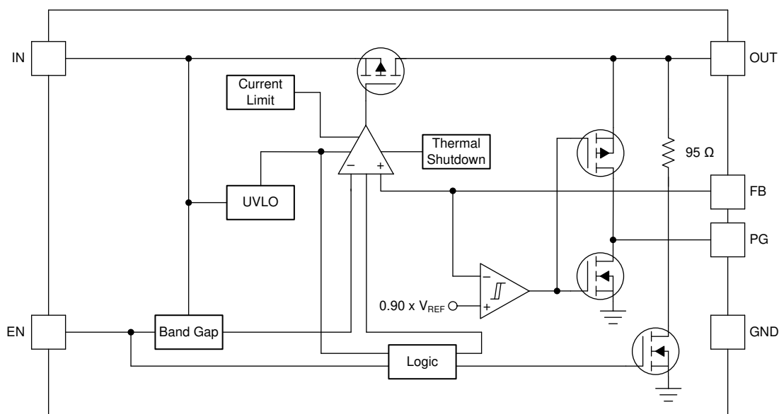
Figure 46. Adjustable Version With Push-Pull Power-Good
