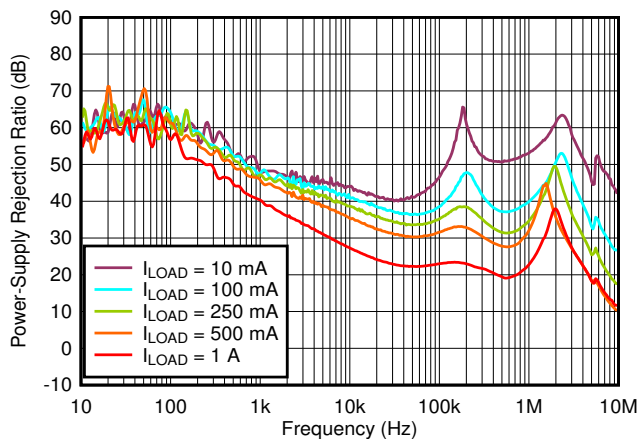
Figure 59. PSRR vs Frequency and I_{LOAD}
