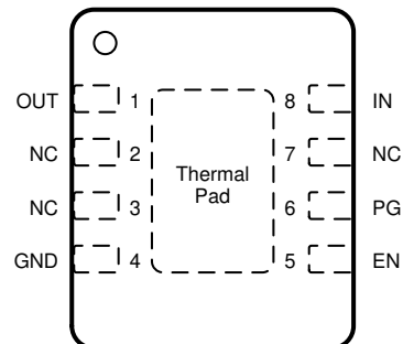
DRB Package (Preview) 8-Pin Fixed WSON Top View
