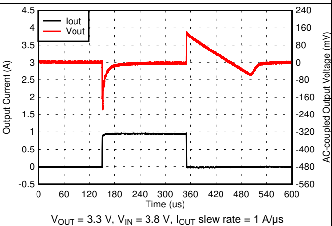
Figure 28. 1-mA to 1-A Load Transient (3.3 V)
