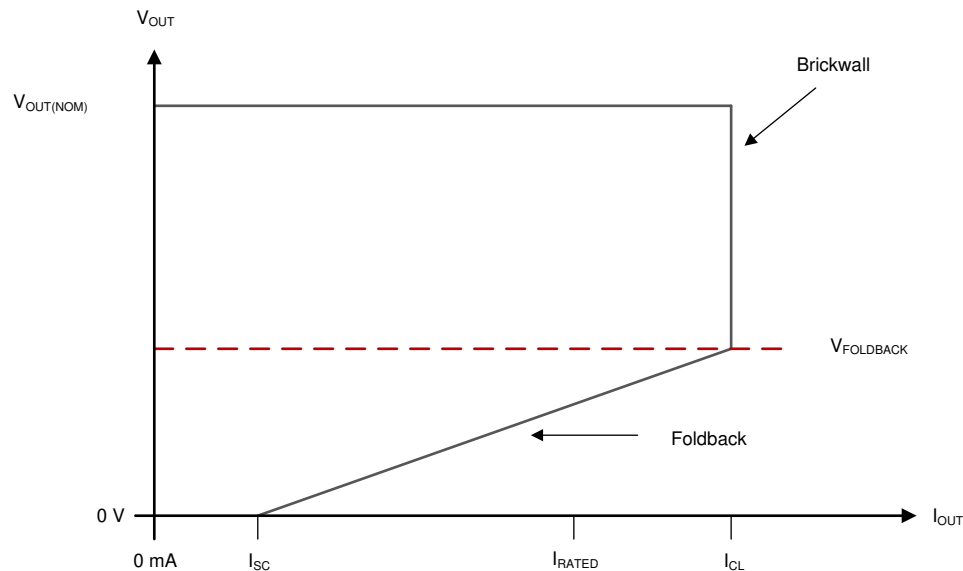
Figure 49. Foldback Current Limit
