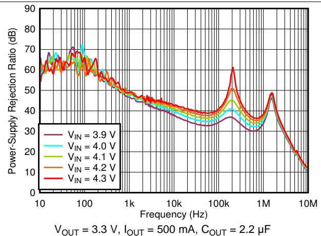
Figure 32. PSRR vs Frequency and V_{IN}
