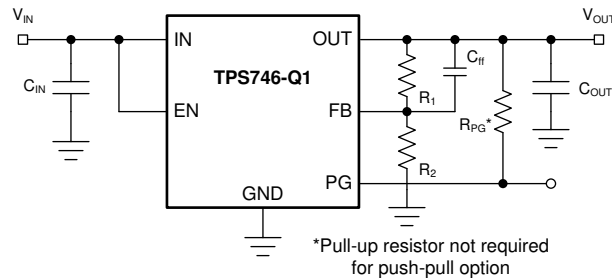
Figure 58. TPS746-Q1 Typical Application
