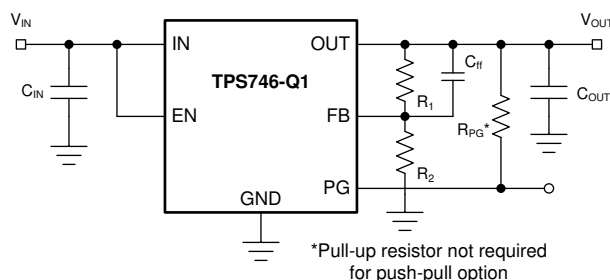
Figure 50. Adjustable Operation
