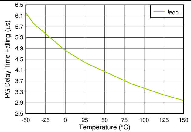
Figure 20. t_{PGDI} vs Temperature
