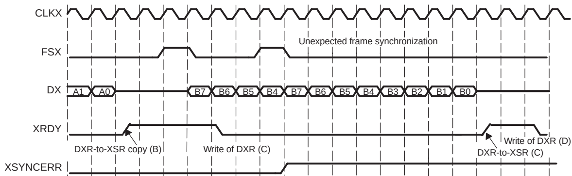
Figure 23-31. Unexpected Transmit Frame Synchronization Pulse
