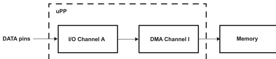
Figure 29-2. Data Flow for Single-Channel Receive Mode
