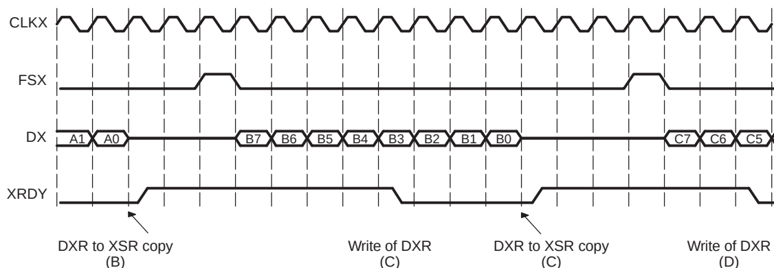
Figure 23-17. Transmit Operation
