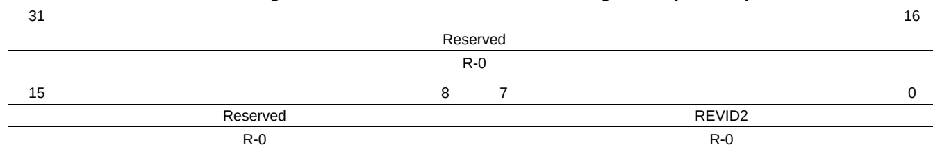
Figure 28-22. Revision Identification Register 2 (REVID2)
