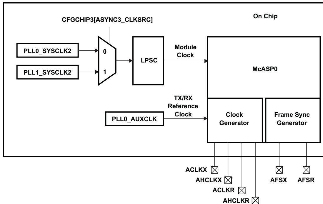
Figure 6-7. McASP Clocking Diagram
