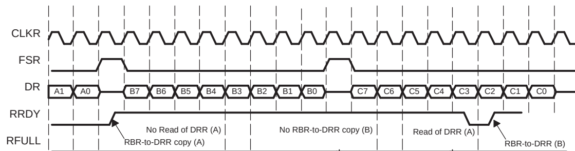
Figure 23-24. Serial Port Receive Overrun Avoided
