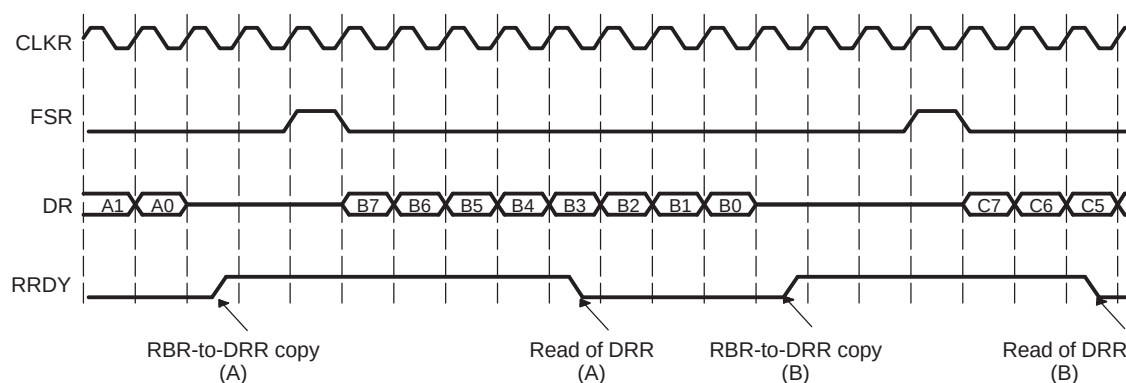
Figure 23-16. Receive Operation
