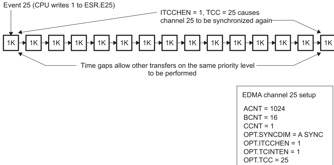
Figure 16-34. Smaller Packet Data Transfers Example
