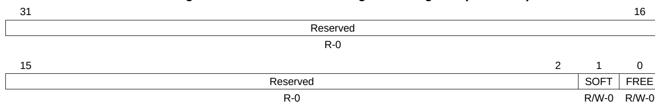
Figure 27-14. Emulation Management Register (EMUMGT)
