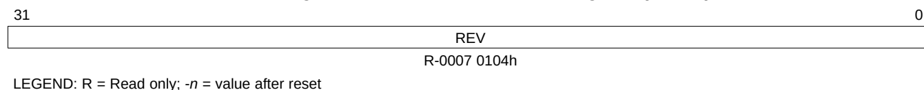
Figure 17-25. MDIO Revision ID Register (REVID)
