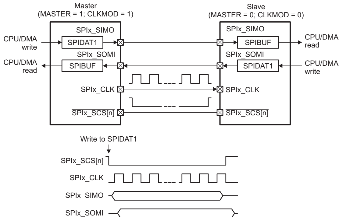
Figure 26-3. SPI 4-Pin Option with \overline{\text{SPIx\_SCS}}[n]
