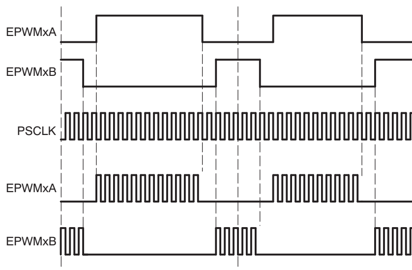
Figure 15-33. Simple PWM-Chopper Submodule Waveforms Showing Chopping Action Only
