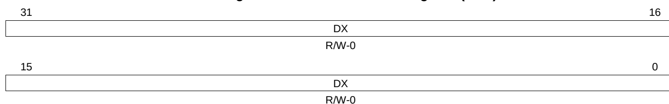
Figure 23-43. Data Transmit Register (DXR)
