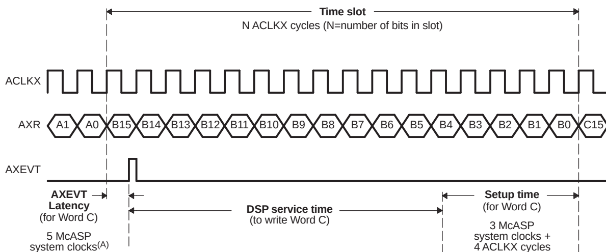
Figure 22-25. DSP Service Time Upon Transmit DMA Event (AXEVT)
