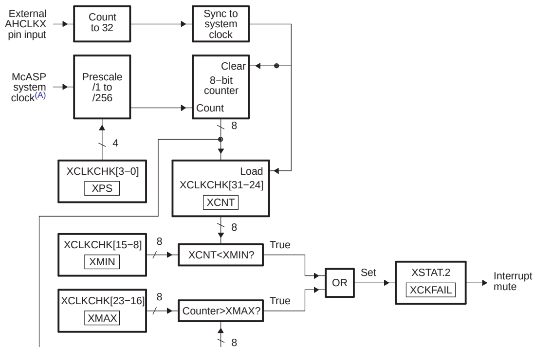
Figure 22-32. Transmit Clock Failure Detection Circuit Block Diagram
