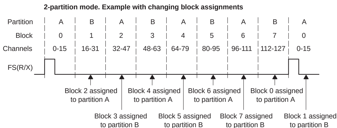
Figure 23-39. Reassigning Channel Blocks Throughout a McBSP Data Transfer
