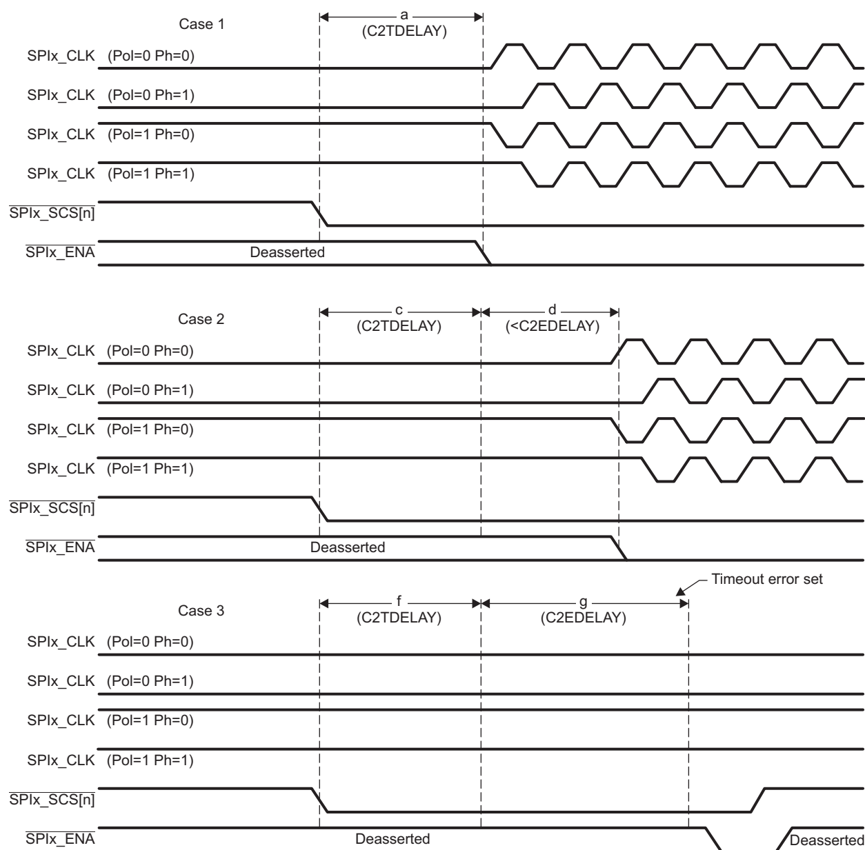
Figure 26-17. SPI 5-Pin Mode Demonstrating C2TDELAY and C2EDELAY
