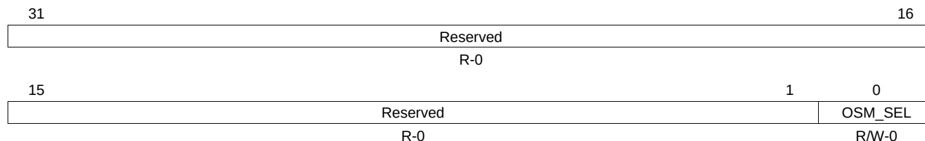
Figure 28-24. Mode Definition Register (MDR)
