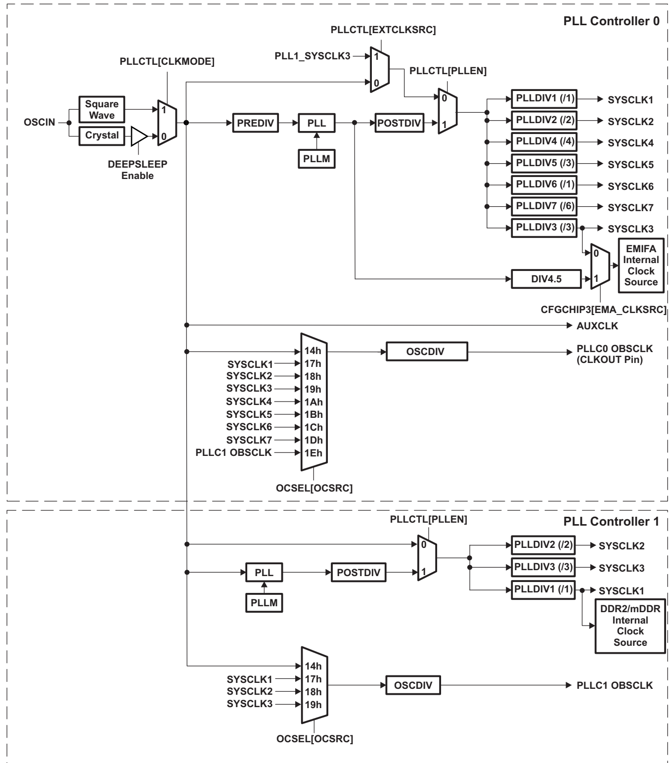
Figure 7-1. PLLC Structure
