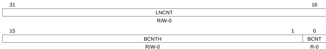
Figure 29-29. uPP DMA Channel I Descriptor 1 Register (UPID1)
