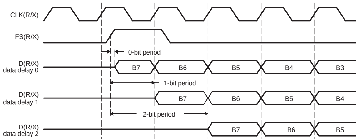
Figure 23-13. Data Delay
