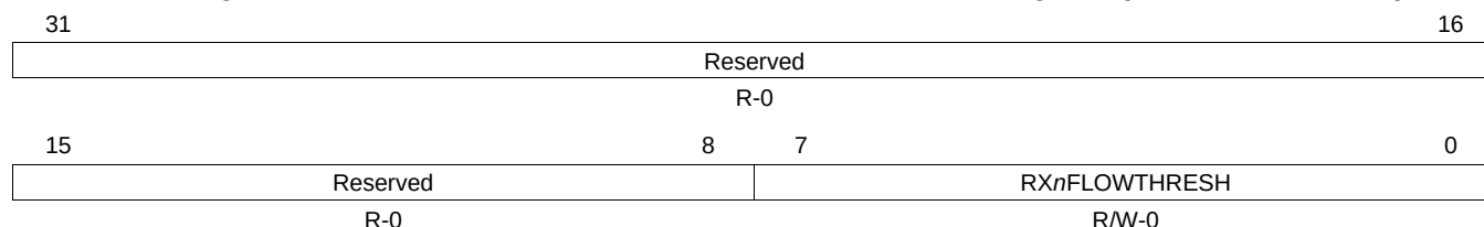
Figure 17-65. Receive Channel n Flow Control Threshold Register (RX n FLOWTHRESH)
