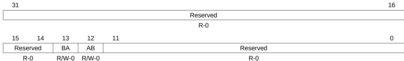
Figure 29-18. uPP Digital Loopback Register (UPDLB)
