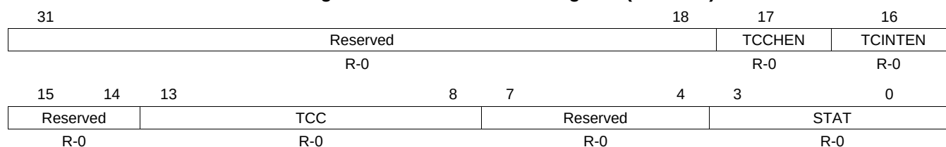
Figure 16-88. Error Details Register (ERRDET)
