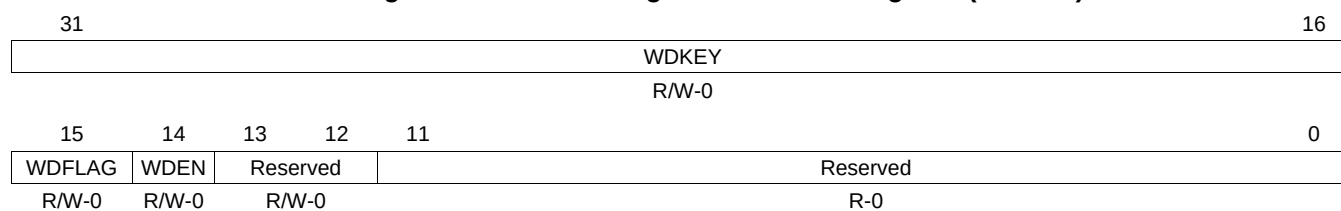
Figure 27-23. Watchdog Timer Control Register (WDTCR)
