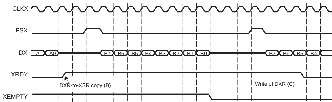
Figure 23-28. Transmit Empty
