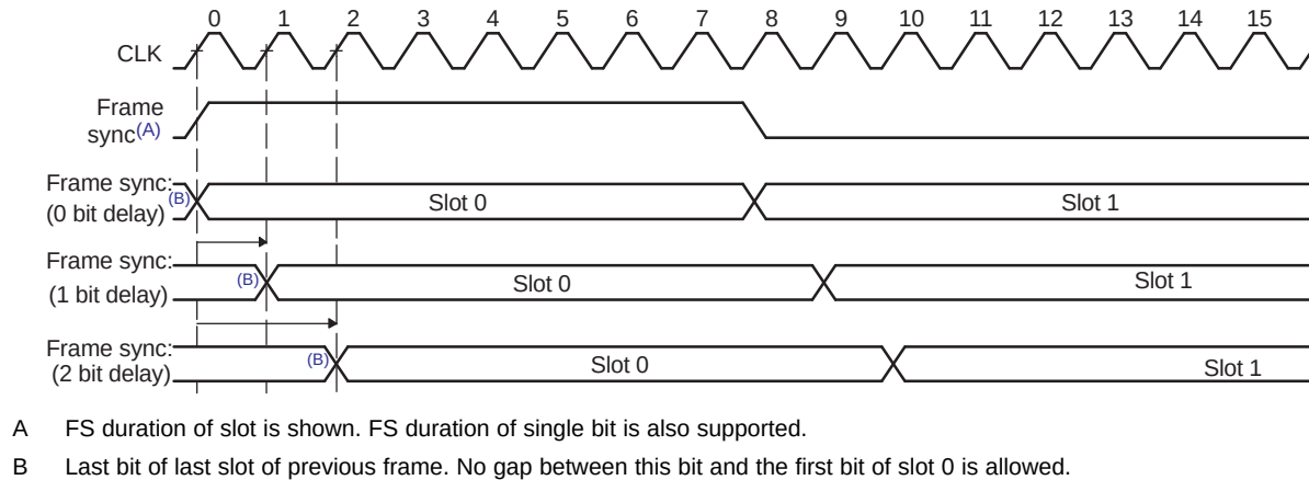
Figure 22-7. TDM Format Bit Delays from Frame Sync
