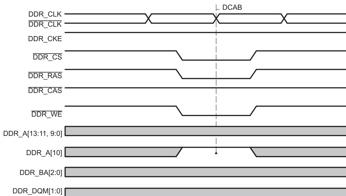
Figure 13-5. DCAB Command
