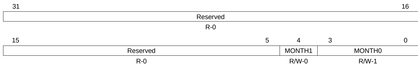
Figure 25-8. Month Register (MONTH)
