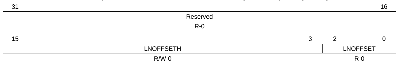
Figure 29-30. uPP DMA Channel I Descriptor 2 Register (UPID2)
