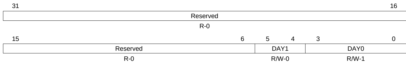
Figure 25-7. Days Register (DAY)
