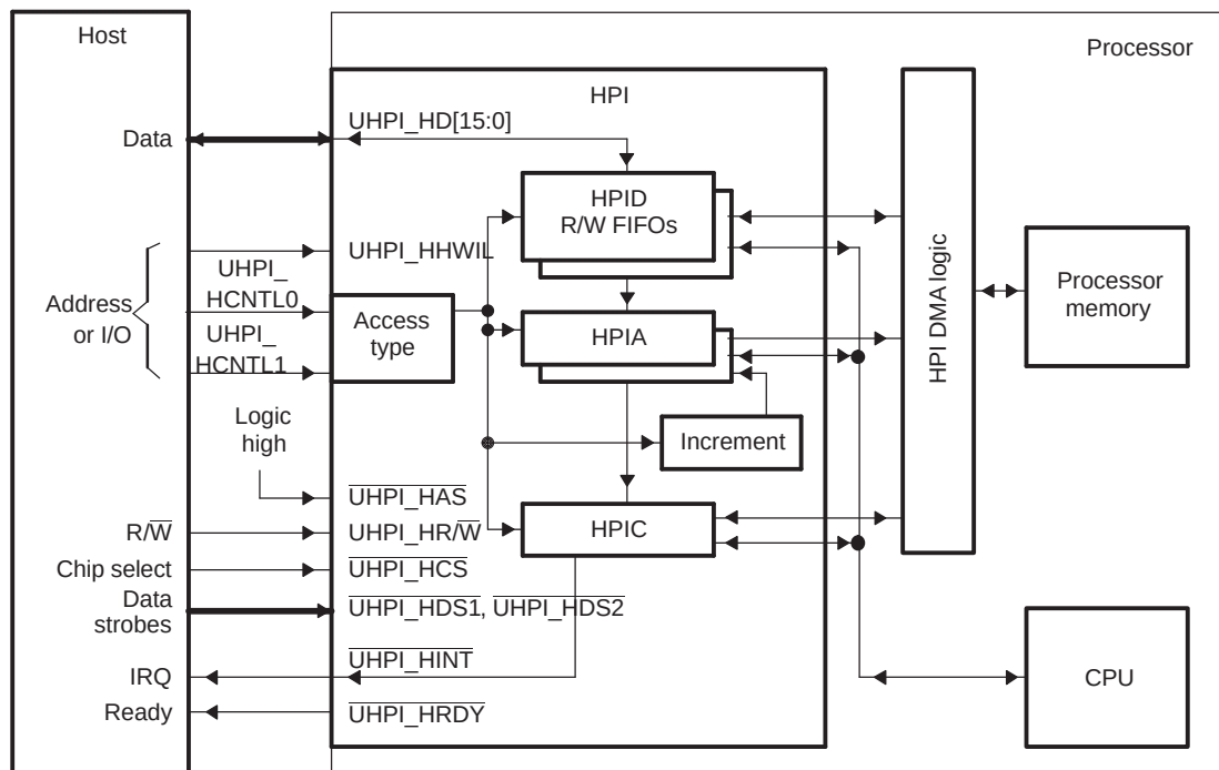
Figure 20-1. HPI Block Diagram
