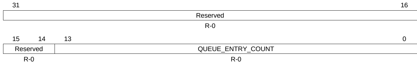
Figure 30-115. Queue Manager Queue N Status Register A (QSTATA[N])
