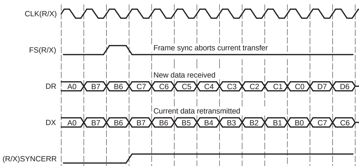
Figure 23-19. Unexpected Frame Synchronization With (R/X)FIG = 0
