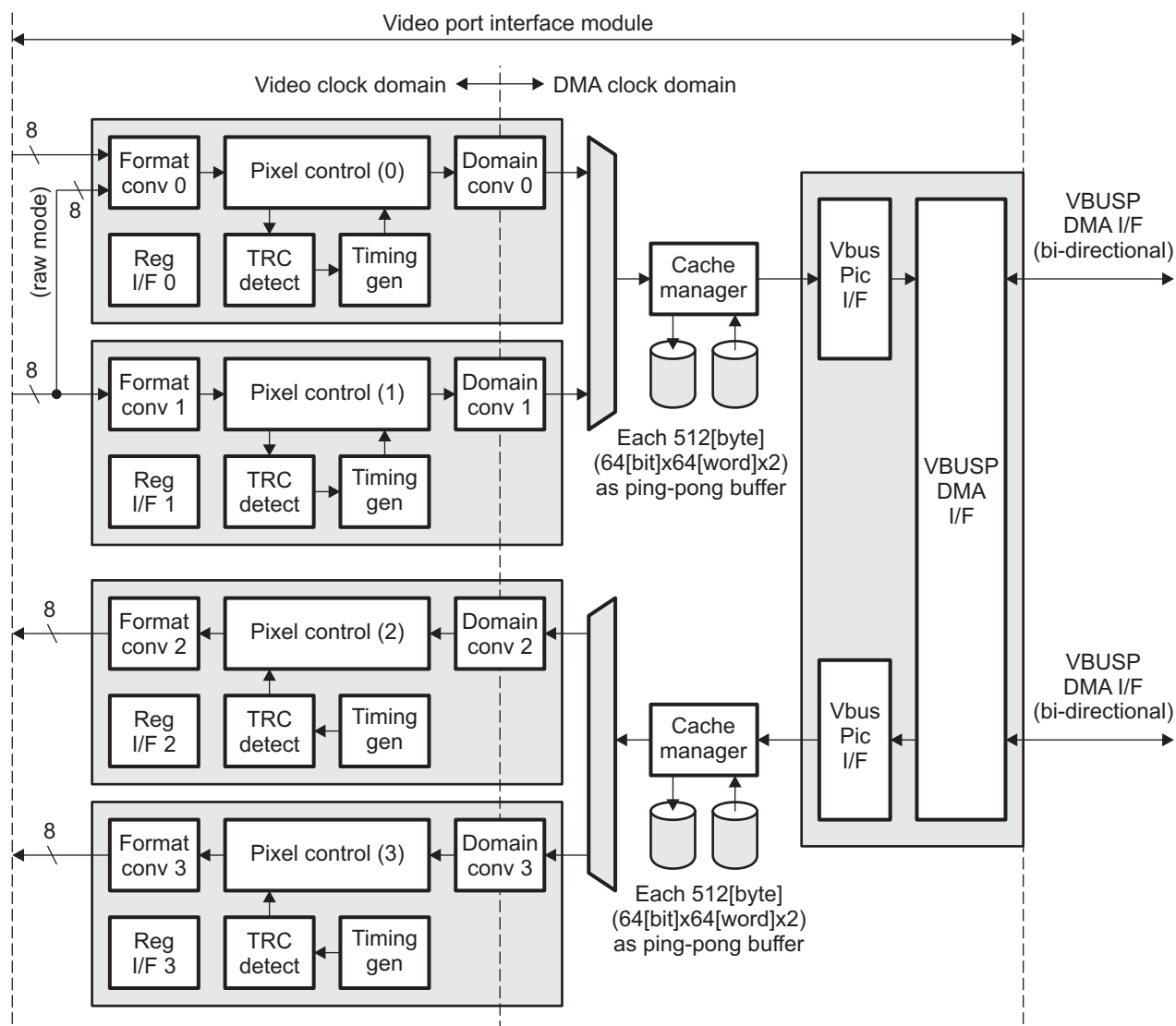
Figure 31-3. VPIF Architecture Block Diagram
