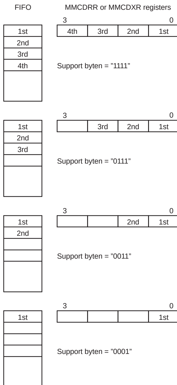
Figure 24-8. Little-Endian Access to MMCDXR/MMCDRR from the CPU or the EDMA
