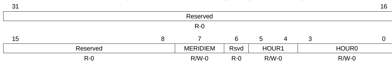
Figure 25-13. Alarm Hour Register (ALARMHOUR)
