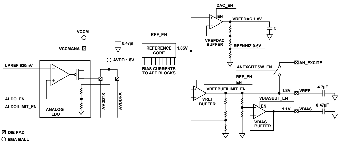
Figure 132. AFE Power-Up
