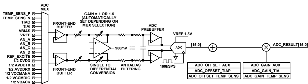
Figure 133. Auxiliary Channel Calibration
