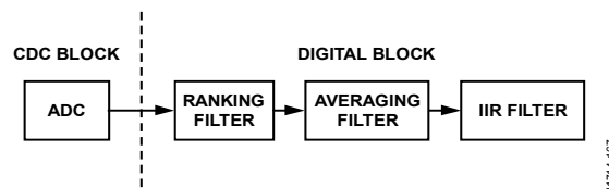
Figure 167. Digital Block
