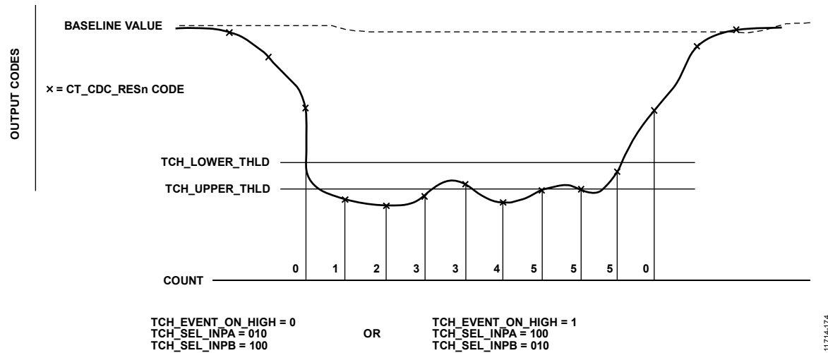
Figure 174. Touch Detection Example
