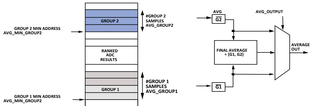
Figure 169. Averaging Filter
