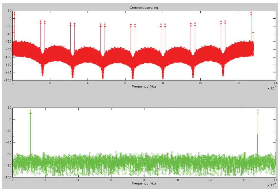
Figure 111. Coherent Sampling
