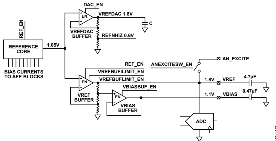
Figure 147. Signal Acquisition Reference Circuit
