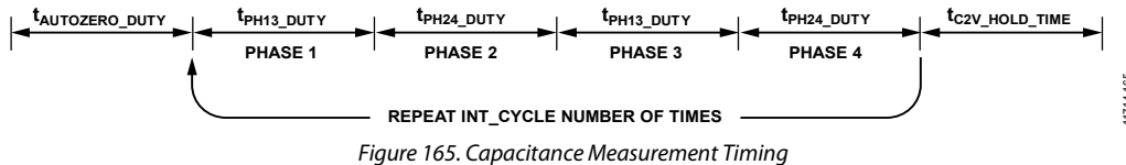
Figure 165. Capacitance Measurement Timing
