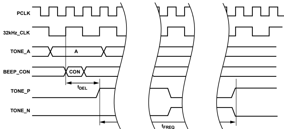
Figure 80. Timing Diagram
