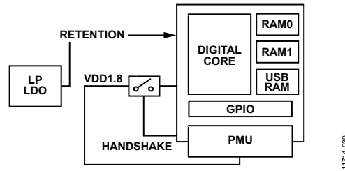
Figure 31. Power Switch
