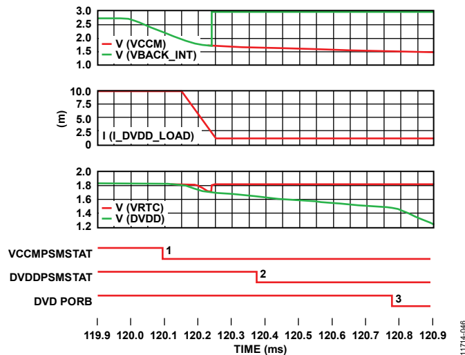
Figure 47. Removing Battery with a 2 \mu F Capacitor in Active Mode
