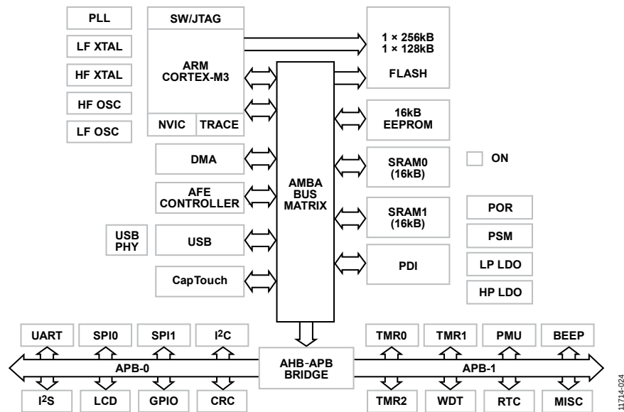
Figure 25. Active Mode
