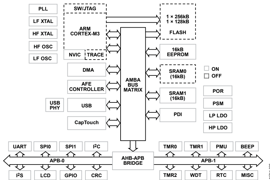
Figure 27. CORE_SLEEP Mode
