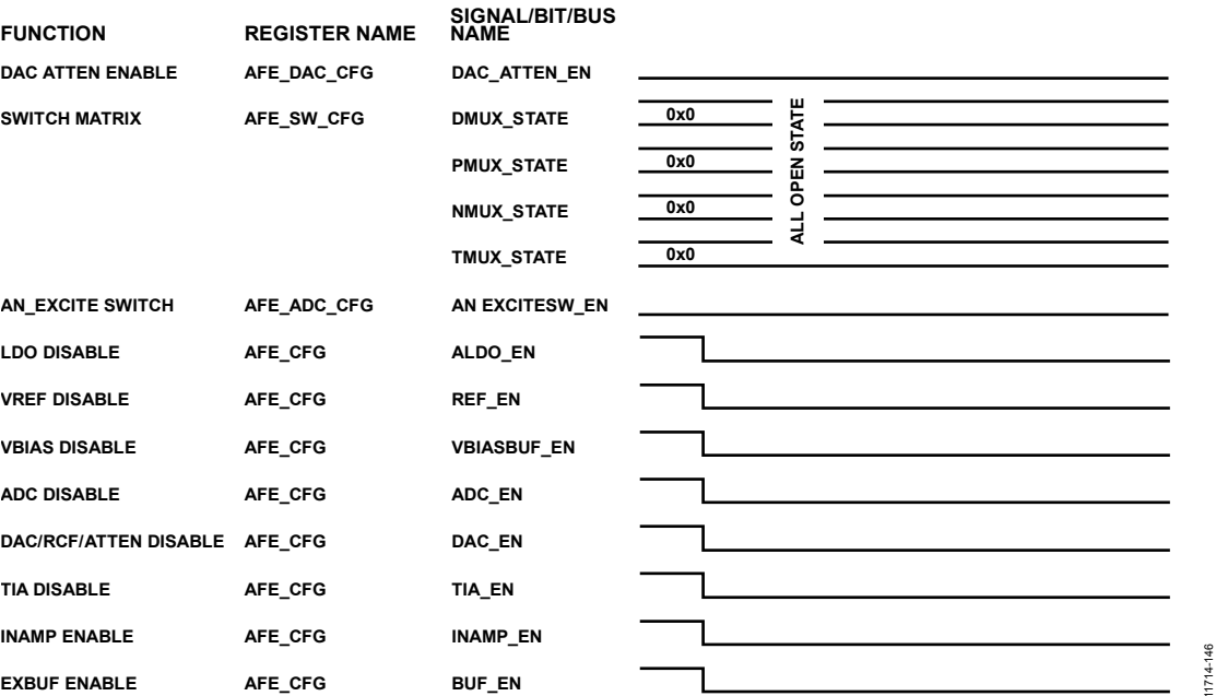
Figure 146. AFE Power-Down
