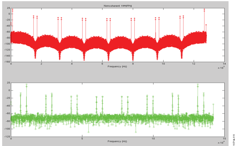
Figure 112. Noncoherent Sampling
