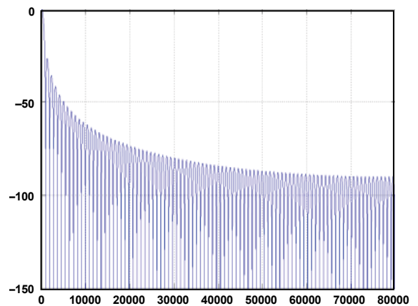
Figure 114. Sinc2hf Frequency Response
