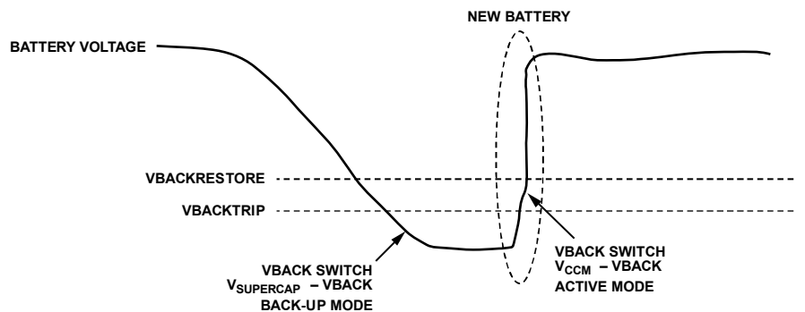
Figure 40. VBACK Switch Threshold Levels ( V_{\text{SUPERCAP}} is the voltage into the VBACK pin.)
