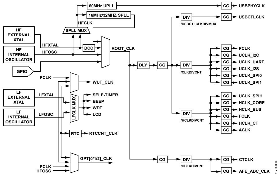
Figure 4. Clocking Diagram
