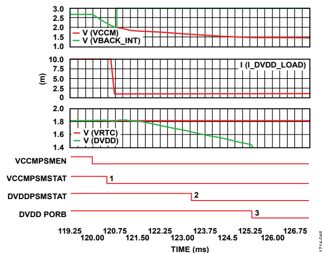
Figure 46. Removing Battery with a 10 \mu F Capacitor in Active Mode (DVDD PORB = Power-On Reset Block)
