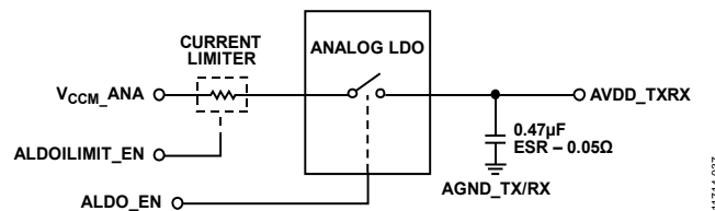
Figure 38. LDO Block Diagram
