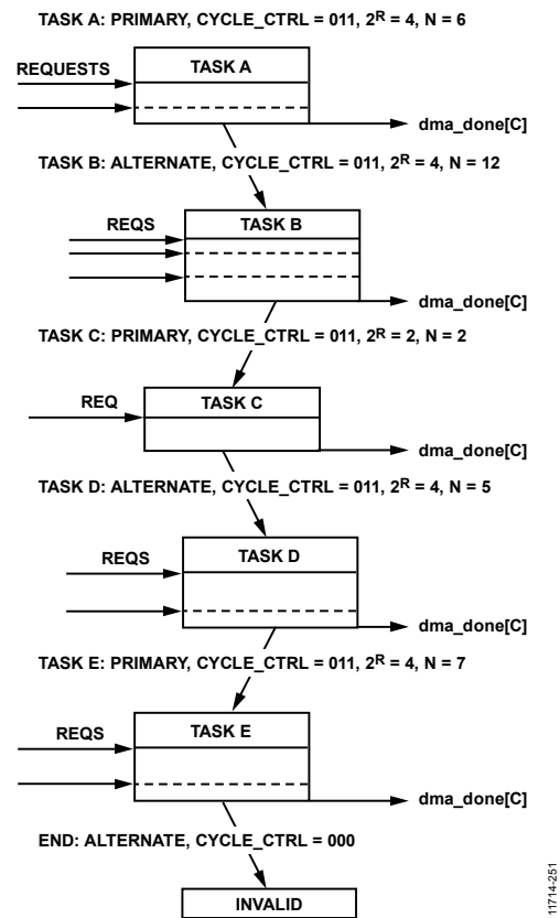
Figure 52. Peripheral Ping-Pong DMA Transfer Process
