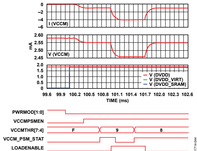
Figure 45. Hibernate to Active Mode
