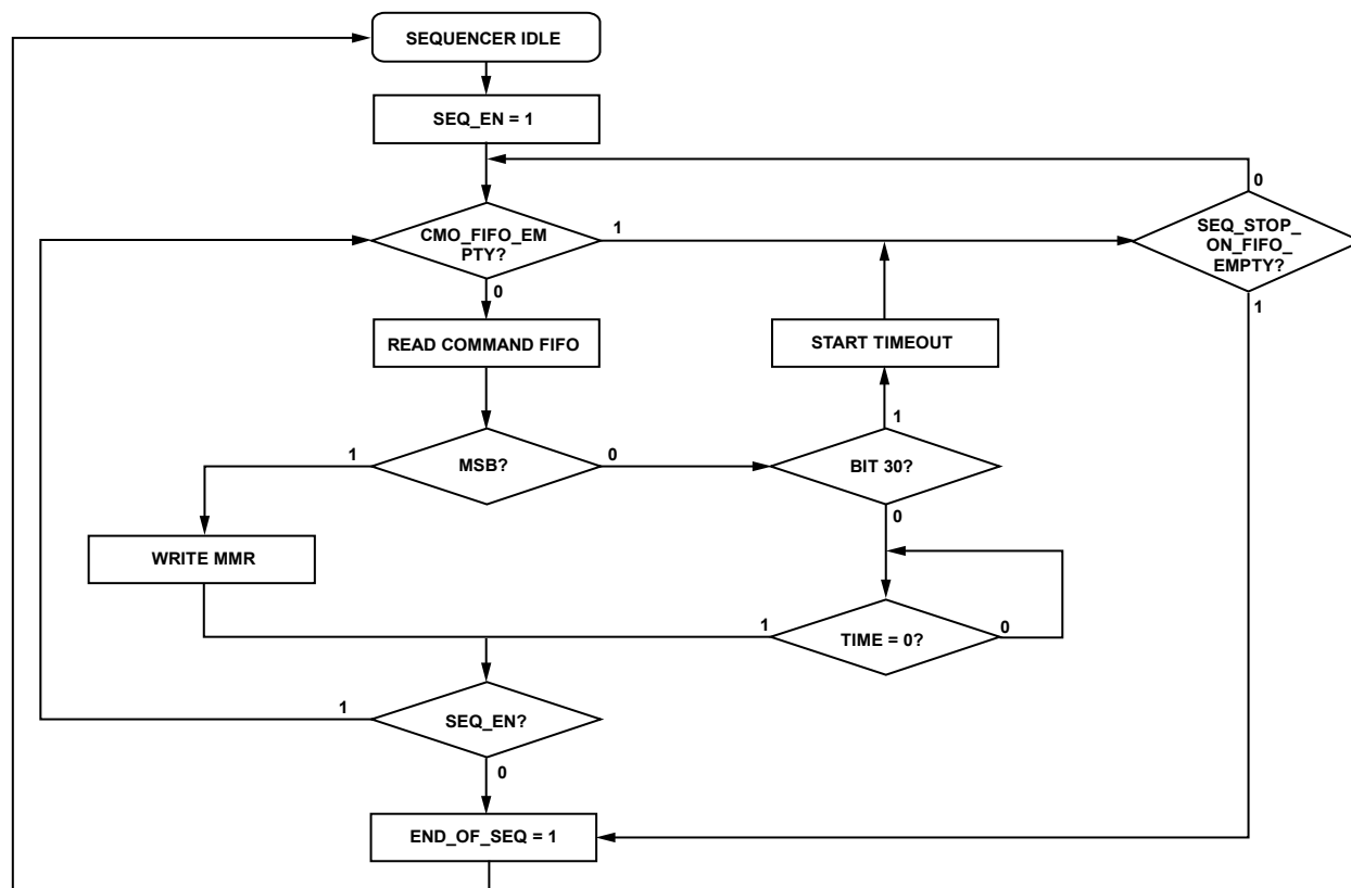
Figure 97. Sequencer Flow Diagram
