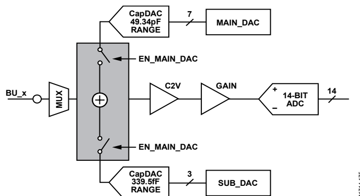
Figure 175. Applying the CapDACs
