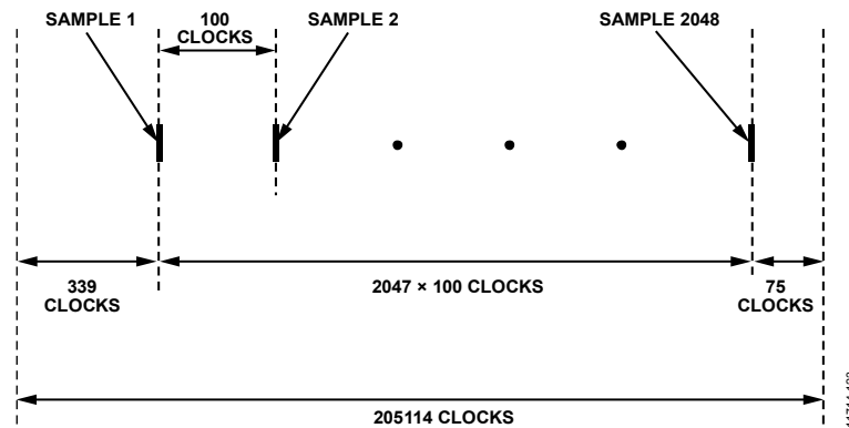
Figure 124. DFT Timing
