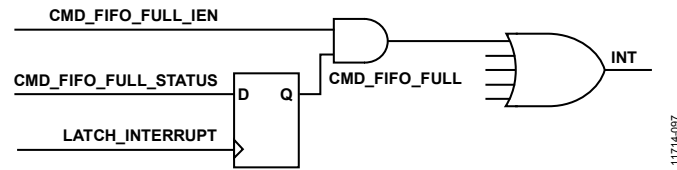
Figure 98. Interrupt Generation (LATCH_INTERRUPT is an Internal Signal)
