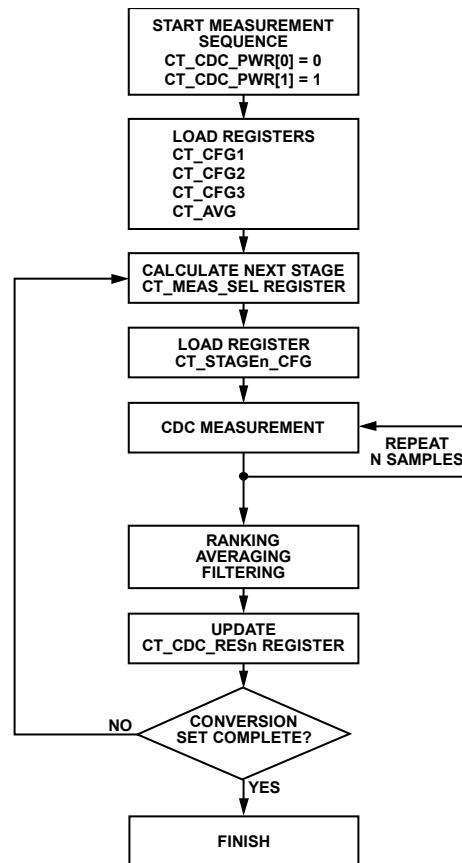
Figure 171. CapTouch Sequencer
