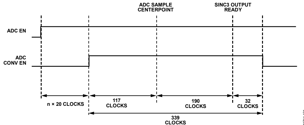
Figure 122. ADC Enable Timing
