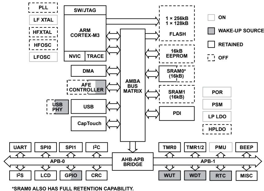
Figure 30. Hibernate Mode
