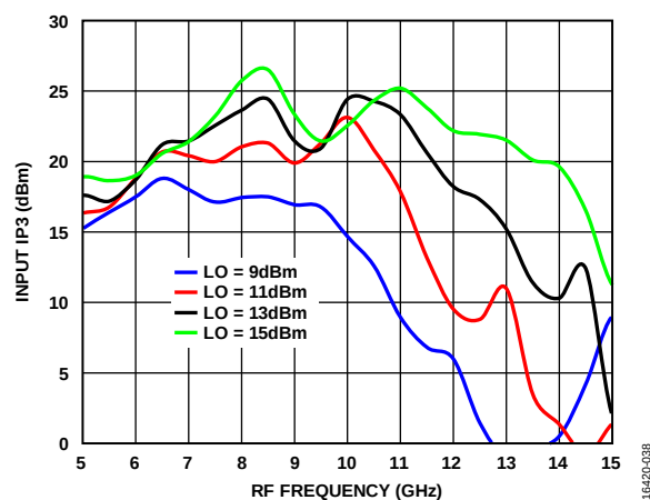
Figure 36. Input IP3 vs. RF Frequency at Various LO Power Levels, T_A = 25^\circ\text{C}
