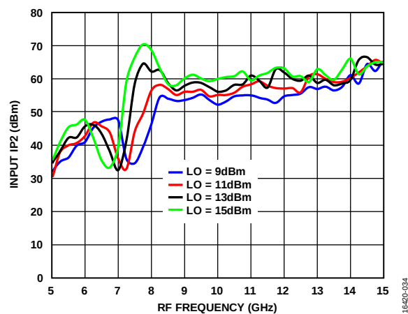
Figure 32. Input IP2 vs. RF Frequency at Various LO Power Levels, T_A = 25^\circ\text{C}
